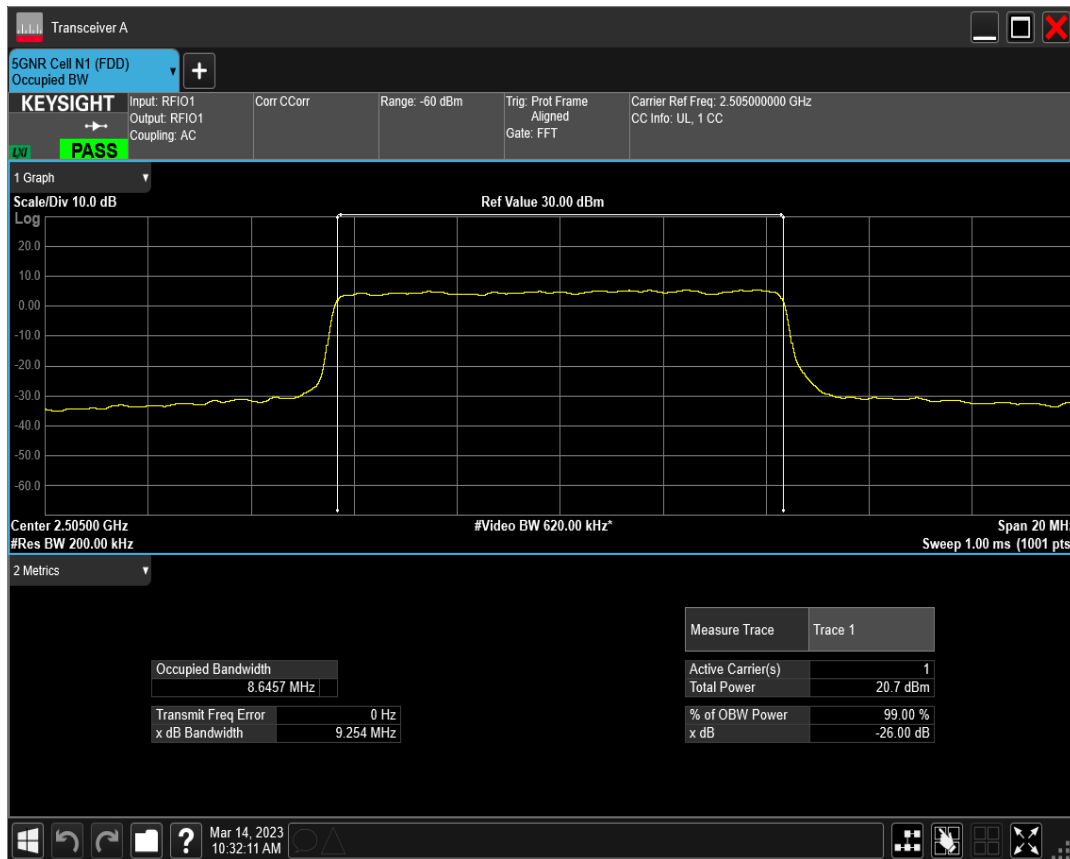
n7 SCS=30kHz DFT_QAM256 BW=10MHz Channel=501000 RB=24@0
