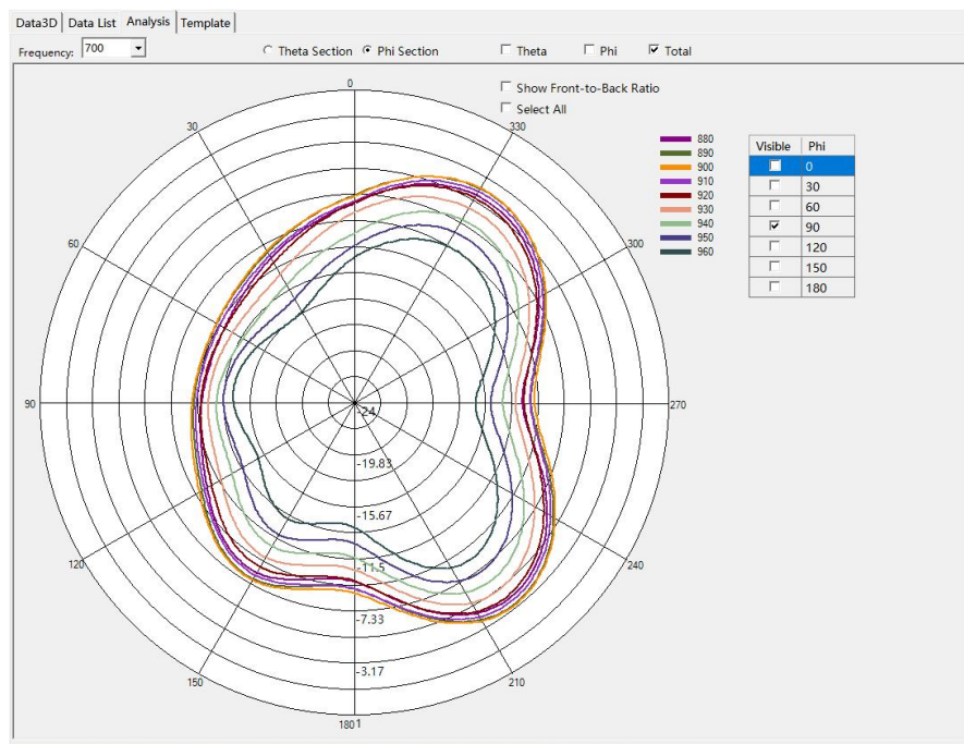
GSM900 / WCDMA B8 / LTE B8 Phi=90deg
