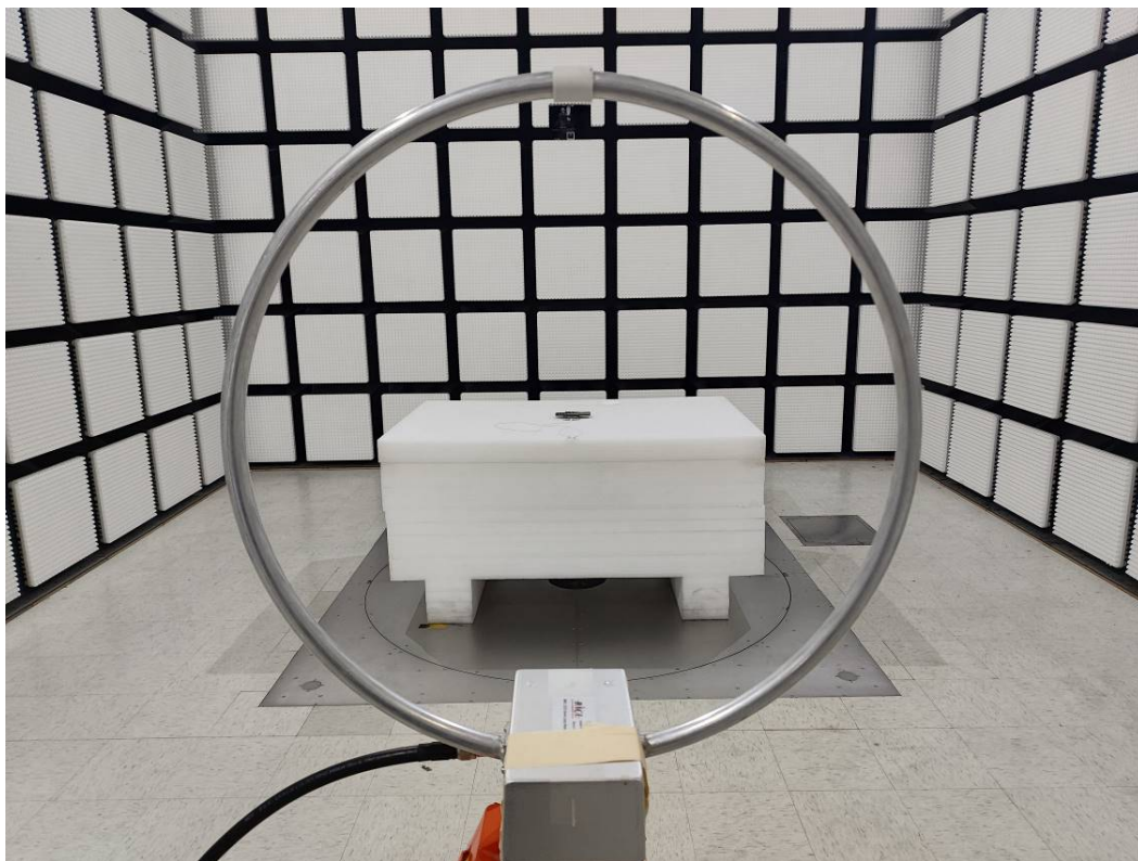
Radiated Emission 9kHz-30MHz parallel View- Normal Version
