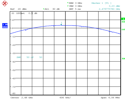
2DH1_High 3.23dBm
