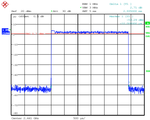
3DH5_Hopping 2.935ms
