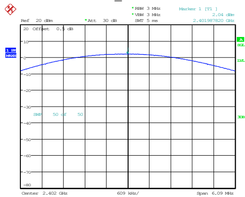
3DH1_Low 2.04dBm
