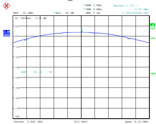
3DH1_Middle 3.81dBm
