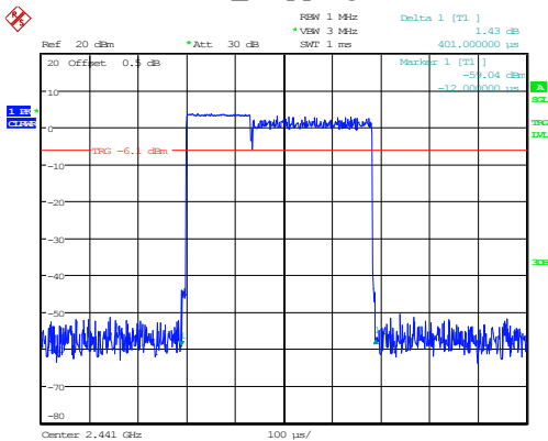
3DH1_Hopping 0.401ms
