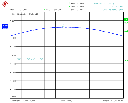
2DH1_Low 2.21dBm
