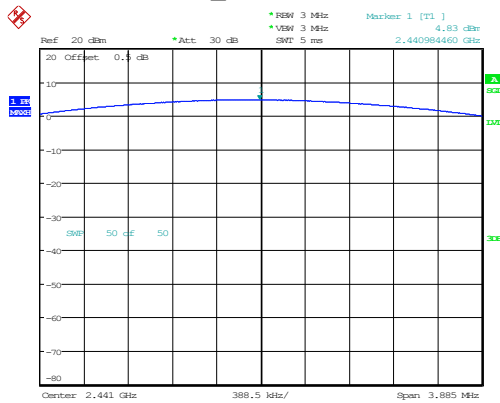
DH1_Middle 4.83dBm
