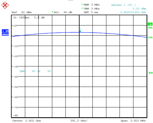
DH1_Low 3.03dBm
