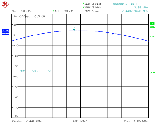
2DH1_Middle 3.98dBm
