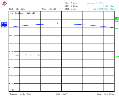
DH1_High 4.10dBm
