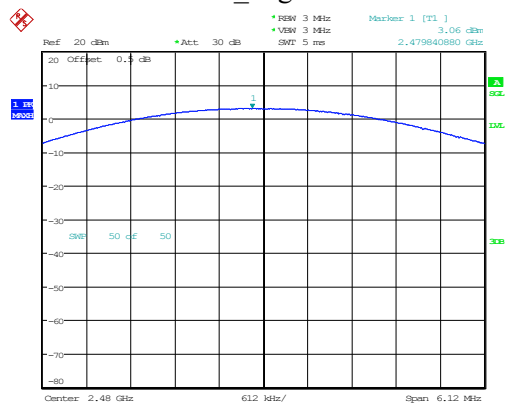
3DH1_High 3.06dBm
