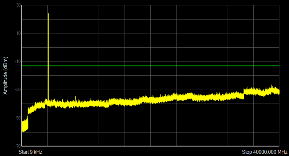
n77 SCS=30kHz CP_QPSK BW=10MHz Channel=679666 RB=1@23
