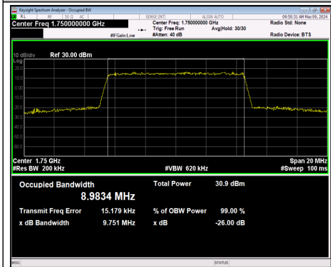
Band4-10MHz-16QAM-20350-50RB#0-PASS
