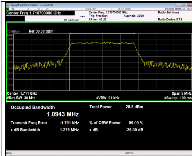
Band4-1.4MHz-64QAM-19957-6RB#0-PASS
