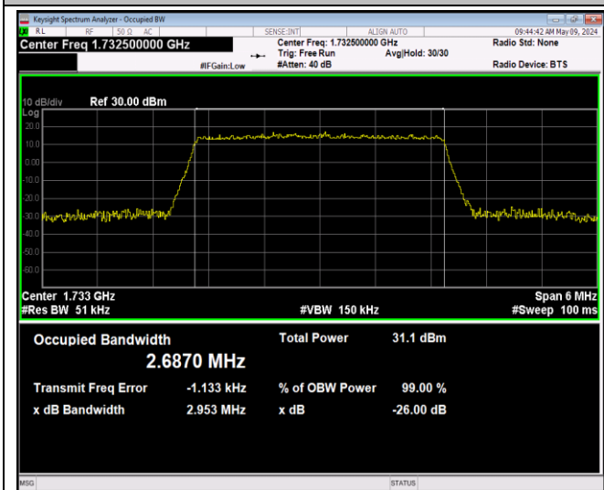
Band4-3MHz-QPSK-20175-15RB#0-PASS
