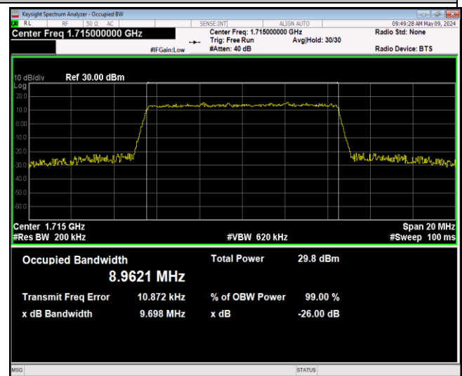
Band4-10MHz-64QAM-20000-50RB#0-PASS
