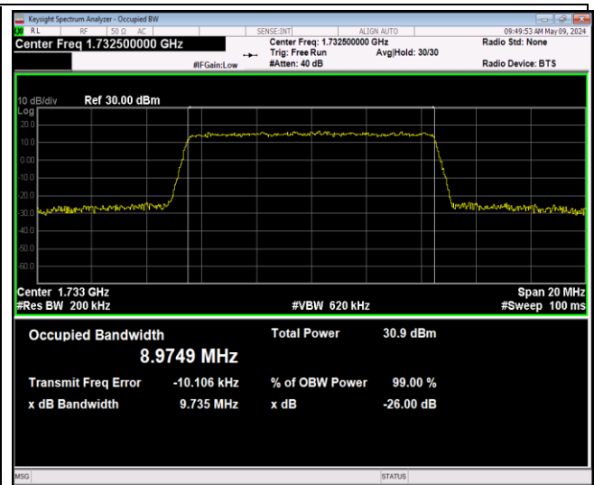
Band4-10MHz-16QAM-20175-50RB#0-PASS
