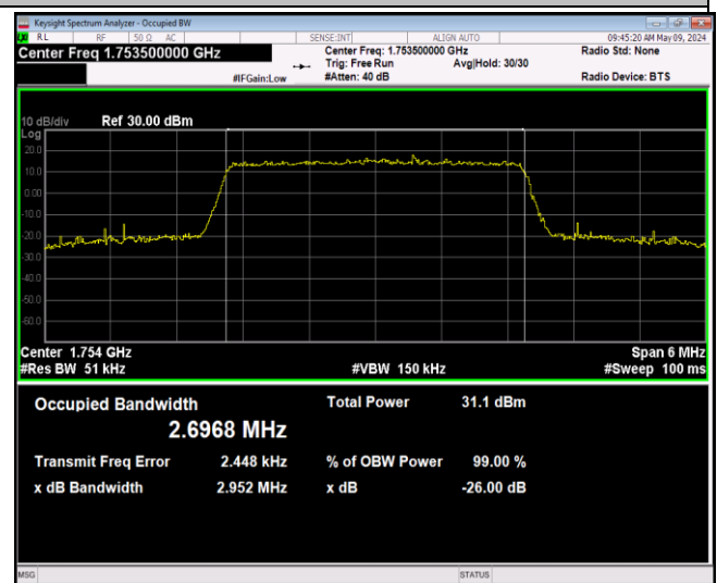
Band4-3MHz-QPSK-20385-15RB#0-PASS
