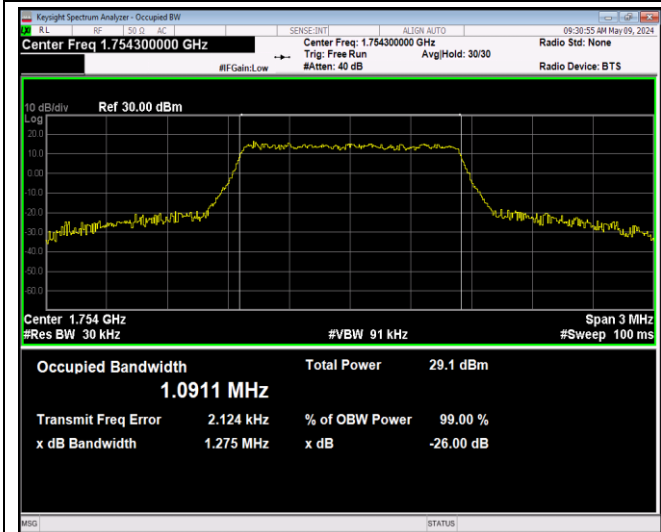
Band4-1.4MHz-64QAM-20393-6RB#0-PASS
