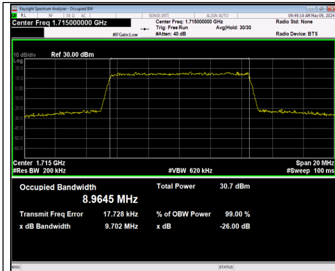
Band4-10MHz-16QAM-20000-50RB#0-PASS
