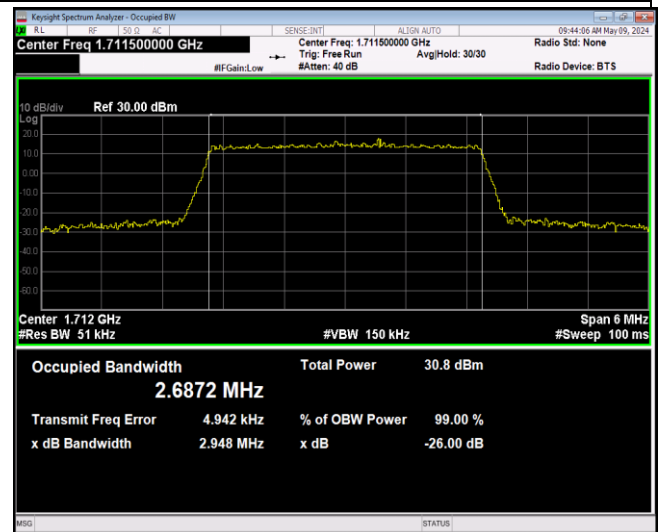
Band4-3MHz-QPSK-19965-15RB#0-PASS
