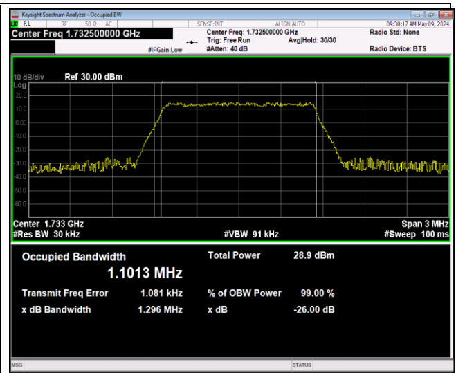
Band4-1.4MHz-64QAM-20175-6RB#0-PASS
