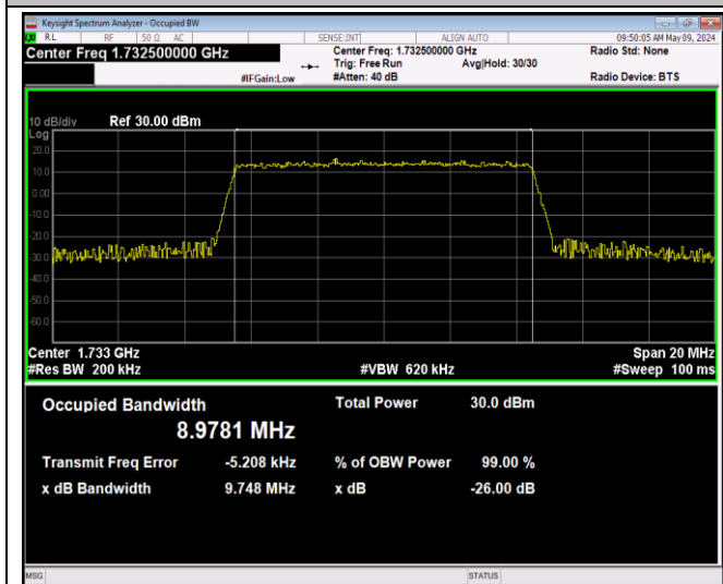
Band4-10MHz-64QAM-20175-50RB#0-PASS
