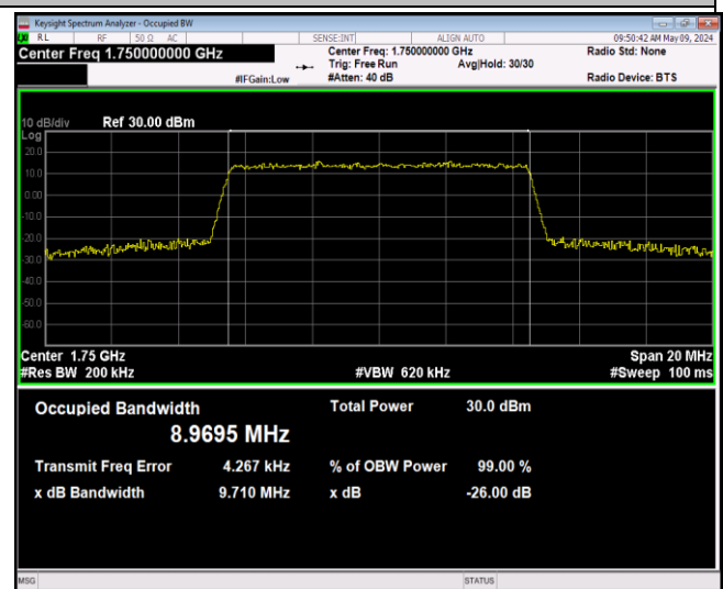
Band4-10MHz-64QAM-20350-50RB#0-PASS
