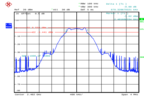
Low 0.679MHz
