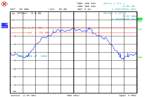
Middle 1.251MHz
