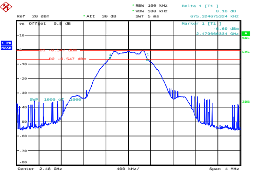
High 0.675MHz
