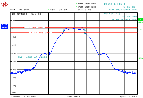
Middle 0.679MHz
