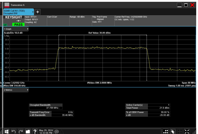
40MHz_30kHz_3625MHz_CP-OFDM 16QAM_RB106@0
