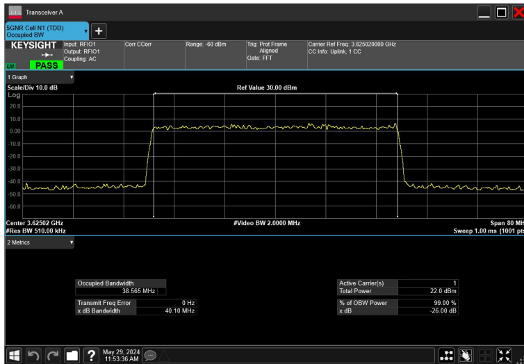
40MHz_15kHz_3625MHz_DFT-s-OFDM 64QAM_RB216@0
