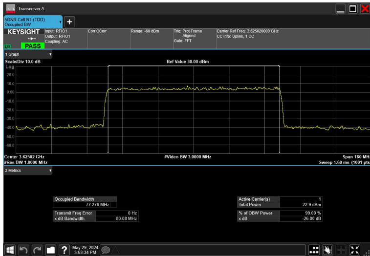
80MHz_30kHz_3625MHz_CP-OFDM16QAM_RB217@0
