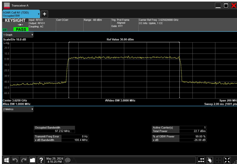
100MHz_30kHz_3625MHz_CP-OFDM16QAM_RB273@0
