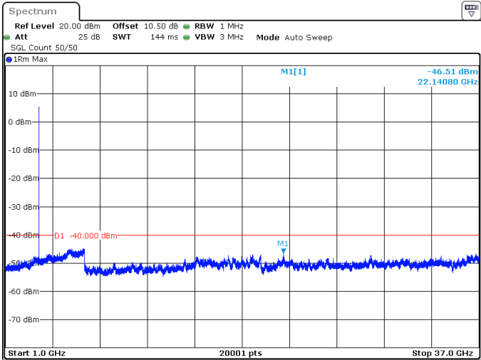
10MHz_15kHz_3555MHz_DFT-s-OFDM QPSK_RB1@51 -46.51 dBm
