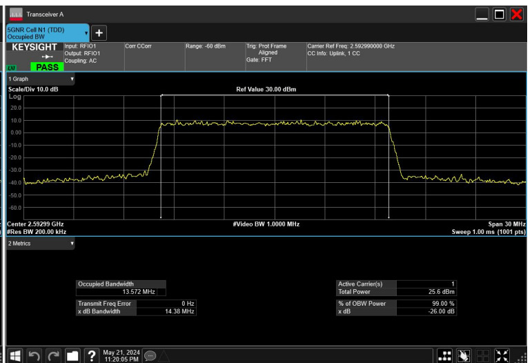
15MHz_30kHz_2592.99MHz_CP-OFDM 16 QAM_RB38@0
