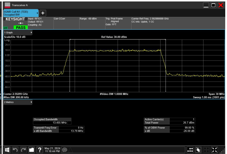
15MHz_30kHz_2592.99MHz_DFT-s-OFDM 16 QAM_RB36@0
