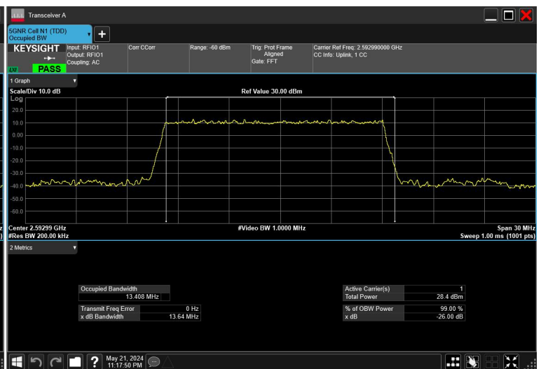
15MHz_30kHz_2592.99MHz_DFT-s-OFDM \pi/2 BPSK_RB36@0
