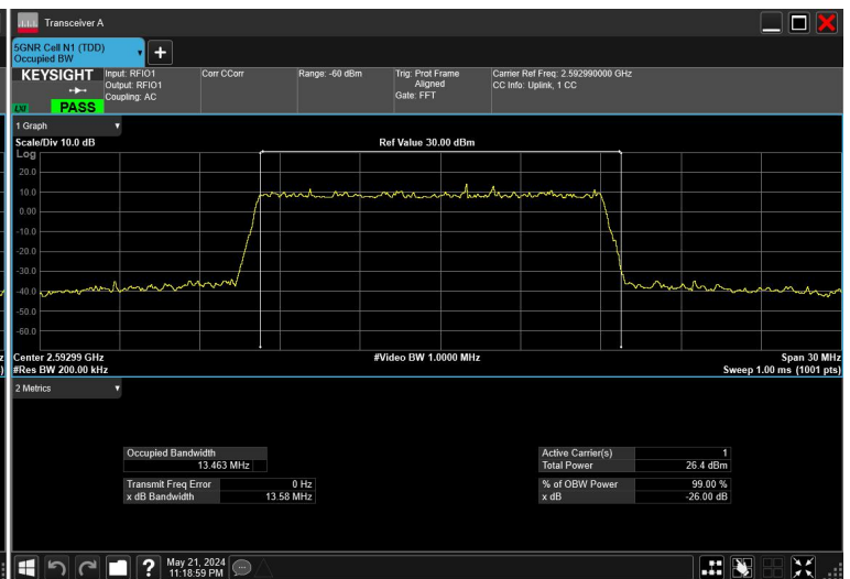
15MHz_30kHz_2592.99MHz_DFT-s-OFDM 64 QAM_RB36@0
