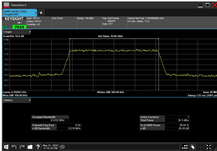
10MHz_30kHz_2592.99MHz_DFT-s-OFDM 64 QAM_RB24@0
