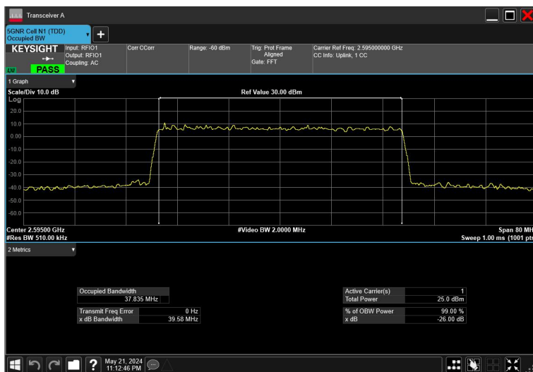
40MHz_30kHz_2595MHz_CP-OFDM 256 QAM_RB106@0
