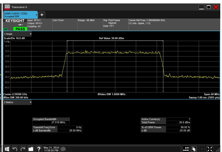
30MHz_30kHz_2595MHz_DFT-s-OFDM 256 QAM_RB75@0
