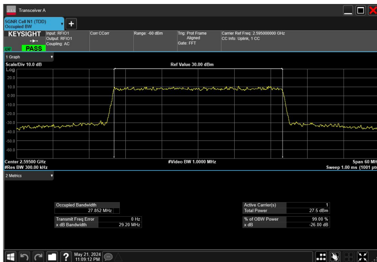
30MHz_30kHz_2595MHz_CP-OFDM 64 QAM_RB78@0
