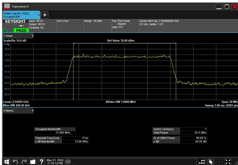
15MHz_30kHz_2592.99MHz_DFT-s-OFDM 256 QAM_RB36@0
