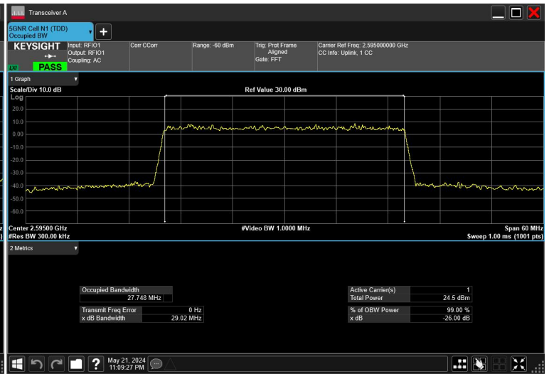
30MHz_30kHz_2595MHz_CP-OFDM 256 QAM_RB78@0
