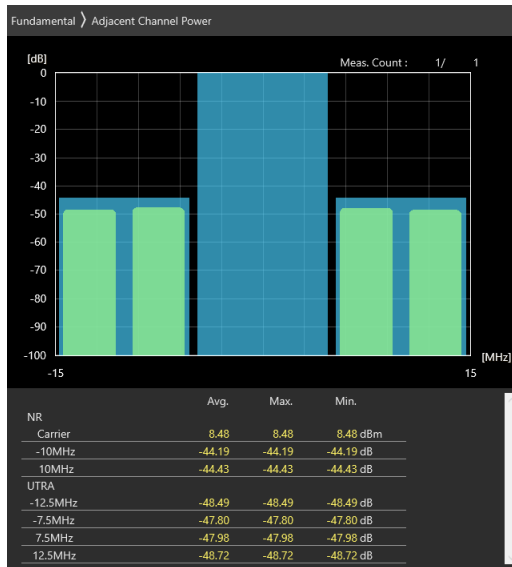
10MHz_30kHz_3555MHz_DFT-s-OFDM 64 QAM_RB24@0 -44.19 dB,-44.43 dB
