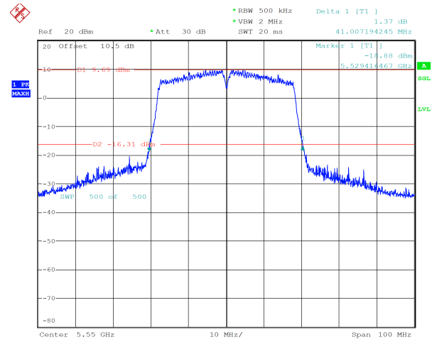
n40_5550MHz_Chain 1 41.007 MHz
