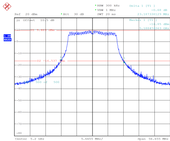
n20_5200MHz_Chain 1 23.187 MHz
