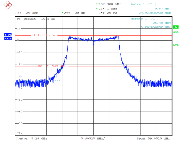
ax20_5280MHz_RU_242/61_Chain 1 24.924 MHz
