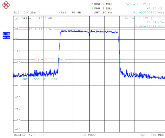
ac80_5530MHz_Chain 1 81.055 MHz
