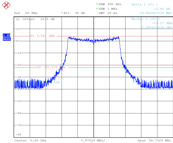
ax20_5260MHz_RU_242/61_Chain 1 24.468 MHz
