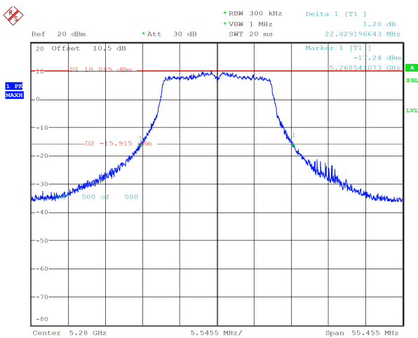
a_5280MHz_Chain 1 22.829 MHz
