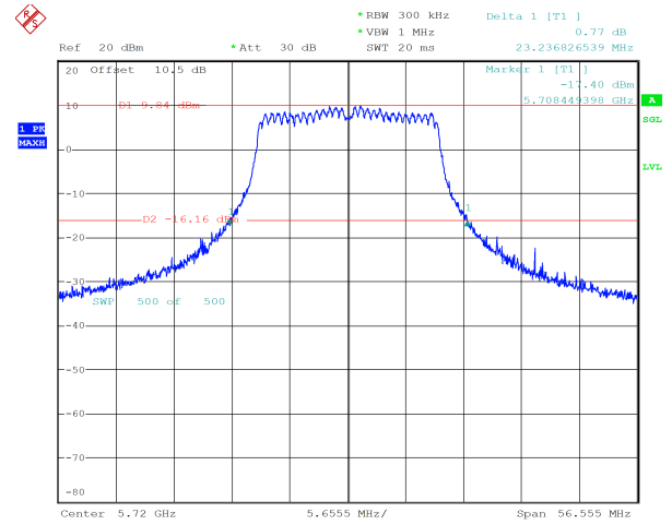
n20_5720MHz_Chain 1 23.237 MHz
