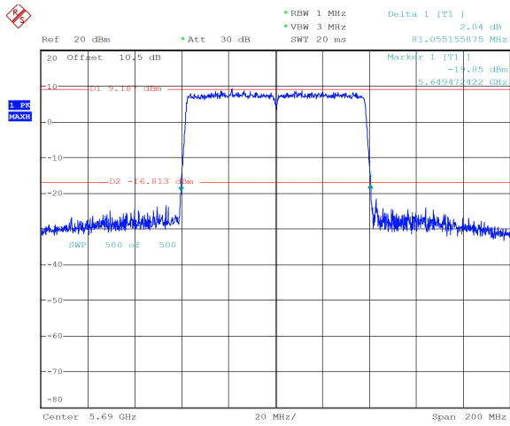
ac80_5690MHz_Chain 1 81.055 MHz
