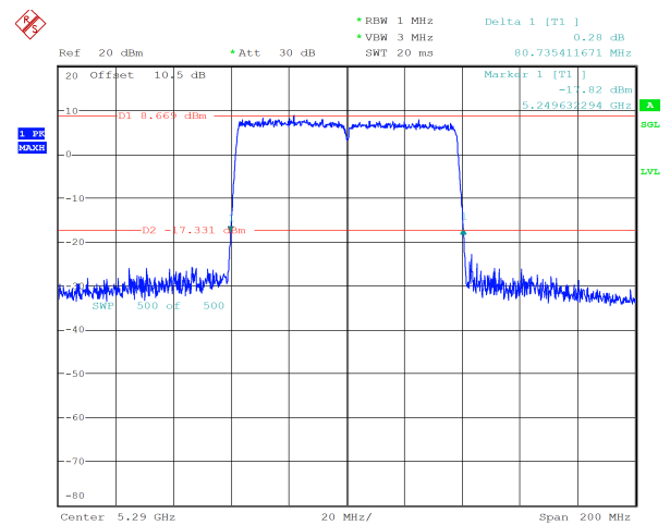
ac80_5290MHz_Chain 1 80.735 MHz
