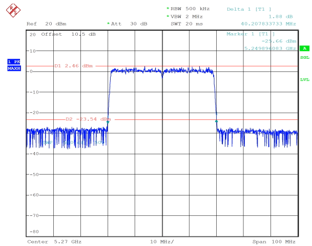
ax40_5270MHz_RU_484/65_Chain 1 40.208 MHz
