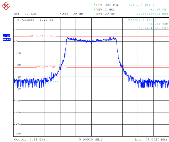
ax20_5320MHz_RU_242/61_Chain 1 24.357 MHz
