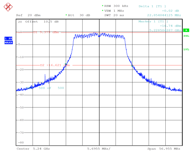
n20_5240MHz_Chain 1 22.855 MHz
