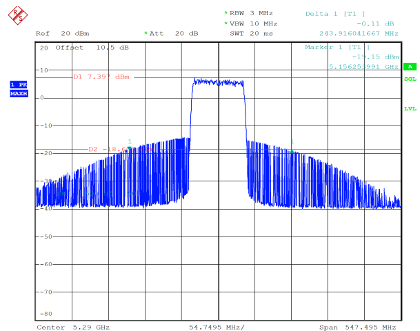
ax80_5290MHz_RU_996/67_Chain 1
