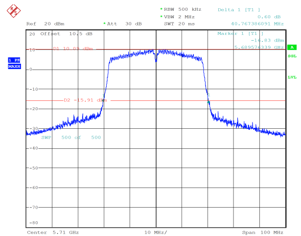
n40_5710MHz_Chain 1 40.767 MHz
