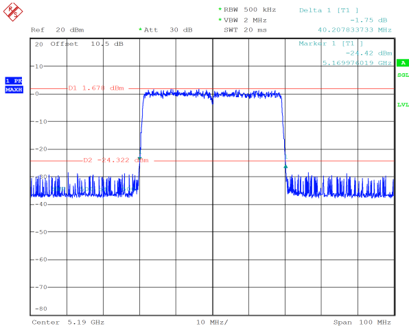
ax40_5190MHz_RU_484/65_Chain 1 40.208 MHz
