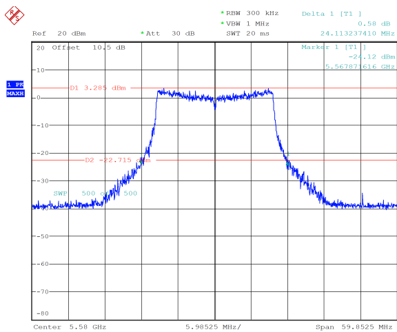
ax20_5580MHz_RU_242/61_Chain 1 24.113 MHz
