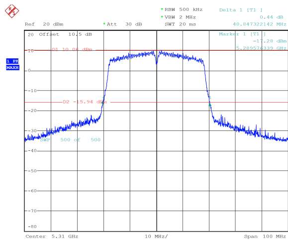
n40_5310MHz_Chain 1 40.847 MHz
