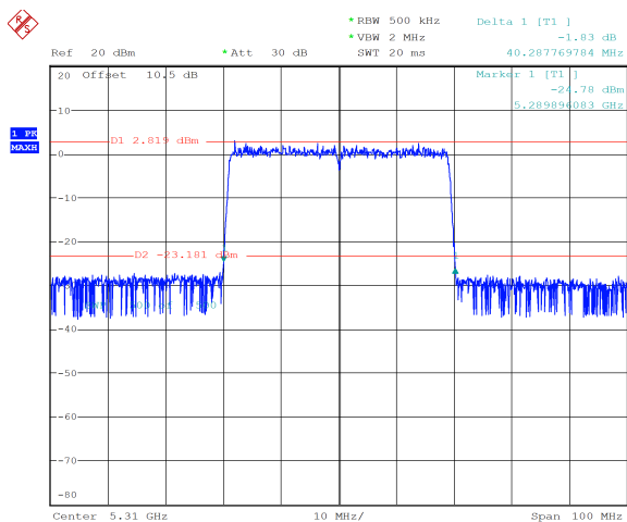
ax40_5310MHz_RU_484/65_Chain 1 40.288 MHz
