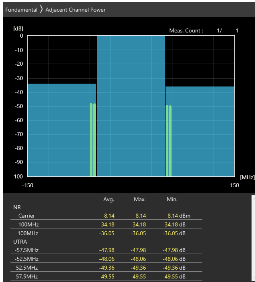
100MHz_30kHz_3600MHz_DFT-s-OFDM 64 QAM_RB270@0 -34.18 dB,-36.05 dB
