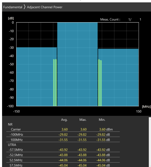
100MHz_30kHz_3650MHz_CP-OFDM 256 QAM_RB1@272 -29.82 dB,-31.55 dB
