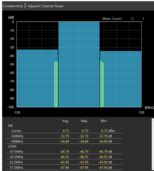
100MHz_30kHz_3650MHz_CP-OFDM 64 QAM_RB1@272 -32.79 dB,-34.49 dB
