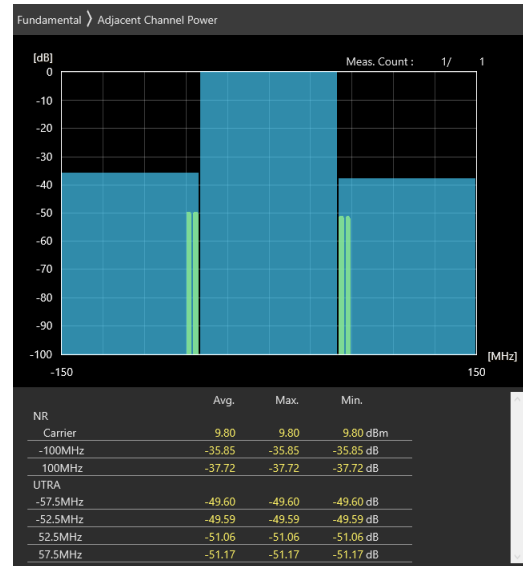
100MHz_30kHz_3600MHz_DFT-s-OFDM 16 QAM_RB135@67 -35.85 dB,-37.72 dB
