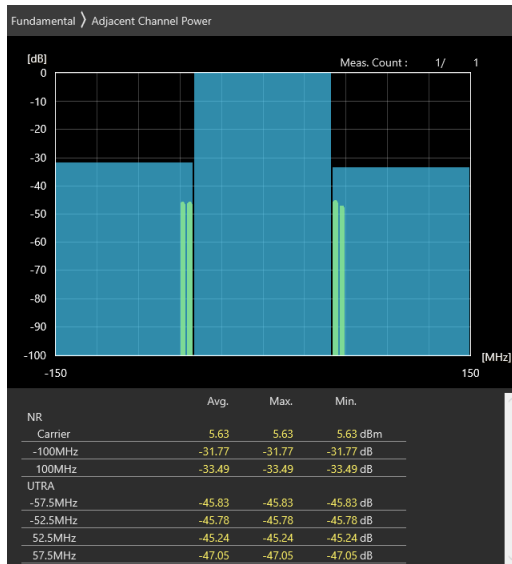
100MHz_30kHz_3650MHz_DFT-s-OFDM 256 QAM_RB1@272 -31.77 dB,-33.49 dB
