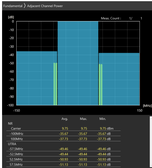
100MHz_30kHz_3650MHz_DFT-s-OFDM 16 QAM_RB135@67 -35.67 dB,-37.73 dB
