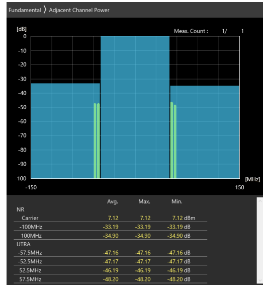
100MHz_30kHz_3650MHz_CP-OFDM 16 QAM_RB1@272 -33.19 dB,-34.9 dB
