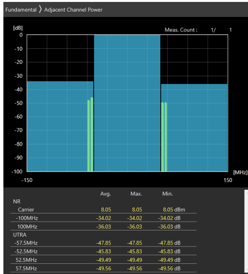
100MHz_30kHz_3600MHz_DFT-s-OFDM 16 QAM_RB1@0 -34.02 dB,-36.03 dB
