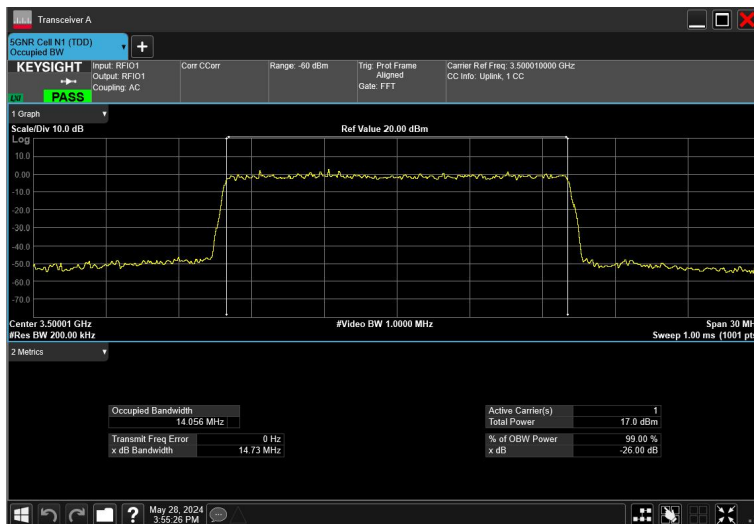
15MHz_15kHz_3500MHz_CP-OFDM64QAM_RB79@0
