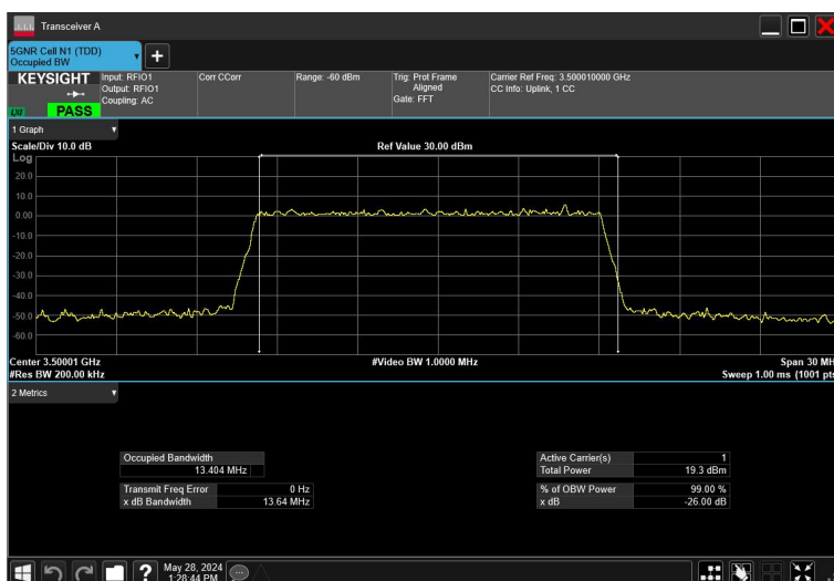
15MHz_30kHz_3500MHz_DFT-s-OFDM QPSK_RB36@0
