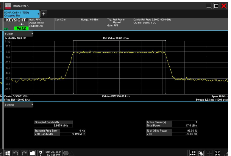
10MHz_30kHz_3500MHz_DFT-s-OFDM 64QAM_RB24@0
