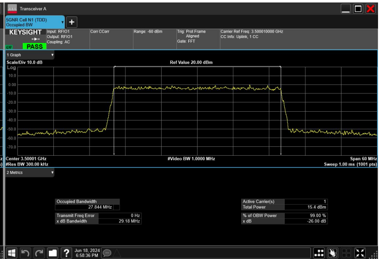
30MHz_30kHz_3500MHz_CP-OFDM256QAM_RB78@0
