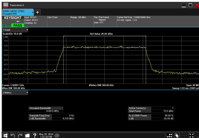
10MHz_30kHz_3500MHz_DFT-s-OFDM 256QAM_RB24@0
