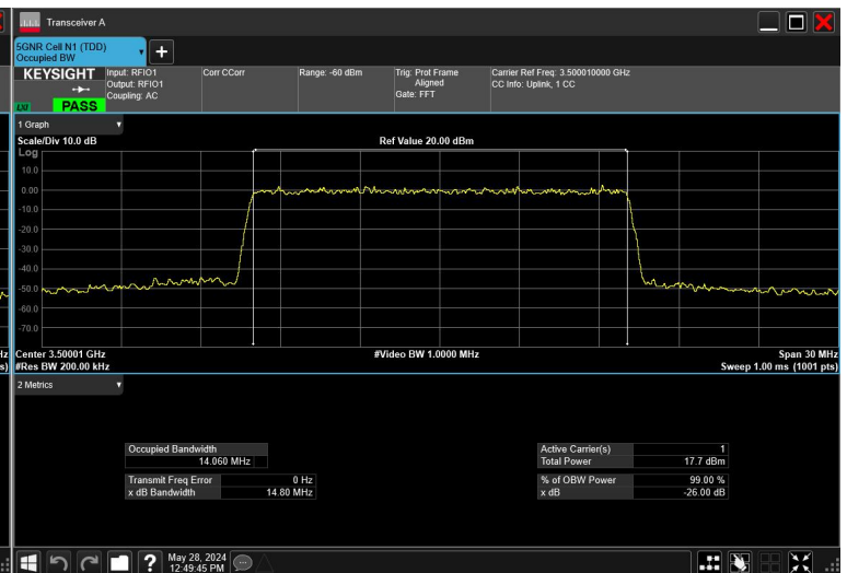
15MHz_15kHz_3500MHz_CP-OFDM QPSK_RB79@0
