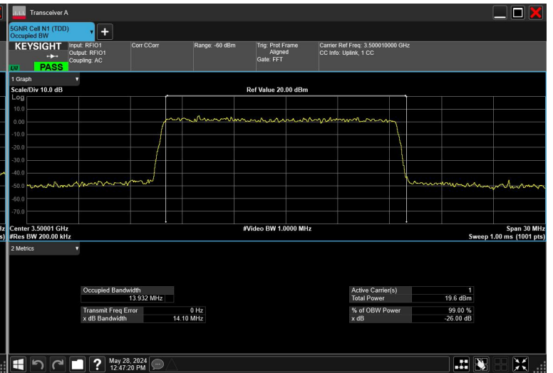
15MHz_15kHz_3500MHz_DFT-s-OFDM QPSK_RB75@0
