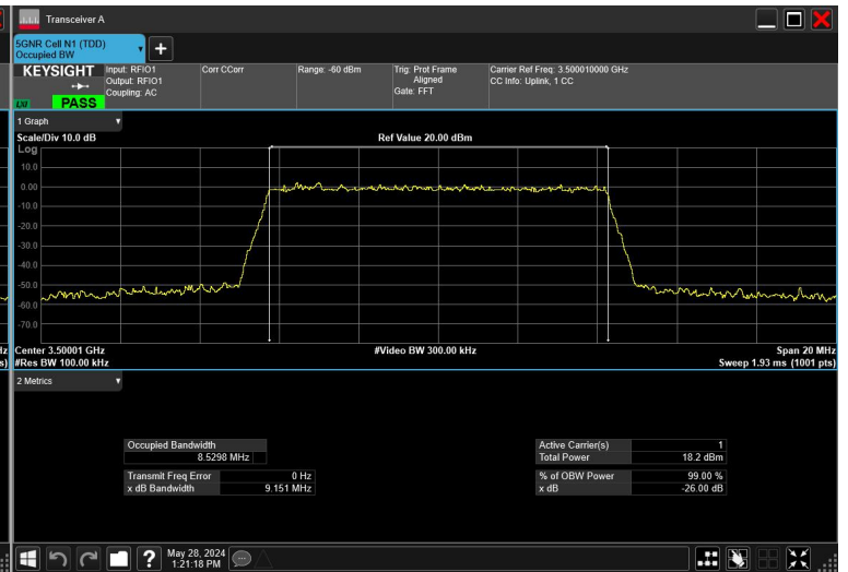
10MHz_30kHz_3500MHz_DFT-s-OFDM 16QAM_RB24@0
