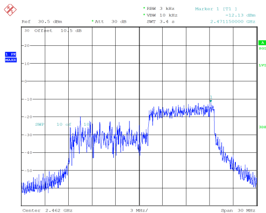
ax20_2462MHz_RU_106/54_Chain 0 -12.13 dBm/3kHz
