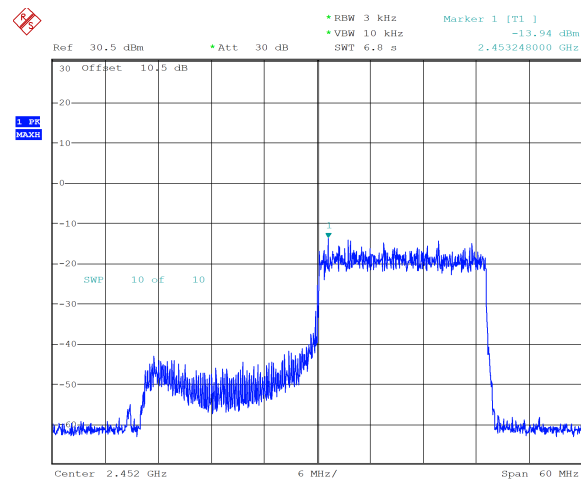
ax40_2452MHz_RU_242/62_Chain 0 -13.94 dBm/3kHz
