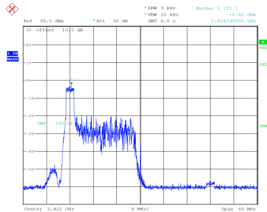
ax40_2422MHz_RU_26/0_Chain 1 -2.62 dBm/3kHz
