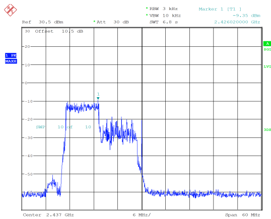
ax40_2437MHz_RU_106/53_Chain 0 -9.35 dBm/3kHz
