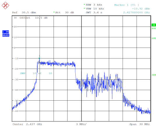
ax20_2437MHz_RU_106/53_Chain 0 -10.92 dBm/3kHz
