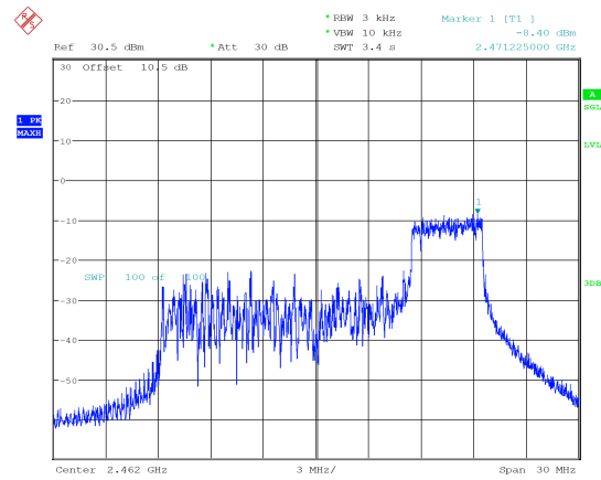
ax20_2462MHz_RU_52/40_Chain 1 -8.40 dBm/3kHz
