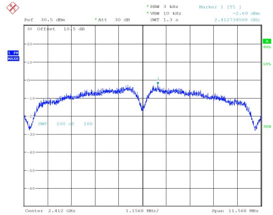
b_2412MHz_Chain 1 -2.69 dBm/3kHz
