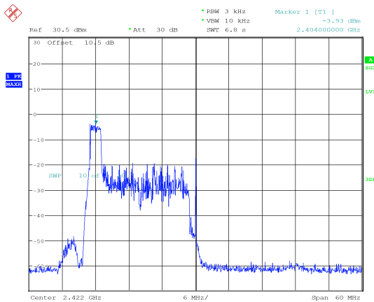
ax40_2422MHz_RU_26/0_Chain 0 -3.93 dBm/3kHz
