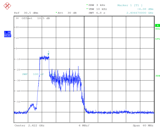
ax40_2422MHz_RU_52/37_Chain 1 -6.08 dBm/3kHz
