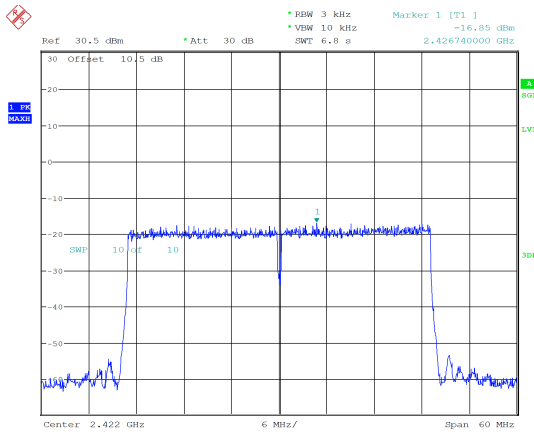
ax40_2422MHz_RU_Full_Chain 0 -16.85 dBm/3kHz
