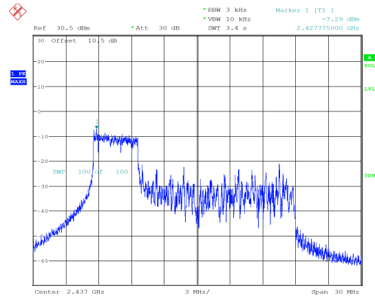
ax20_2437MHz_RU_52/37_Chain 1 -7.29 dBm/3kHz
