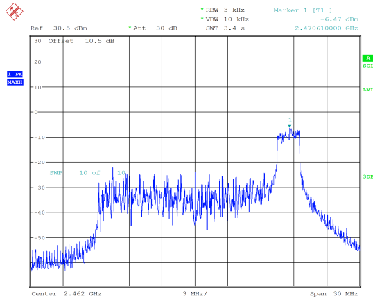
ax20_2462MHz_RU_26/8_Chain 0 -6.47 dBm/3kHz
