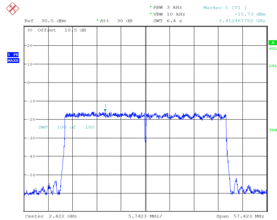
ax40_2422MHz_RU_Full_Chain 1 -15.73 dBm/3kHz
