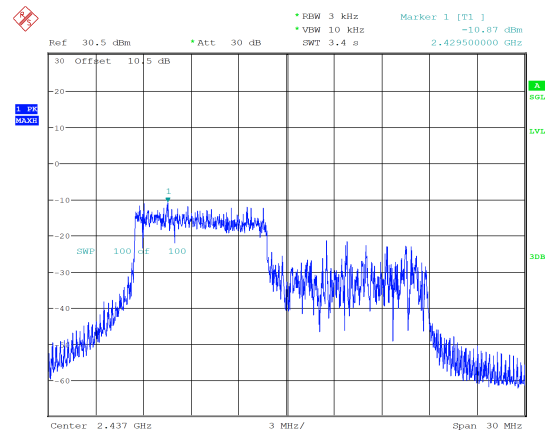
ax20_2437MHz_RU_106/53_Chain 1 -10.87 dBm/3kHz
