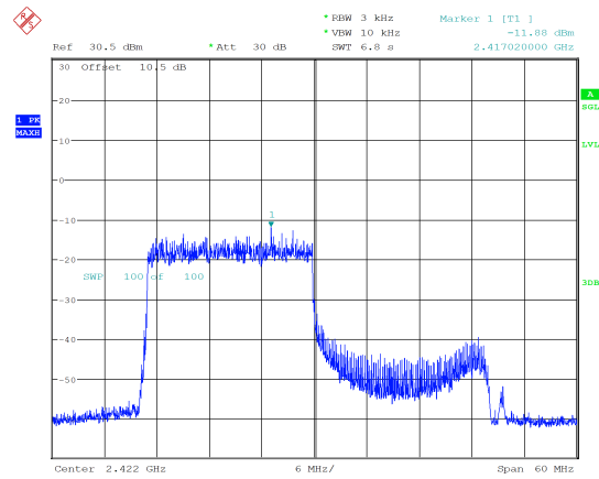
ax40_2422MHz_RU_242/61_Chain 1 -11.88 dBm/3kHz
