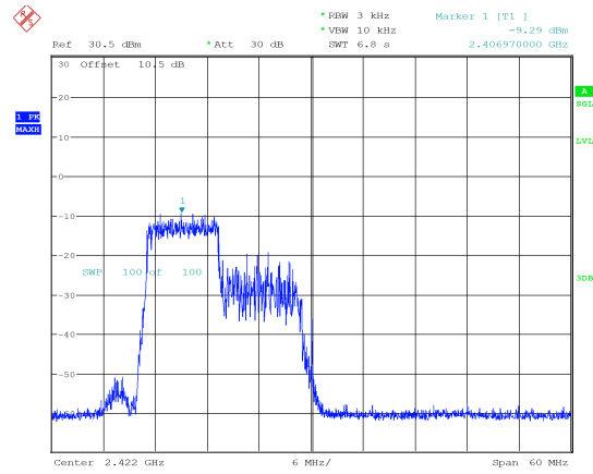
ax40_2422MHz_RU_106/53_Chain 1 -9.29 dBm/3kHz
