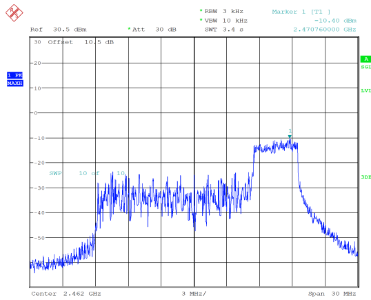
ax20_2462MHz_RU_52/40_Chain 0 -10.40 dBm/3kHz
