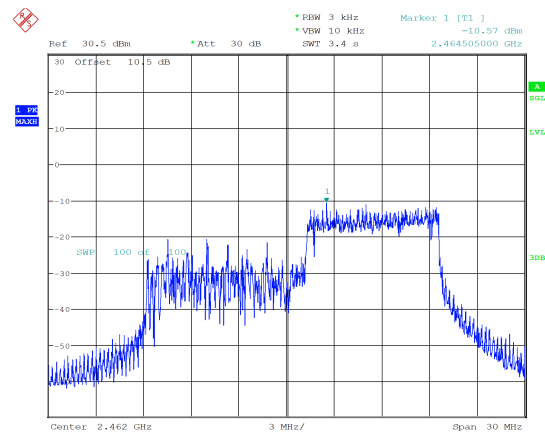
ax20_2462MHz_RU_106/54_Chain 1 -10.57 dBm/3kHz
