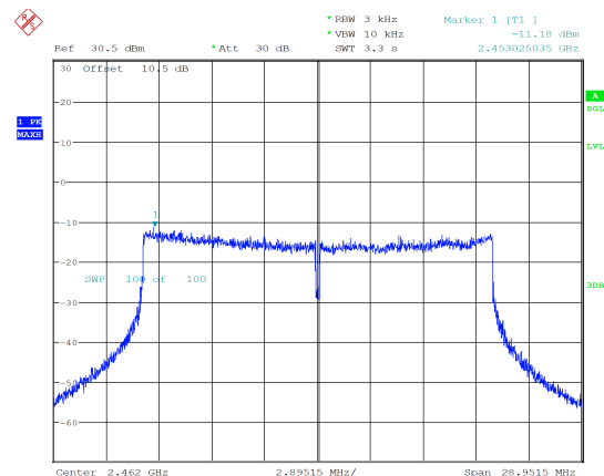
ax20_2462MHz_RU_Full_Chain 1 -11.18 dBm/3kHz
