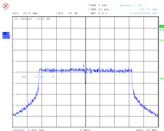
ax20_2462MHz_RU_Full_Chain 0 -14.73 dBm/3kHz
