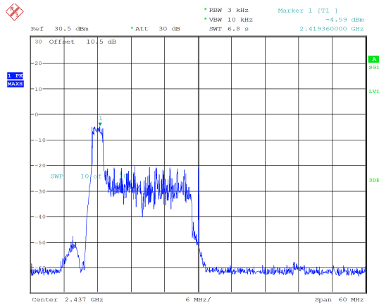
ax40_2437MHz_RU_26/0_Chain 0 -4.59 dBm/3kHz
