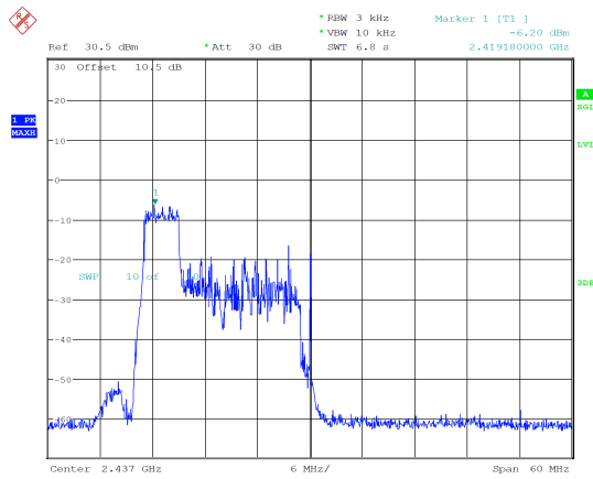
ax40_2437MHz_RU_52/37_Chain 0 -6.20 dBm/3kHz
