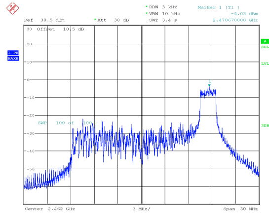
ax20_2462MHz_RU_26/8_Chain 1 -4.03 dBm/3kHz
