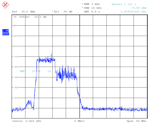
ax40_2422MHz_RU_106/53_Chain 0 -9.49 dBm/3kHz
