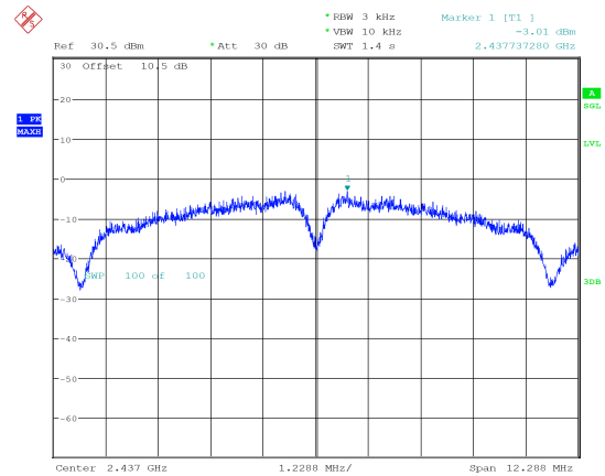
b_2437MHz_Chain 1 -3.01 dBm/3kHz
