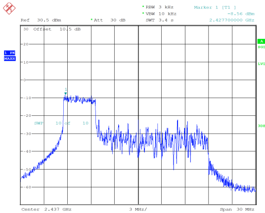
ax20_2437MHz_RU_52/37_Chain 0 -8.56 dBm/3kHz
