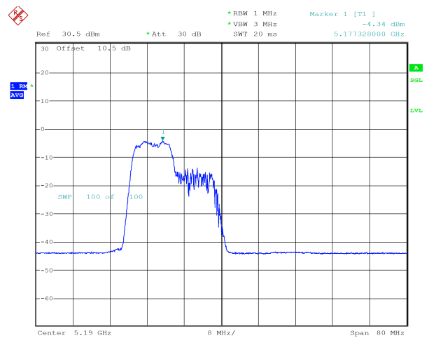
ax40_5190MHz_RU_106/53_Chain 1 -4.34 dBm
