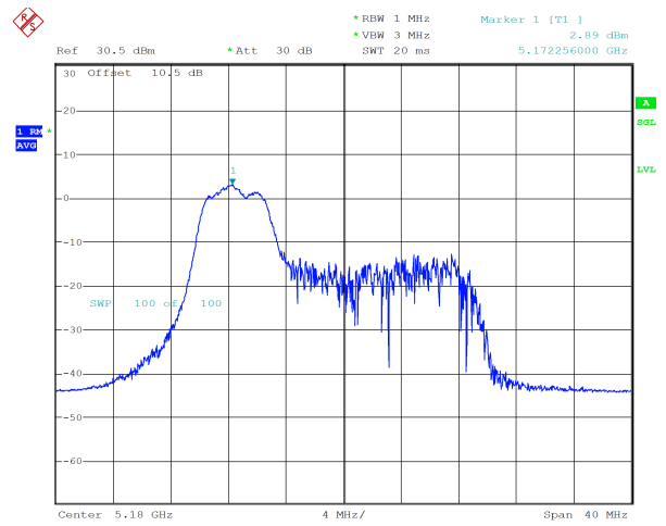
ax20_5180MHz_RU_52/37_Chain 1 2.89 dBm
