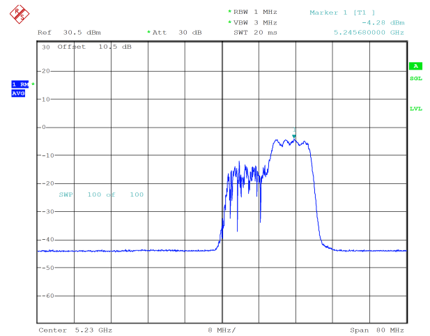
ax40_5230MHz_RU_106/56_Chain 1 -4.28 dBm
