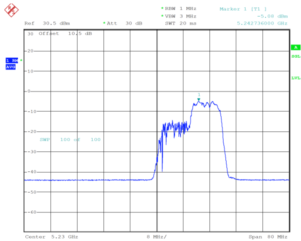
ax40_5230MHz_RU_106/56_Chain 0 -5.08 dBm
