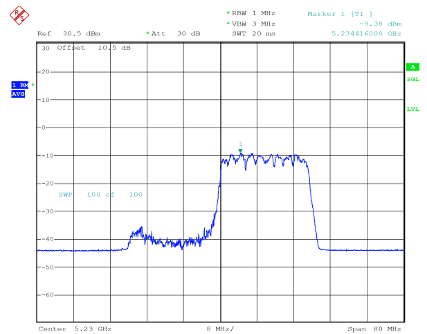
ax40_5230MHz_RU_242/62_Chain 1 -9.38 dBm
