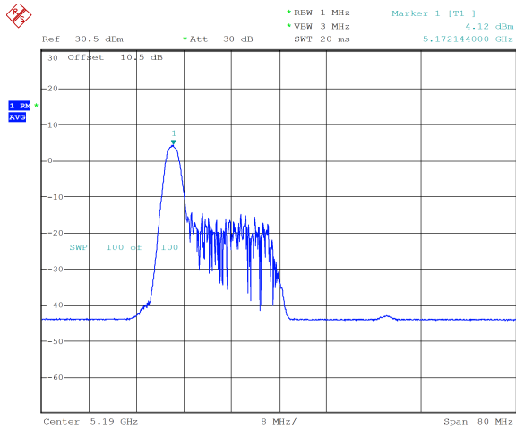
ax40_5190MHz_RU_26/0_Chain 0 4.12 dBm
