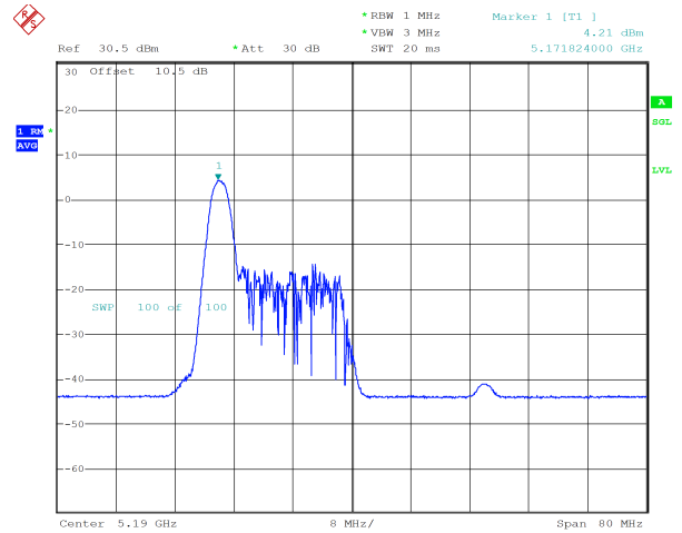
ax40_5190MHz_RU_26/0_Chain 1 4.21 dBm
