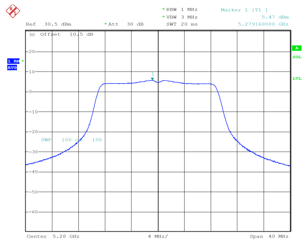
n20_5280MHz_Chain 1 5.47 dBm
