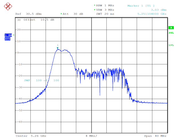
ax20_5260MHz_RU_52/37_Chain 1 3.03 dBm
