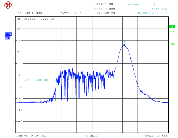
ax20_5260MHz_RU_26/0_Chain 1 5.45 dBm
