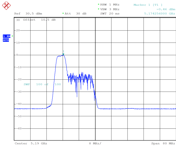
ax40_5190MHz_RU_52/37_Chain 0 -0.46 dBm
