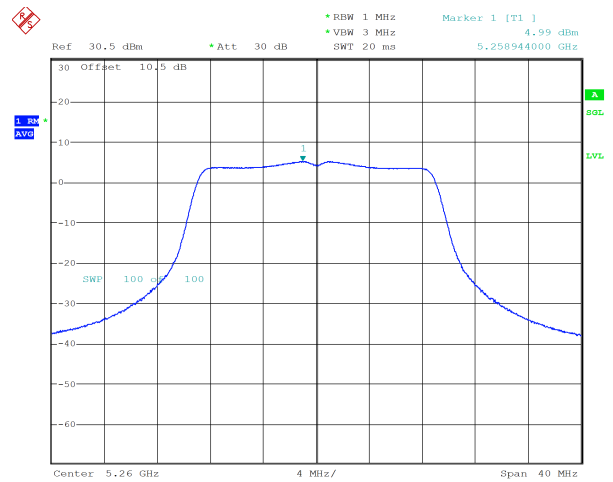
n20_5260MHz_Chain 1 4.99 dBm
