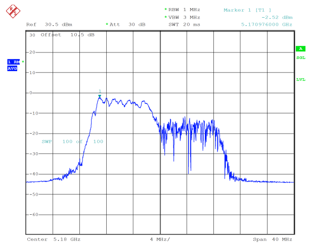
ax20_5180MHz_RU_106/53_Chain 1 -2.52 dBm
