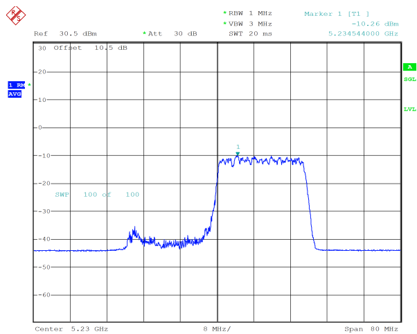
ax40_5230MHz_RU_242/62_Chain 0 -10.26 dBm
