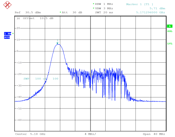
ax20_5180MHz_RU_26/0_Chain 1 5.71 dBm
