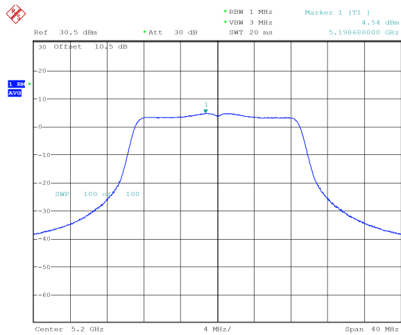
n20_5200MHz_Chain 0 4.54 dBm
