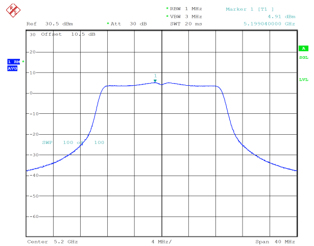
n20_5200MHz_Chain 1 4.91 dBm
