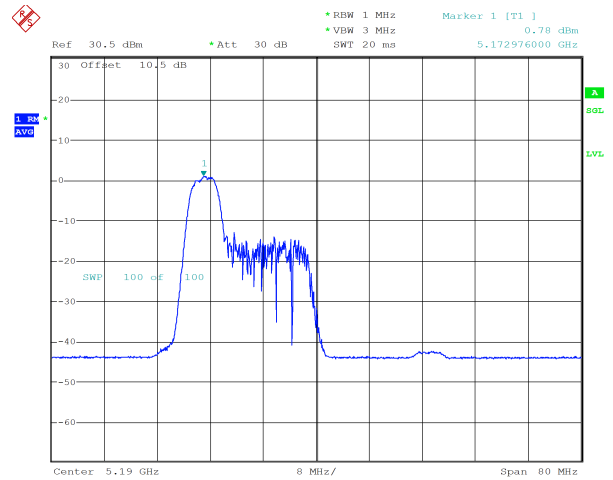
ax40_5190MHz_RU_52/37_Chain 1 0.78 dBm
