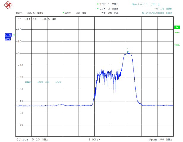
ax40_5230MHz_RU_52/44_Chain 1 -0.14 dBm
