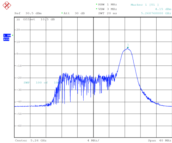
ax20_5260MHz_RU_26/0_Chain 0 5.17 dBm
