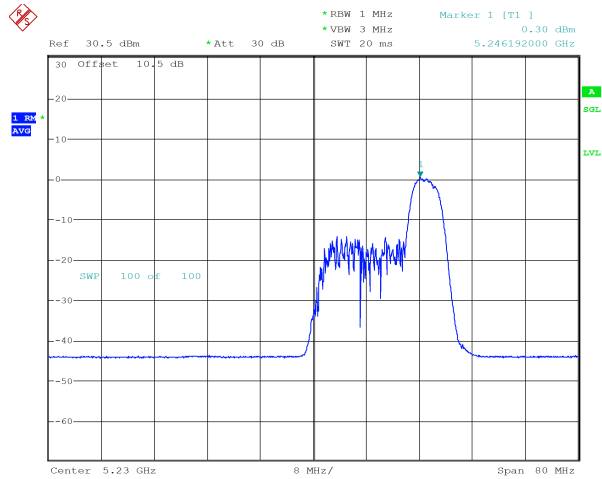
ax40_5230MHz_RU_52/44_Chain 0 0.30 dBm
