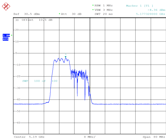
ax40_5190MHz_RU_106/53_Chain 0 -4.36 dBm
