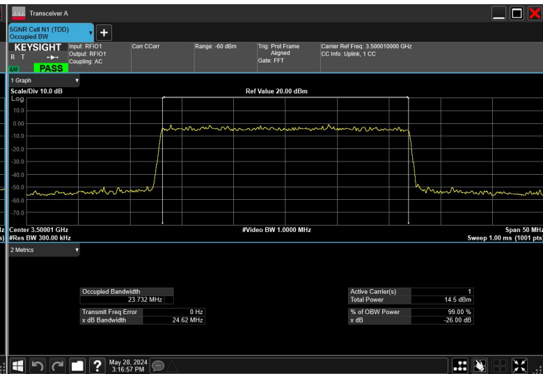
25MHz_15kHz_3500MHz_CP-OFDM256QAM_RB133@0
