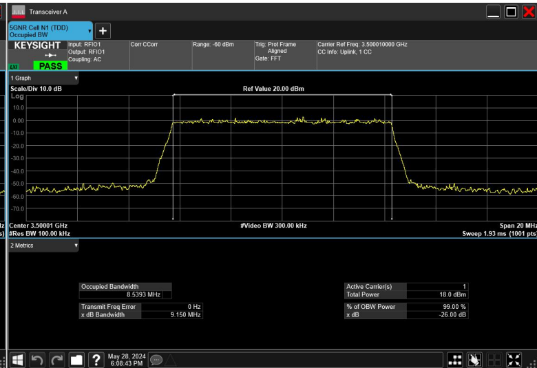
10MHz_30kHz_3500MHz_DFT-s-OFDM 16QAM_RB24@0
