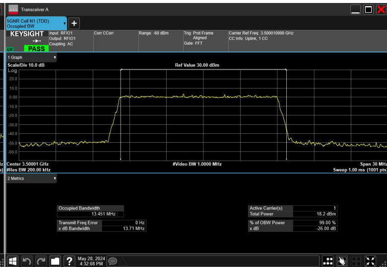
15MHz_30kHz_3500MHz_DFT-s-OFDM 16QAM_RB36@0
