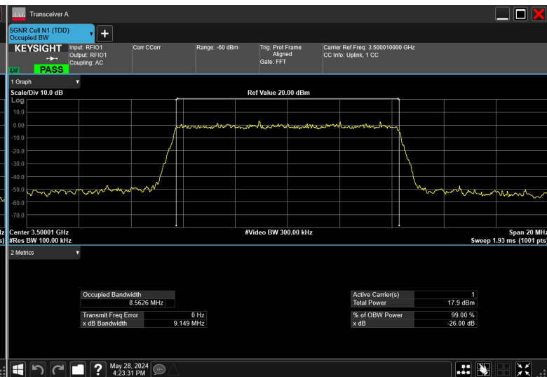
10MHz_30kHz_3500MHz_DFT-s-OFDM 64QAM_RB24@0
