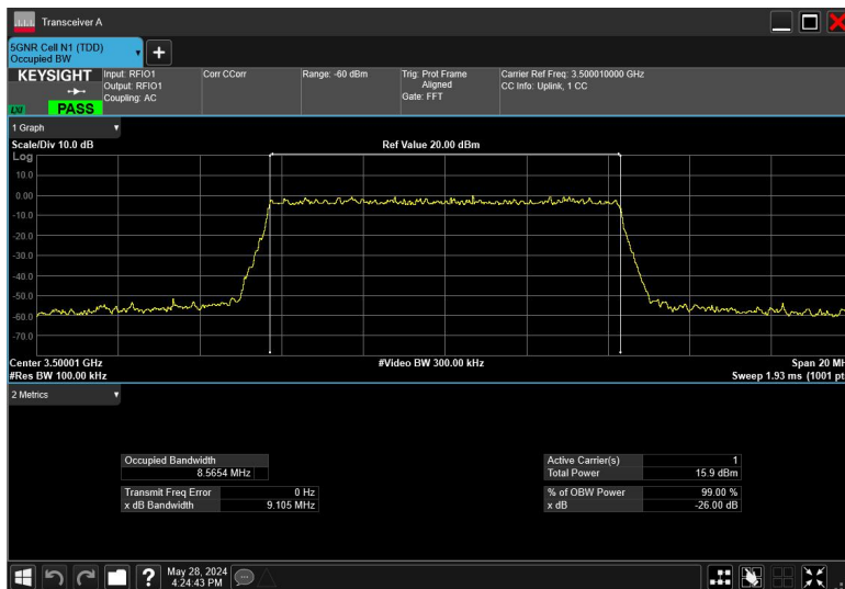
10MHz_30kHz_3500MHz_DFT-s-OFDM 256QAM_RB24@0
