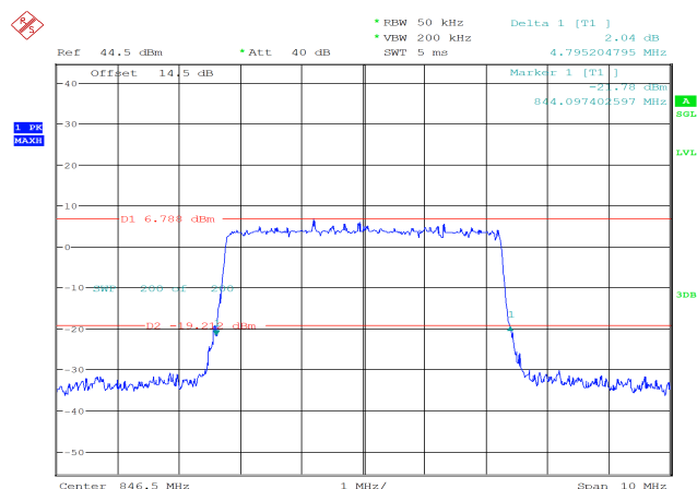
26dB Bandwidth 4.795MHz
