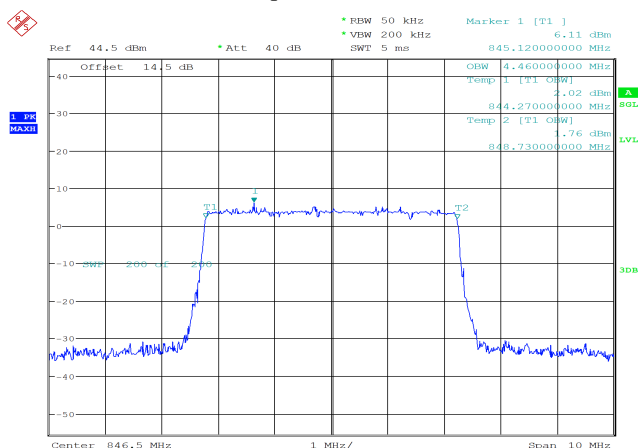
99% Occupied Bandwidth 4.46 MHz
