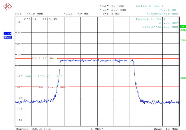
26dB Bandwidth 4.835MHz
