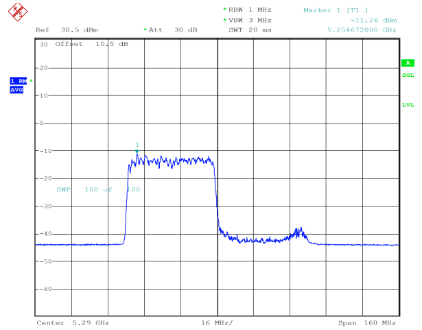
ax80_5290MHz_RU_484/65_Chain 1 -11.26 dBm
