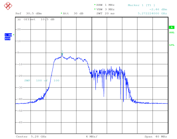
ax20_5280MHz_RU_106/53_Chain 1 -2.46 dBm
