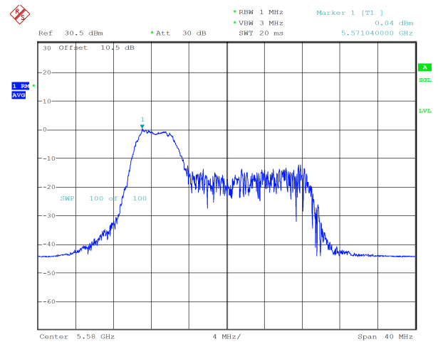
ax20_5580MHz_RU_52/37_Chain 1 0.04 dBm
