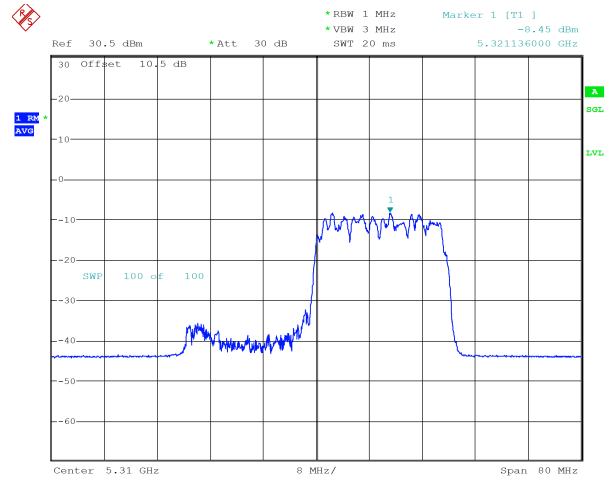
ax40_5310MHz_RU_242/62_Chain 1 -8.45 dBm
