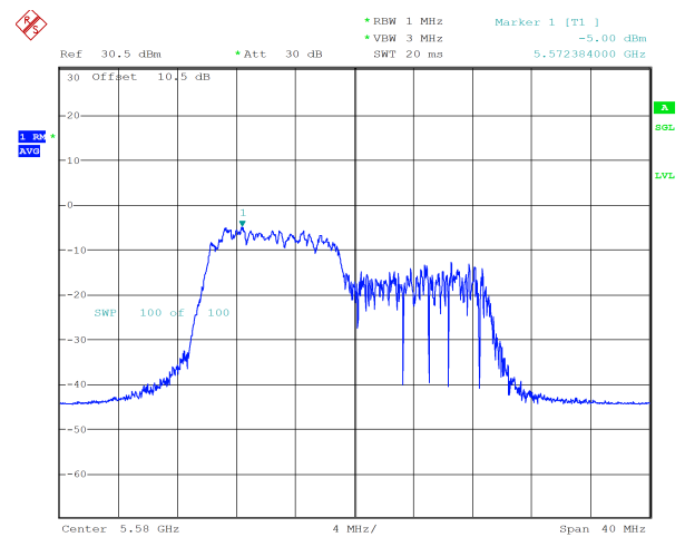
ax20_5580MHz_RU_106/53_Chain 1 -5.00 dBm
