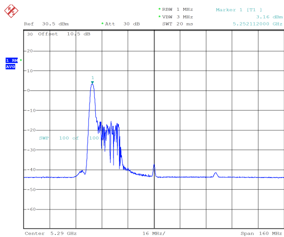
ax80_5290MHz_RU_26/0_Chain 0 3.16 dBm
