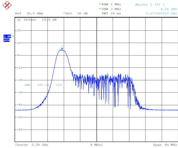
ax20_5580MHz_RU_26/0_Chain 0 4.26 dBm
