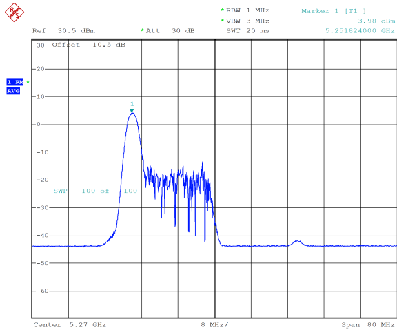
ax40_5270MHz_RU_26/0_Chain 0 3.98 dBm
