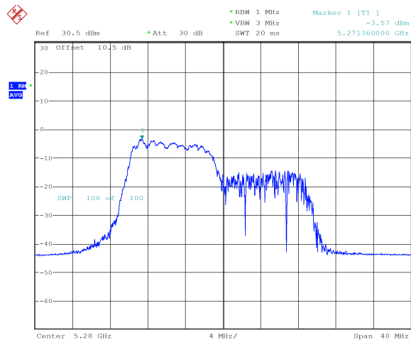
ax20_5280MHz_RU_106/53_Chain 0 -3.57 dBm
