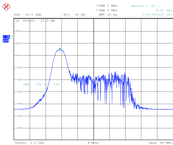
ax20_5500MHz_RU_26/0_Chain 0 4.43 dBm
