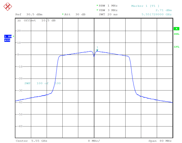
n40_5550MHz_Chain 1 2.71 dBm
