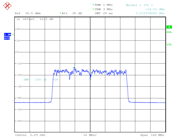
ax80_5290MHz_RU_996/67_Chain 1 -14.51 dBm
