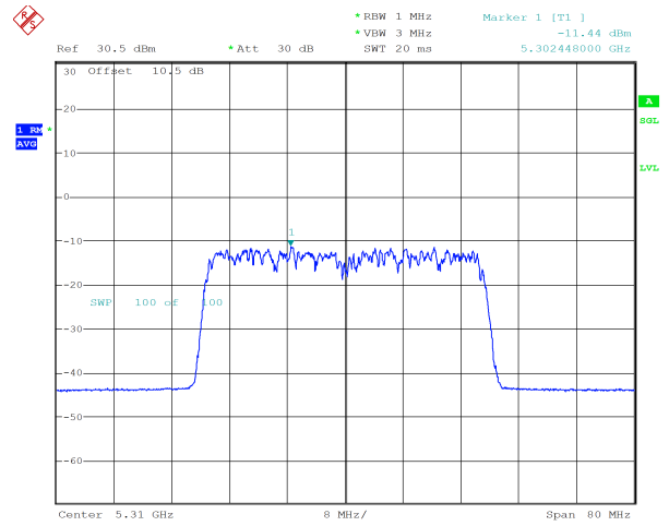
ax40_5310MHz_RU_484/65_Chain 1 -11.44 dBm
