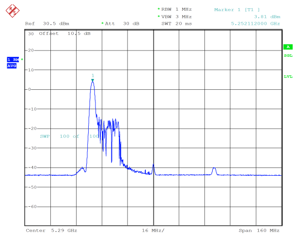
ax80_5290MHz_RU_26/0_Chain 1 3.81 dBm
