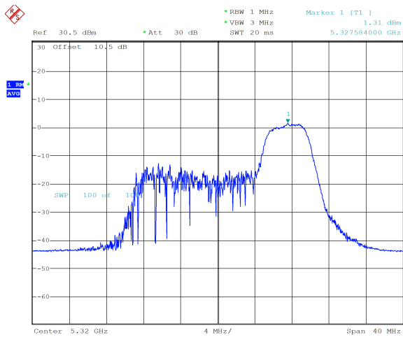
ax20_5320MHz_RU_52/40_Chain 0 1.31 dBm
