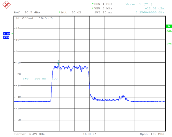
ax80_5290MHz_RU_484/65_Chain 0 -12.32 dBm
