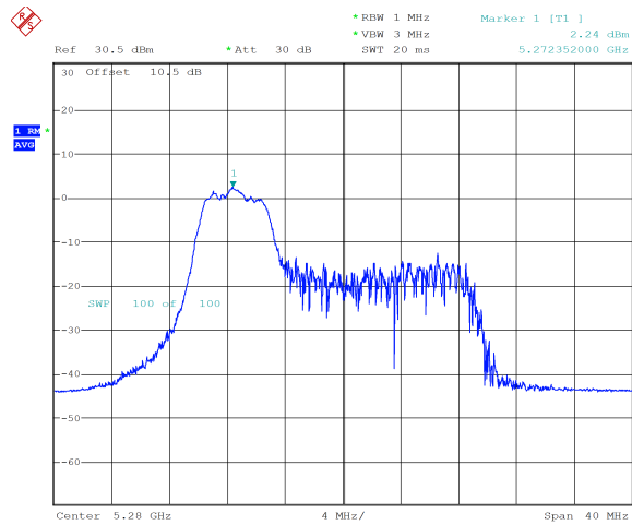
ax20_5280MHz_RU_52/37_Chain 0 2.24 dBm
