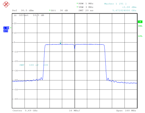
ac80_5690MHz_Chain 1 -2.08 dBm
