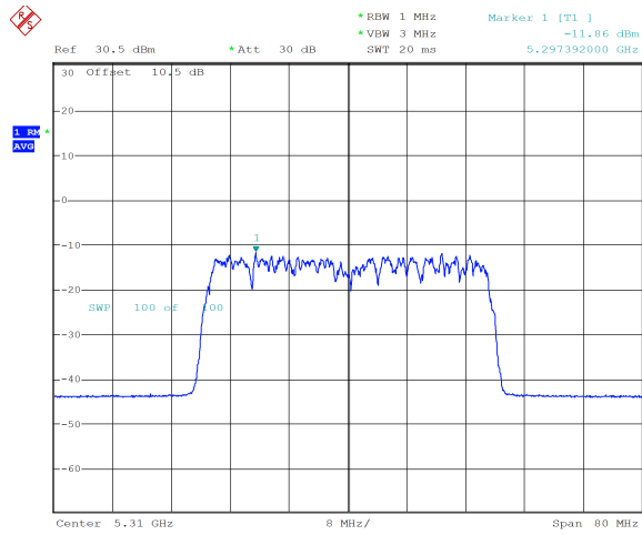
ax40_5310MHz_RU_484/65_Chain 0 -11.86 dBm
