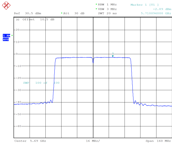
ac80_5690MHz_Chain 0 -2.89 dBm
