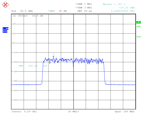
ax80_5290MHz_RU_996/67_Chain 0 -15.22 dBm
