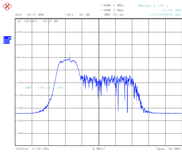
ax20_5580MHz_RU_52/37_Chain 0 -1.61 dBm
