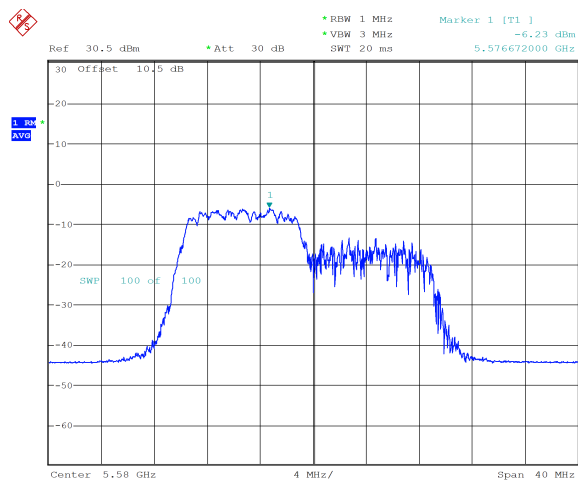
ax20_5580MHz_RU_106/53_Chain 0 -6.23 dBm
