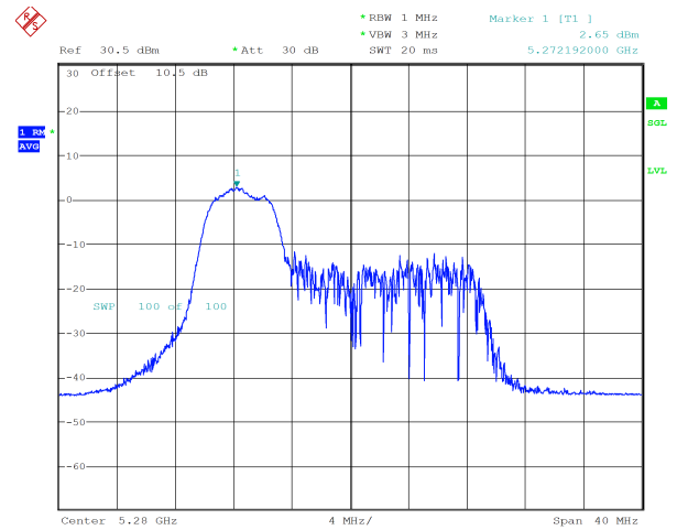
ax20_5280MHz_RU_52/37_Chain 1 2.65 dBm
