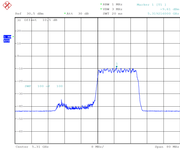
ax40_5310MHz_RU_242/62_Chain 0 -9.61 dBm
