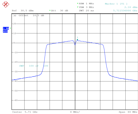
n40_5710MHz_Chain 0 2.18 dBm
