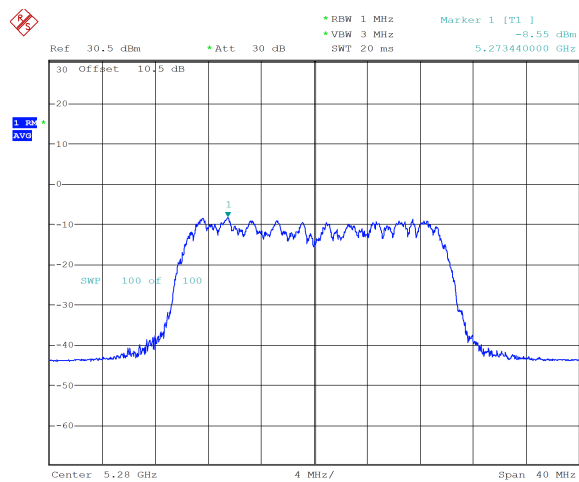
ax20_5280MHz_RU_242/61_Chain 0 -8.55 dBm
