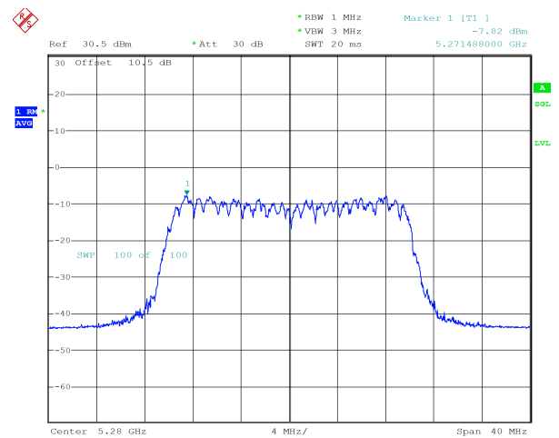
ax20_5280MHz_RU_242/61_Chain 1 -7.82 dBm
