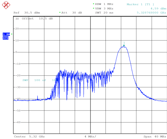
ax20_5320MHz_RU_26/8_Chain 0 5.22 dBm
