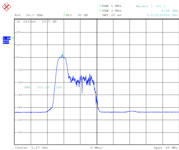
ax40_5270MHz_RU_52/37_Chain 0 0.46 dBm
