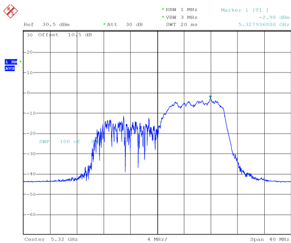
ax20_5320MHz_RU_106/54_Chain 0 -2.98 dBm
