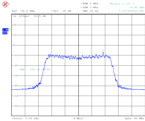
ax20_5320MHz_RU_242/61_Chain 0 -8.40 dBm
