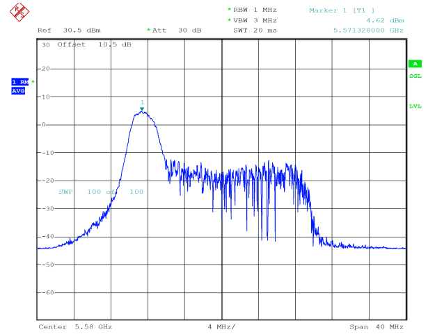
ax20_5580MHz_RU_26/0_Chain 1 4.62 dBm
