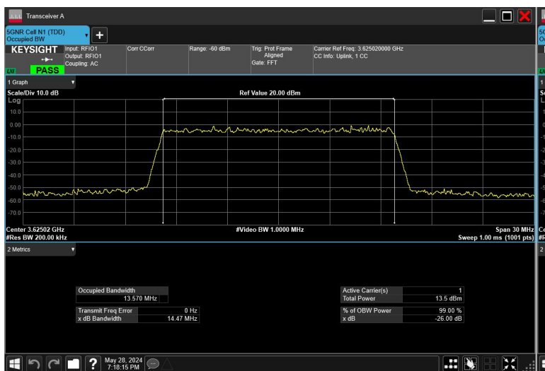
15MHz_30kHz_3625MHz_CP-OFDM 256QAM_RB38@0
