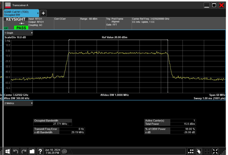
30MHz_30kHz_3625MHz_CP-OFDM256QAM_RB78@0
