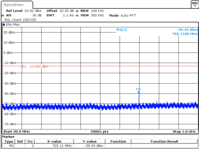
30MHz_30kHz_3500MHz_DFT-s-OFDM QPSK_RB1@77 -39.45 dBm
