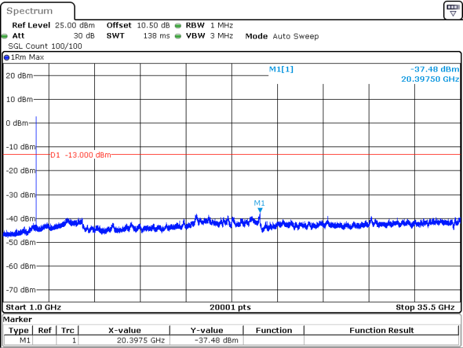
40MHz_30kHz_3470MHz_DFT-s-OFDM QPSK_RB1@105 -37.48 dBm
