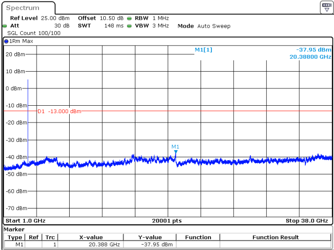
15MHz_15kHz_3707.5MHz_DFT-s-OFDM QPSK_RB1@78 -37.95 dBm
