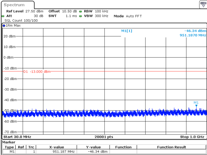
25MHz_30kHz_3500MHz_DFT-s-OFDM QPSK_RB1@64 -46.34 dBm
