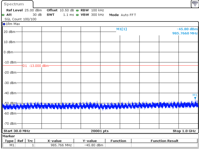
100MHz_30kHz_3500MHz_DFT-s-OFDM QPSK_RB1@272 -45.80 dBm
