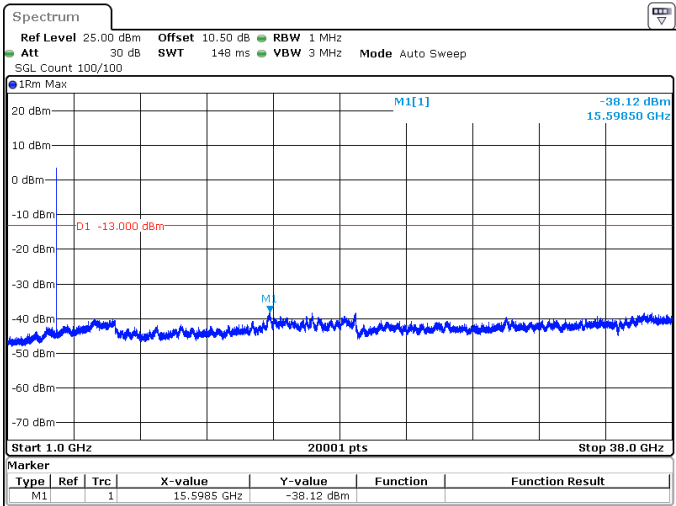
15MHz_15kHz_3707.5MHz_DFT-s-OFDM QPSK_RB1@0 -38.12 dBm
