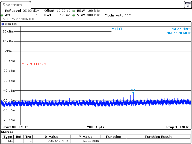
40MHz_30kHz_3470MHz_DFT-s-OFDM QPSK_RB100@0 -43.55 dBm
