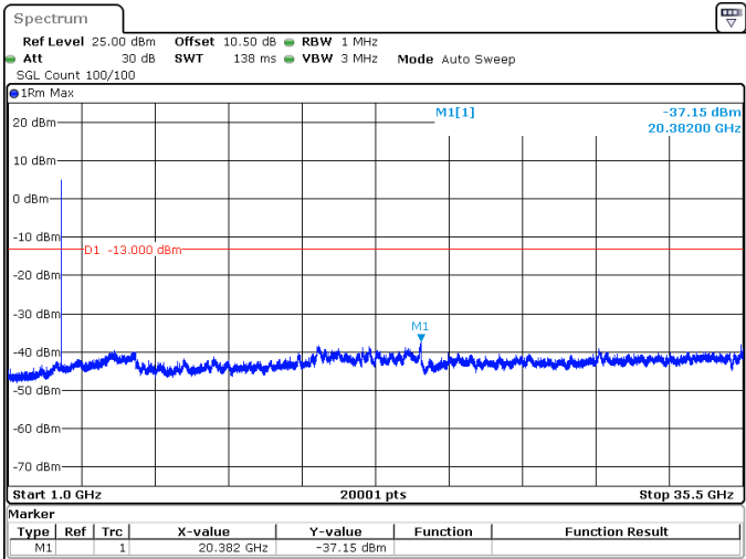
70MHz_30kHz_3515MHz_DFT-s-OFDM QPSK_RB1@0 -37.15 dBm
