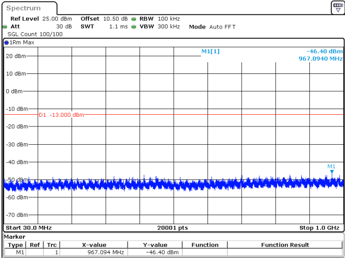
70MHz_30kHz_3515MHz_DFT-s-OFDM QPSK_RB1@188 -46.40 dBm
