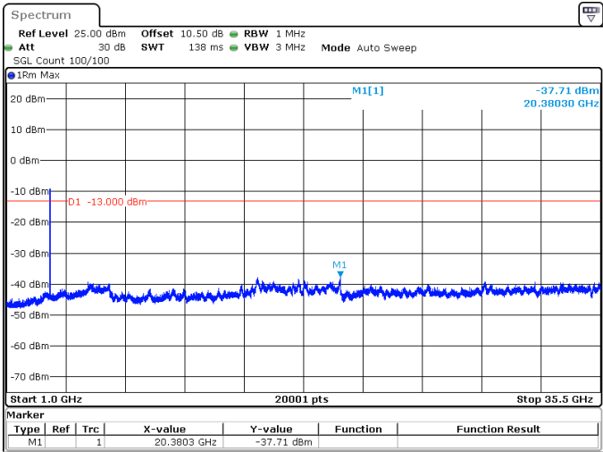
70MHz_30kHz_3515MHz_DFT-s-OFDM QPSK_RB180@0 -37.71 dBm
