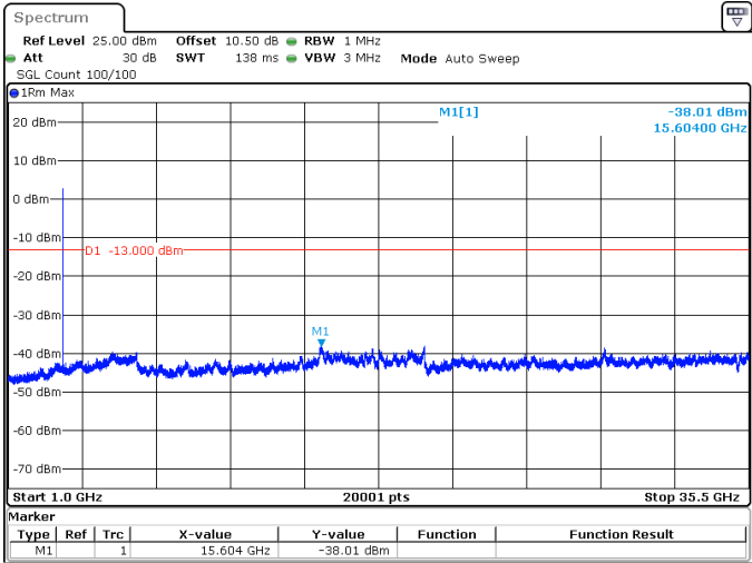
30MHz_30kHz_3535MHz_DFT-s-OFDM QPSK_RB1@77 -38.01 dBm
