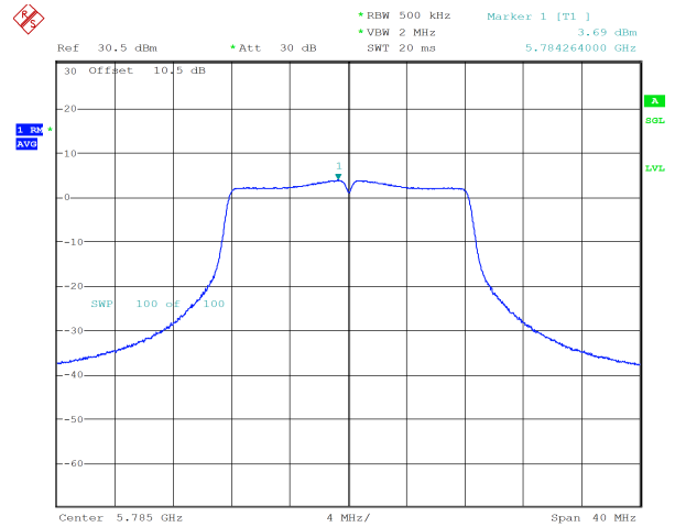
a_5785MHz_Chain 1 3.69 dBm
