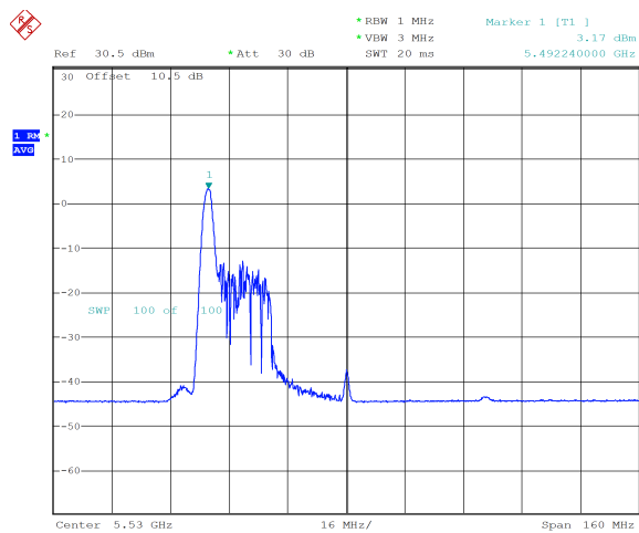
ax80_5530MHz_RU_26/0_Chain 0 3.17 dBm
