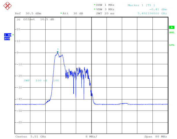
ax40_5510MHz_RU_52/37_Chain 1 -0.41 dBm
