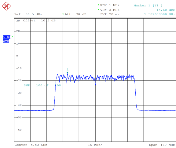
ax80_5530MHz_RU_996/67_Chain 0 -14.60 dBm
