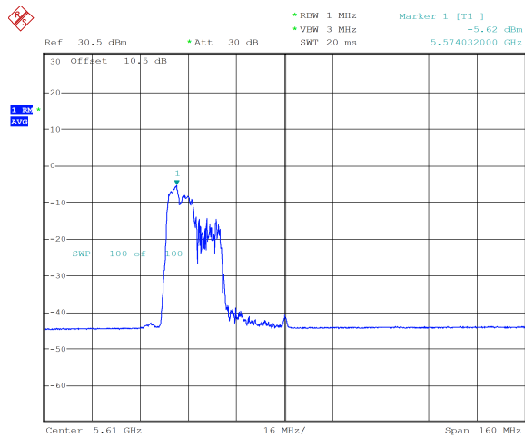
ax80_5610MHz_RU_106/53_Chain 0 -5.62 dBm
