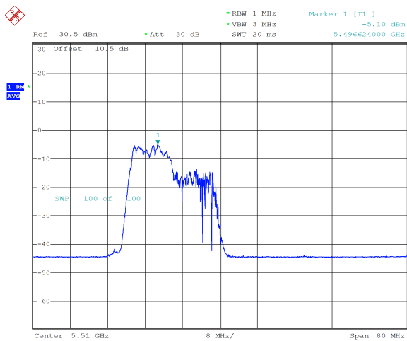
ax40_5510MHz_RU_106/53_Chain 0 -5.10 dBm
