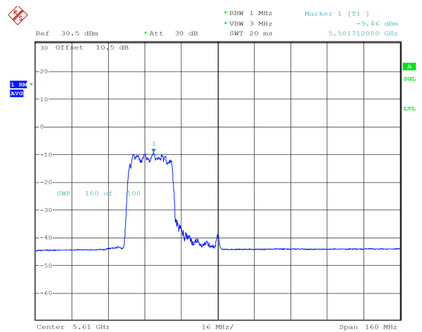
ax80_5610MHz_RU_242/61_Chain 1 -9.46 dBm
