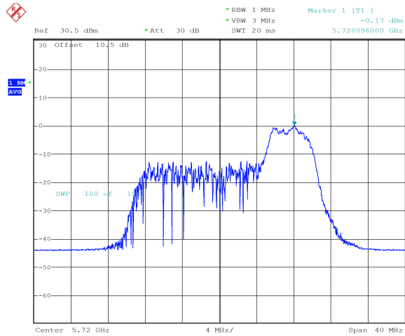
ax20_5720MHz_RU_52/40_Chain 0 -0.17 dBm
