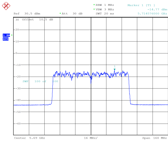
ax80_5690MHz_RU_996/67_Chain 0 -14.77 dBm
