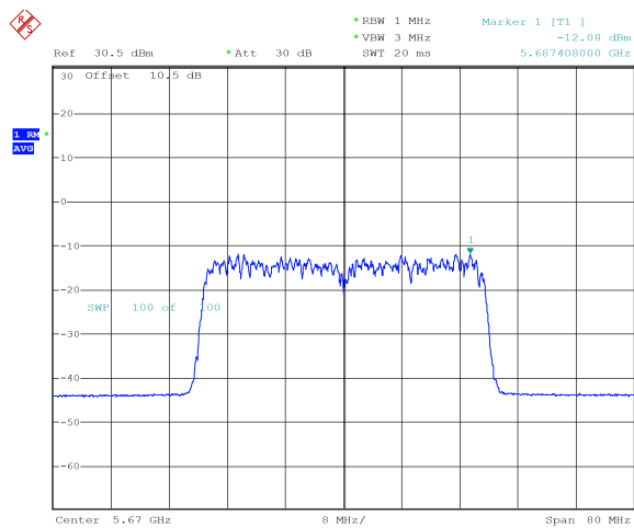
ax40_5670MHz_RU_484/65_Chain 0 -12.08 dBm
