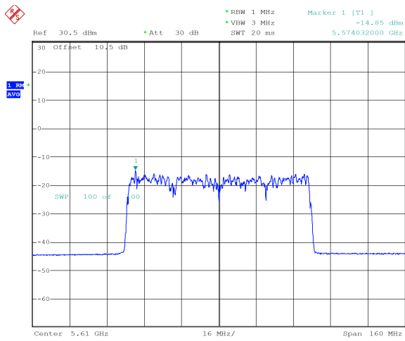
ax80_5610MHz_RU_996/67_Chain 0 -14.85 dBm
