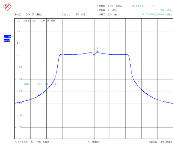
n20_5745MHz_Chain 0 1.98 dBm
