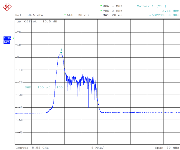
ax40_5550MHz_RU_26/0_Chain 0 2.66 dBm
