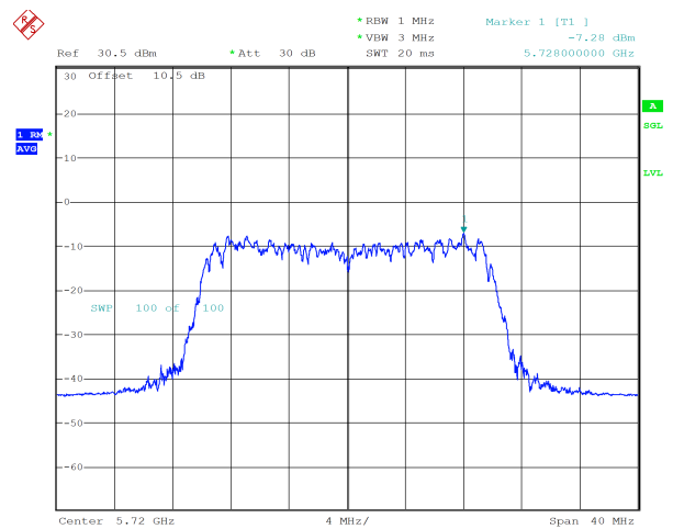
ax20_5720MHz_RU_242/61_Chain 1 -7.28 dBm
