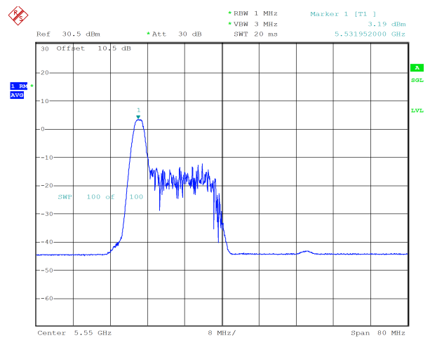
ax40_5550MHz_RU_26/0_Chain 1 3.19 dBm
