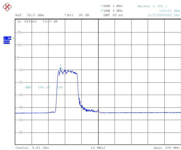
ax80_5610MHz_RU_242/61_Chain 0 -10.03 dBm
