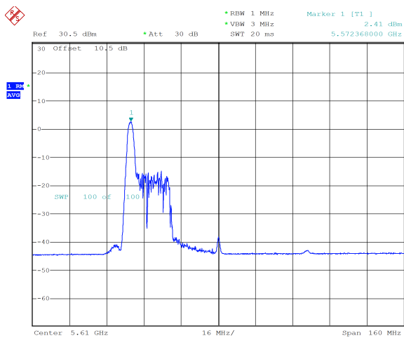
ax80_5610MHz_RU_26/0_Chain 0 2.41 dBm
