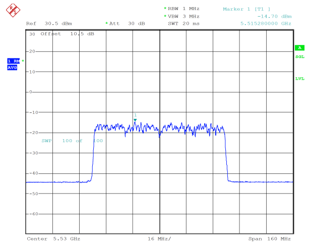
ax80_5530MHz_RU_996/67_Chain 1 -14.70 dBm
