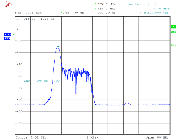
ax40_5510MHz_RU_26/0_Chain 1 3.78 dBm
