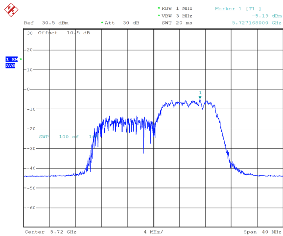
ax20_5720MHz_RU_106/54_Chain 0 -5.19 dBm
