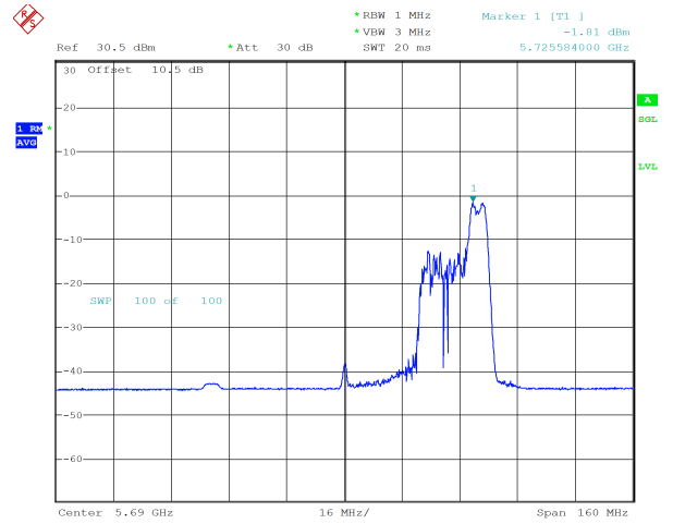
ax80_5690MHz_RU_52/52_Chain 1 -1.81 dBm
