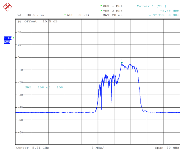
ax40_5710MHz_RU_106/56_Chain 0 -5.45 dBm
