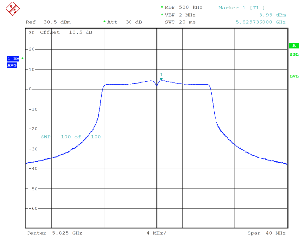
a_5825MHz_Chain 1 3.95 dBm
