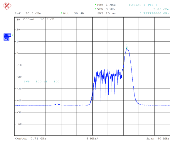
ax40_5710MHz_RU_26/17_Chain 0 3.06 dBm
