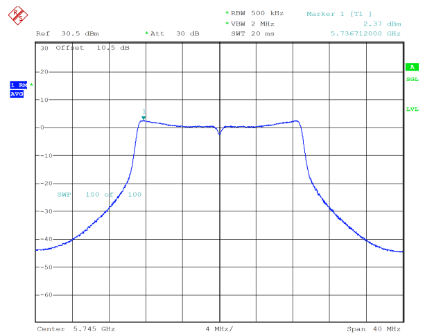
n20_5745MHz_Chain 1 2.37 dBm
