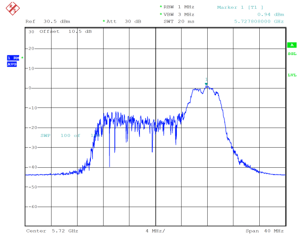
ax20_5720MHz_RU_52/40_Chain 1 0.94 dBm
