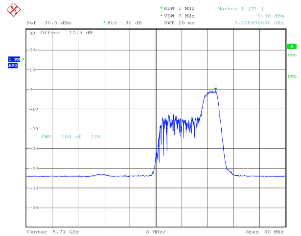
ax40_5710MHz_RU_52/44_Chain 1 -0.96 dBm
