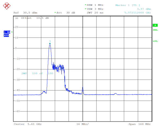
ax80_5610MHz_RU_26/0_Chain 1 3.37 dBm
