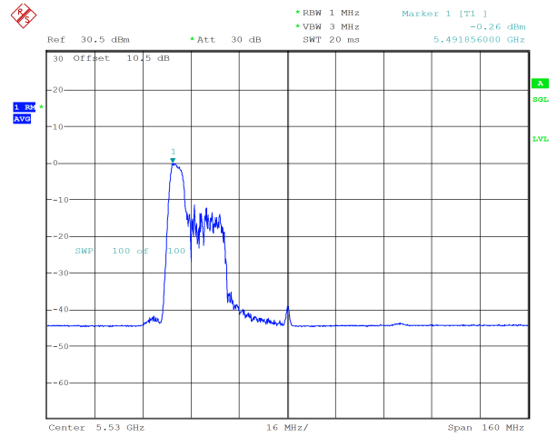
ax80_5530MHz_RU_52/37_Chain 1 -0.26 dBm
