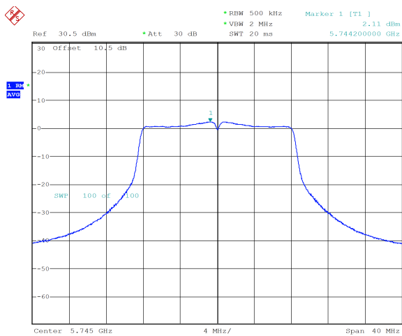
a_5745MHz_Chain 0 2.11 dBm
