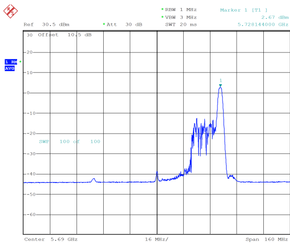
ax80_5690MHz_RU_26/36_Chain 0 2.67 dBm
