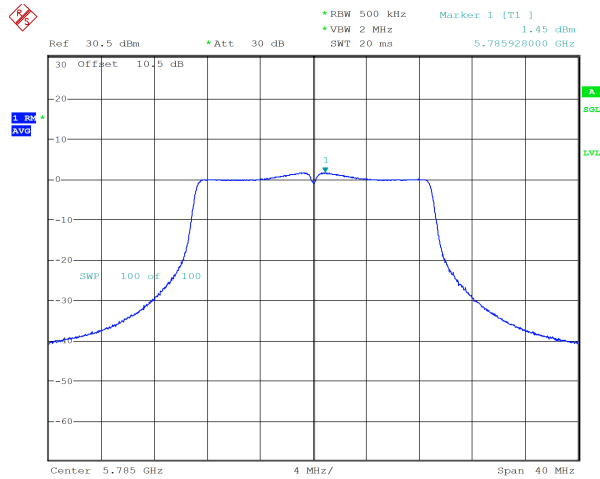
n20_5785MHz_Chain 0 1.45 dBm
