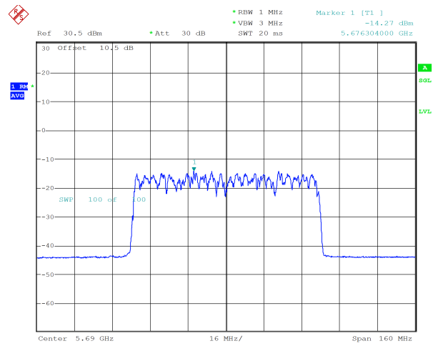
ax80_5690MHz_RU_996/67_Chain 1 -14.27 dBm
