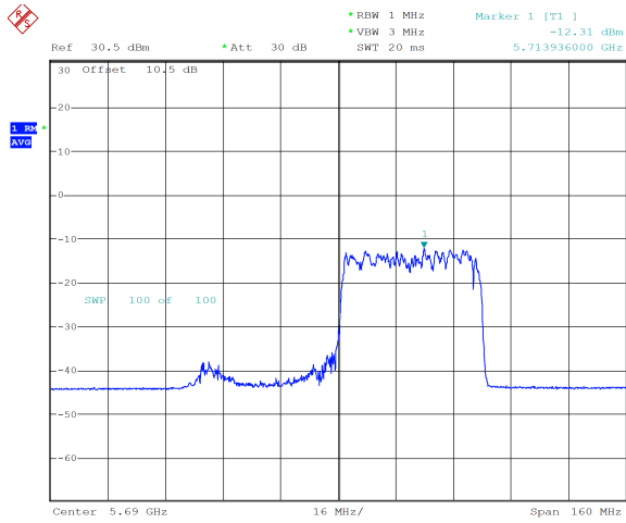
ax80_5690MHz_RU_484/66_Chain 0 -12.31 dBm
