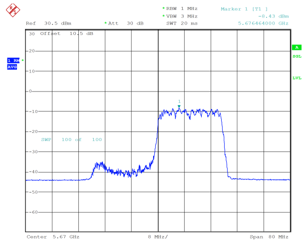
ax40_5670MHz_RU_242/62_Chain 1 -8.43 dBm
