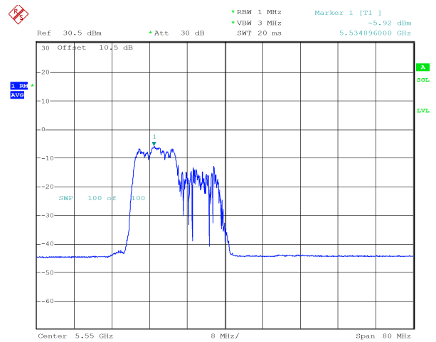
ax40_5550MHz_RU_106/53_Chain 1 -5.92 dBm
