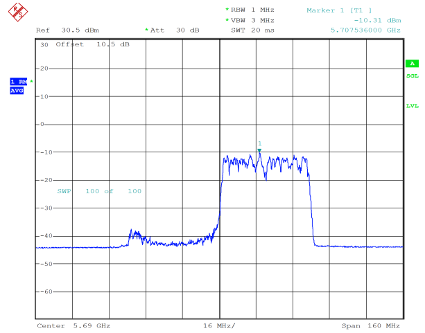
ax80_5690MHz_RU_484/66_Chain 1 -10.31 dBm
