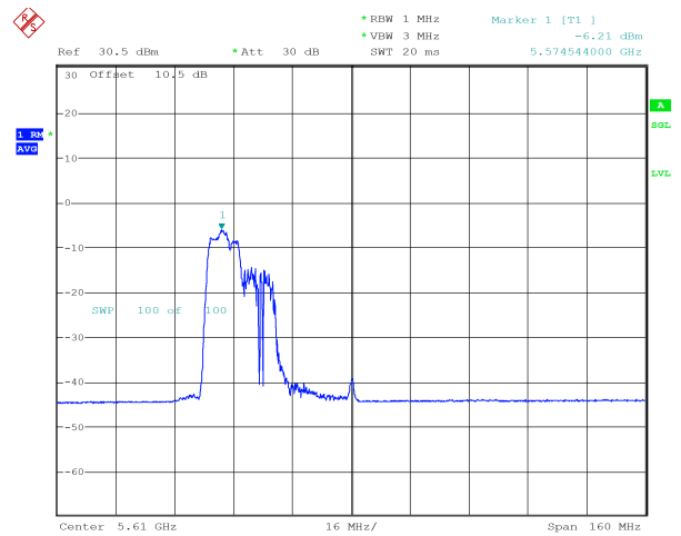
ax80_5610MHz_RU_106/53_Chain 1 -6.21 dBm
