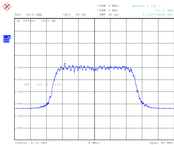
ax20_5720MHz_RU_242/61_Chain 0 -8.11 dBm
