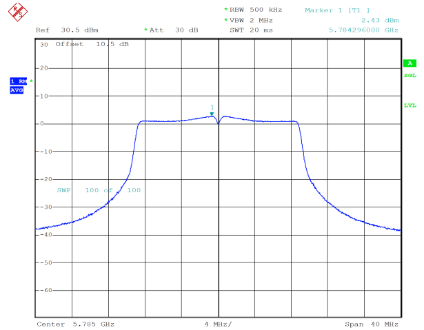
n20_5785MHz_Chain 1 2.43 dBm
