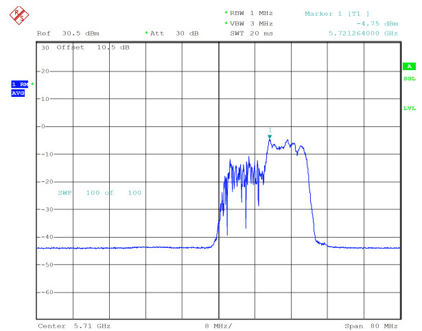
ax40_5710MHz_RU_106/56_Chain 1 -4.75 dBm
