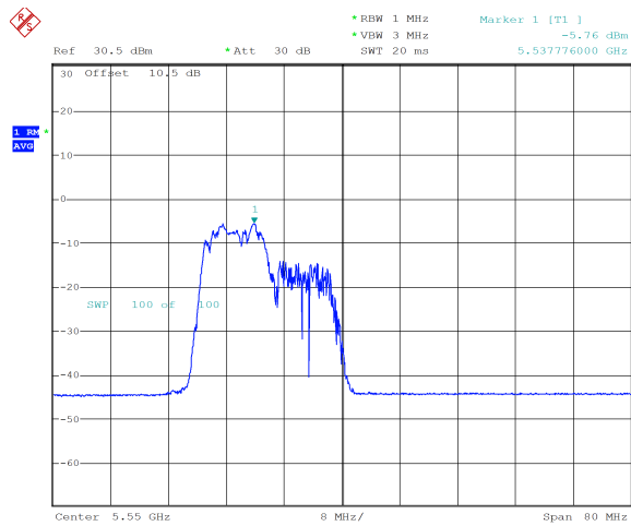
ax40_5550MHz_RU_106/53_Chain 0 -5.76 dBm
