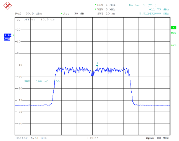
ax40_5510MHz_RU_484/65_Chain 1 -11.73 dBm
