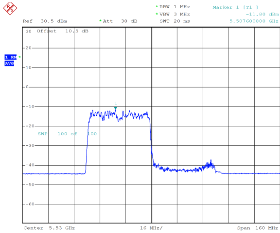
ax80_5530MHz_RU_484/65_Chain 0 -11.80 dBm
