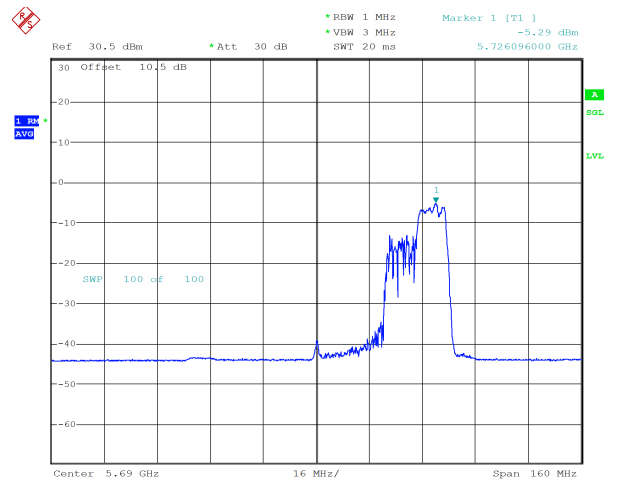
ax80_5690MHz_RU_106/60_Chain 1 -5.29 dBm
