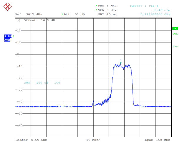
ax80_5690MHz_RU_242/64_Chain 1 -8.49 dBm
