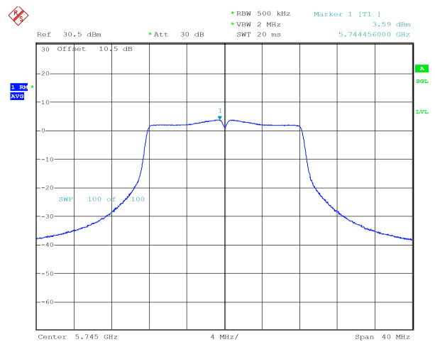
a_5745MHz_Chain 1 3.59 dBm
