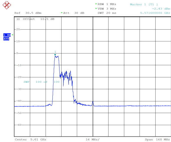
ax80_5610MHz_RU_52/37_Chain 0 -2.43 dBm
