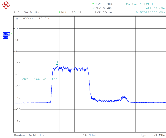
ax80_5610MHz_RU_484/65_Chain 0 -12.56 dBm
