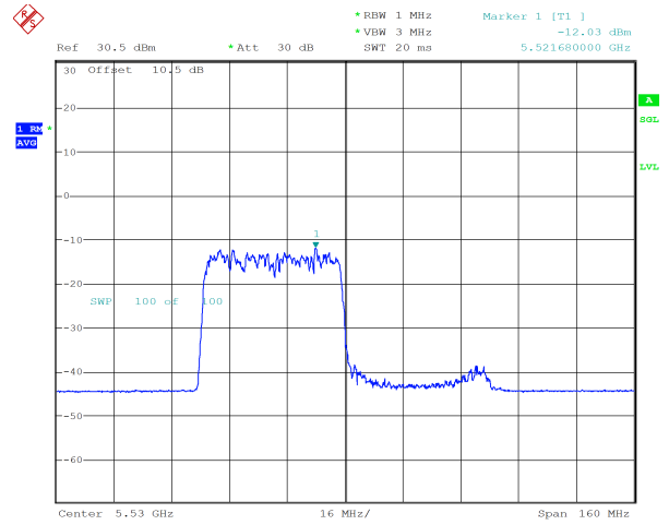
ax80_5530MHz_RU_484/65_Chain 1 -12.03 dBm
