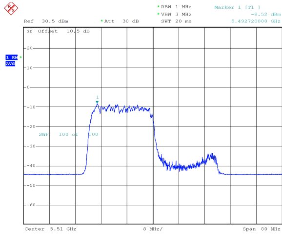
ax40_5510MHz_RU_242/61_Chain 0 -8.52 dBm
