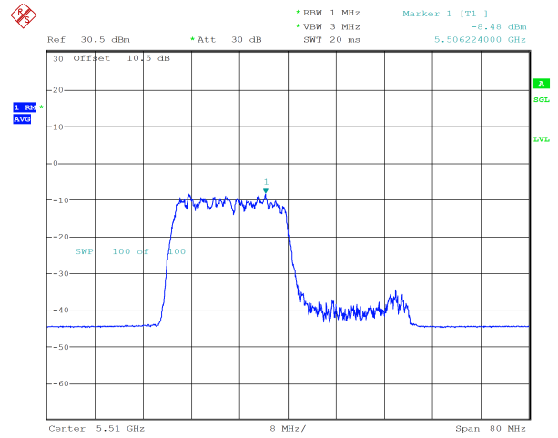
ax40_5510MHz_RU_242/61_Chain 1 -8.48 dBm
