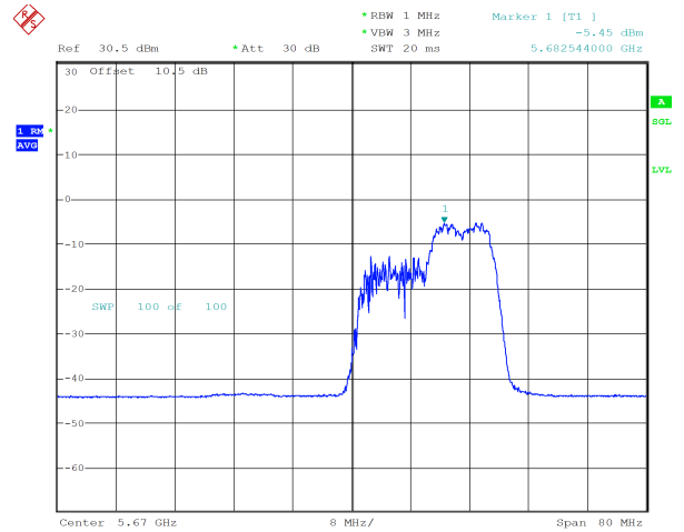
ax40_5670MHz_RU_106/56_Chain 1 -5.45 dBm
