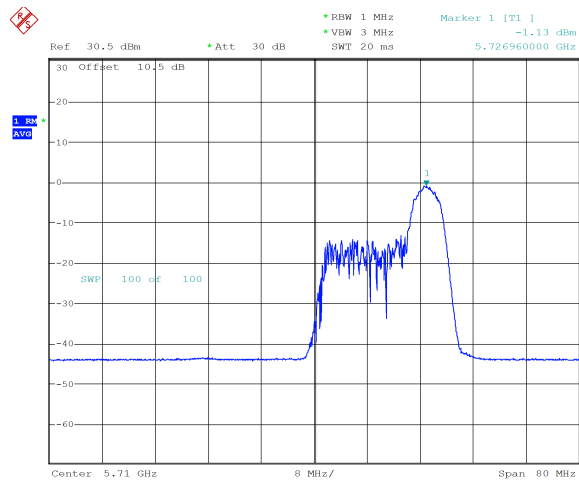
ax40_5710MHz_RU_52/44_Chain 0 -1.13 dBm
