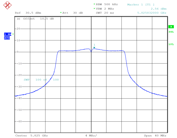
n20_5825MHz_Chain 1 2.56 dBm
