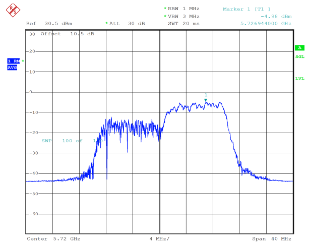
ax20_5720MHz_RU_106/54_Chain 1 -4.98 dBm
