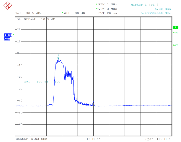
ax80_5530MHz_RU_106/53_Chain 1 -5.30 dBm
