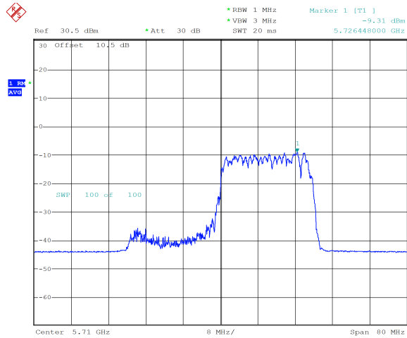
ax40_5710MHz_RU_242/62_Chain 0 -9.31 dBm
