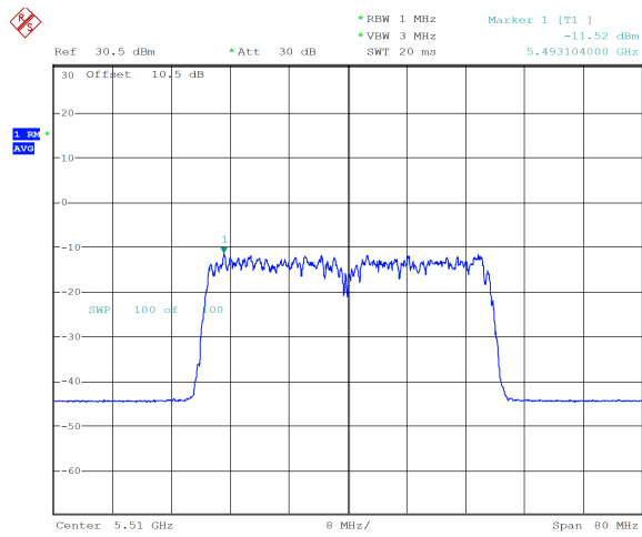
ax40_5510MHz_RU_484/65_Chain 0 -11.52 dBm
