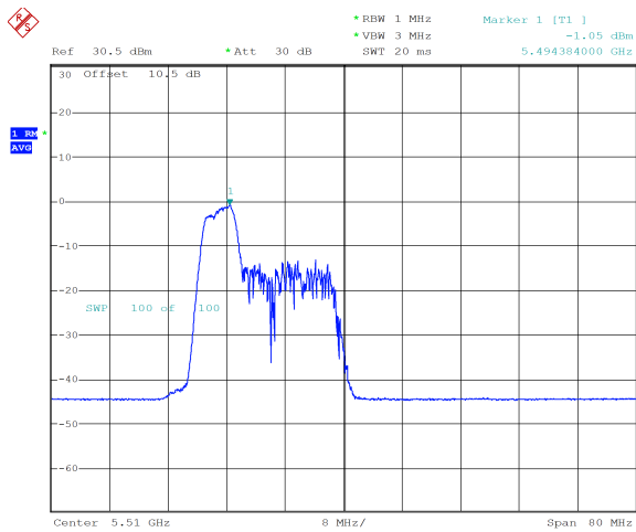
ax40_5510MHz_RU_52/37_Chain 0 -1.05 dBm
