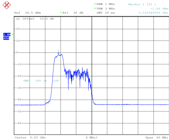
ax40_5550MHz_RU_52/37_Chain 0 -1.66 dBm
