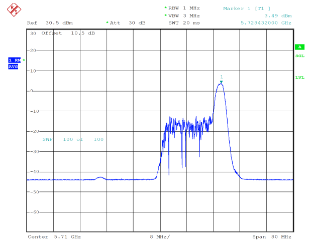
ax40_5710MHz_RU_26/17_Chain 1 3.49 dBm
