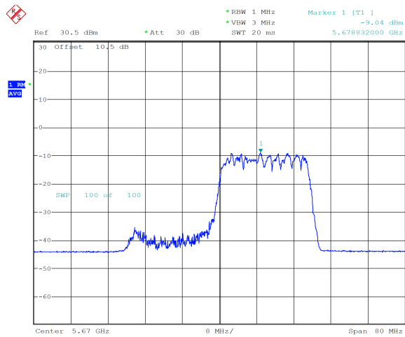
ax40_5670MHz_RU_242/62_Chain 0 -9.04 dBm
