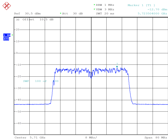
ax40_5710MHz_RU_484/65_Chain 0 -12.70 dBm
