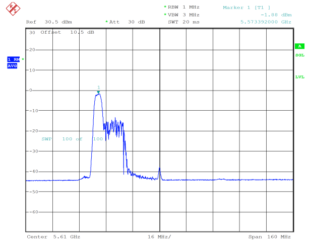
ax80_5610MHz_RU_52/37_Chain 1 -1.88 dBm
