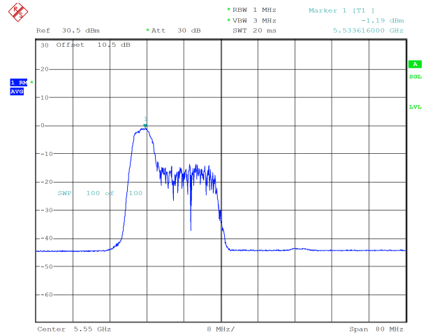
ax40_5550MHz_RU_52/37_Chain 1 -1.19 dBm
