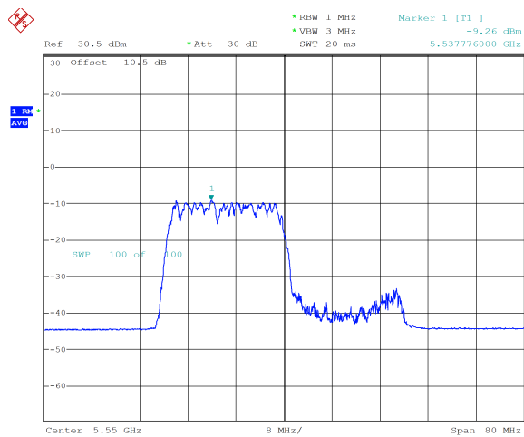
ax40_5550MHz_RU_242/61_Chain 0 -9.26 dBm
