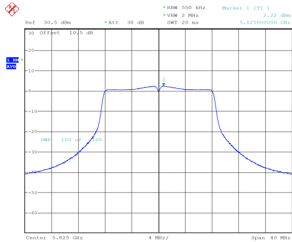
a_5825MHz_Chain 0 2.22 dBm
