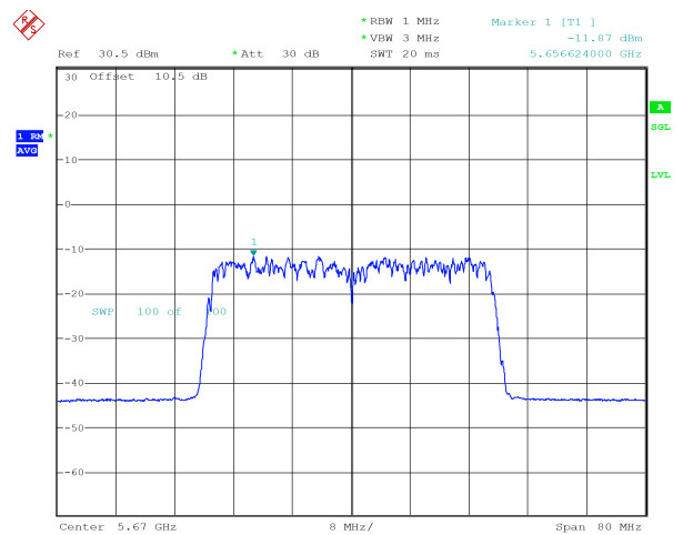
ax40_5670MHz_RU_484/65_Chain 1 -11.87 dBm
