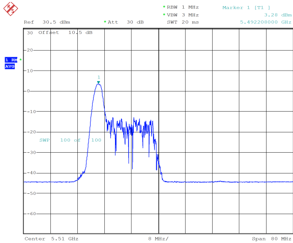
ax40_5510MHz_RU_26/0_Chain 0 3.28 dBm
