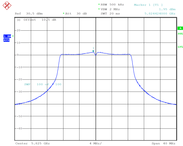
n20_5825MHz_Chain 0 1.95 dBm
