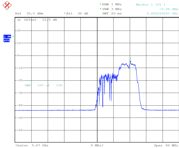
ax40_5670MHz_RU_106/56_Chain 0 -5.96 dBm
