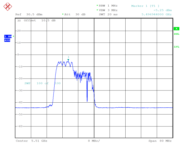
ax40_5510MHz_RU_106/53_Chain 1 -5.25 dBm
