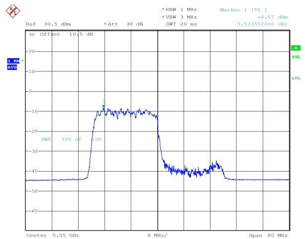
ax40_5550MHz_RU_242/61_Chain 1 -8.57 dBm
