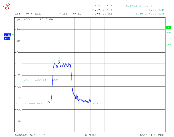
ax80_5530MHz_RU_242/61_Chain 1 -8.70 dBm
