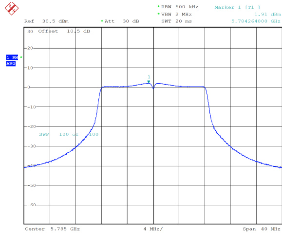
a_5785MHz_Chain 0 1.91 dBm
