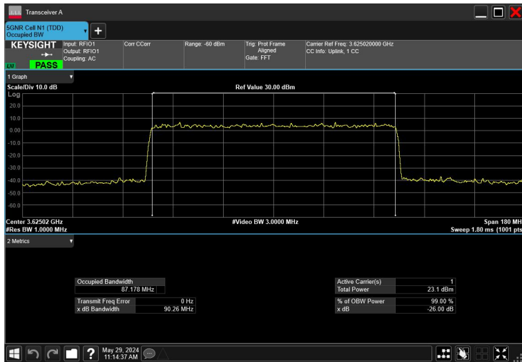
90MHz_30kHz_3625MHz_CP-OFDM 16QAM_RB245@0
