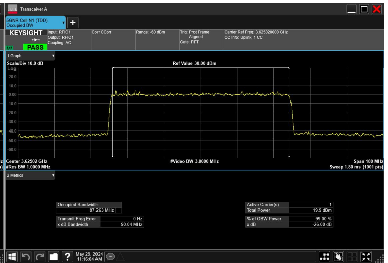
90MHz_30kHz_3625MHz_CP-OFDM 256QAM_RB245@0
