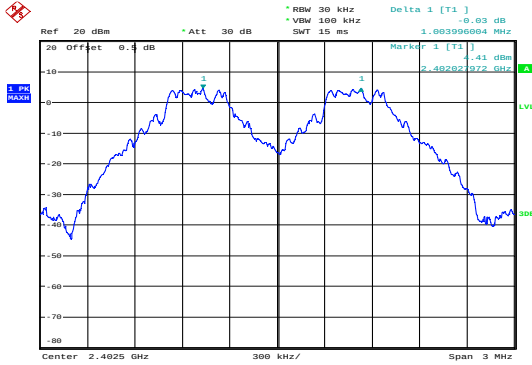
GFSK_Low 1.004MHz
