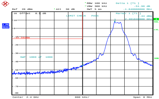
GFSK_Low
