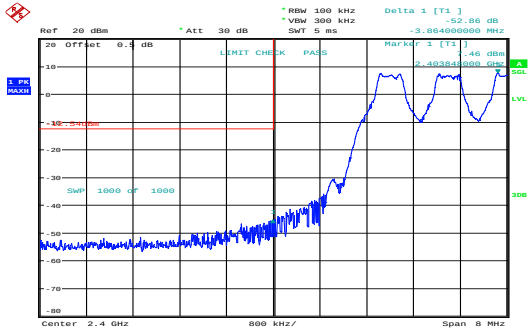
GFSK_Hopping_Lower
