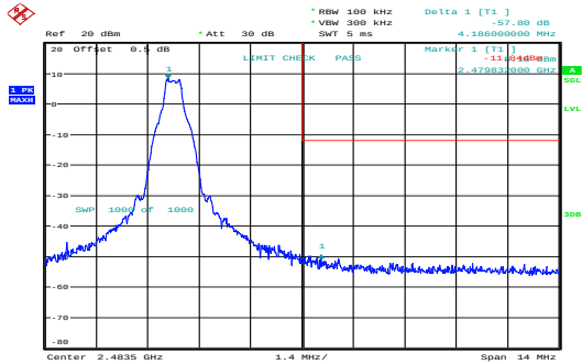
GFSK_High
