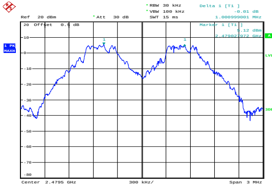
GFSK_High 1.001MHz
