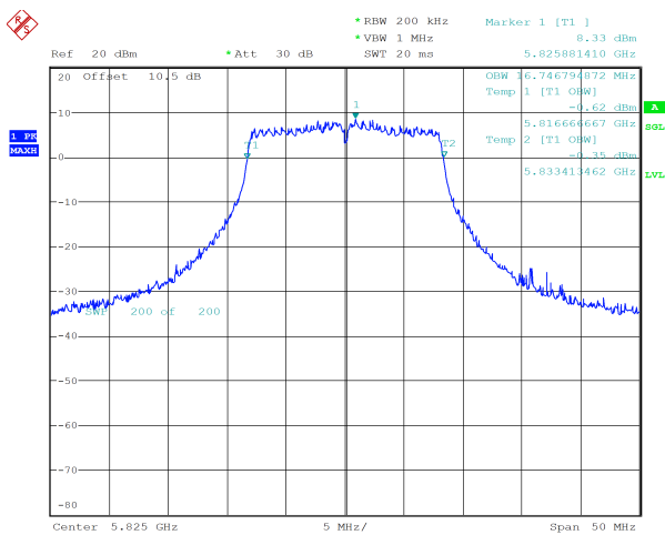
a_5825MHz_Chain 1 16.747 MHz
