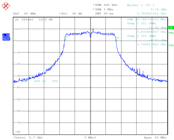
a_5700MHz_Chain 1 16.747 MHz
