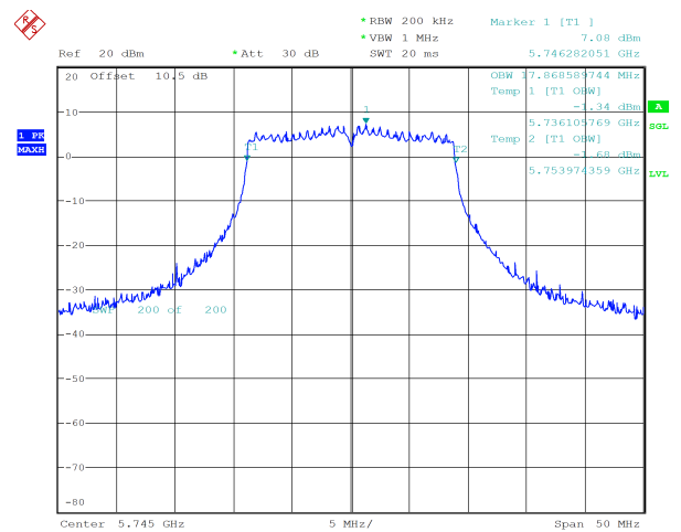
n20_5745MHz_Chain 1 17.869 MHz
