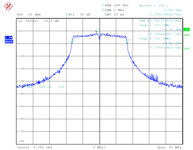
a_5785MHz_Chain 1 16.747 MHz
