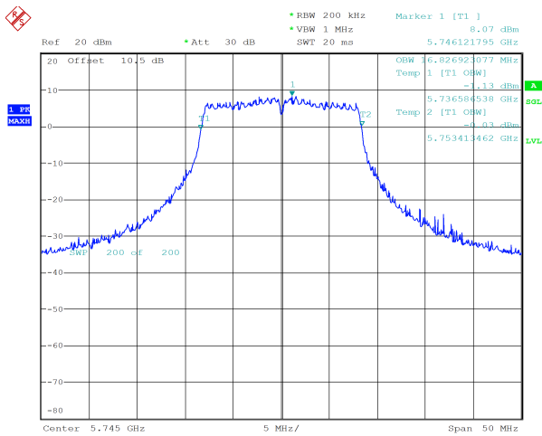
a_5745MHz_Chain 1 16.827 MHz
