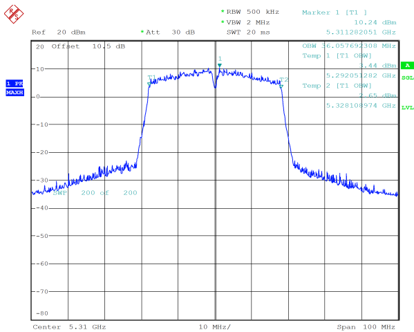
n40_5310MHz_Chain 1 36.058 MHz
