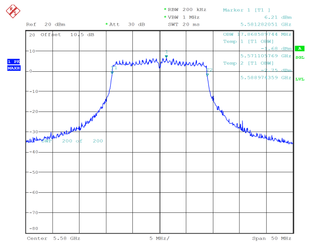
n20_5580MHz_Chain 1 17.869 MHz
