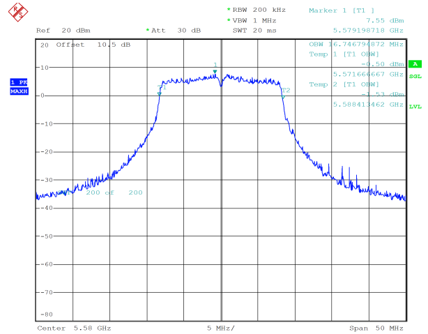
a_5580MHz_Chain 1 16.747 MHz
