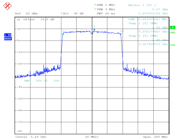
ac80_5290MHz_Chain 1 75.641 MHz
