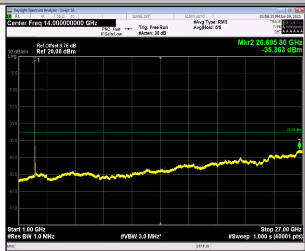
7-7-20MHz-20MHz-16QAM-16QAM-20850-21048-1RB#0-0 RB#0-1000~27000MHz-PASS
