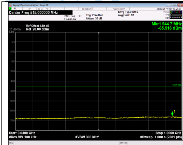
7-7-20MHz-20MHz-16QAM-16QAM-20850-21048-1RB#9 9-ORB#0-30~1000MHz-PASS
