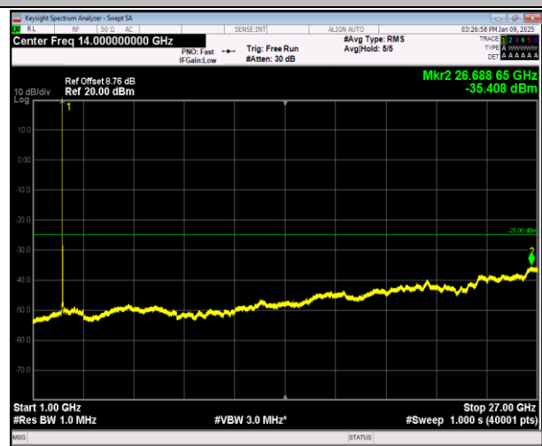
7-7-10MHz-20MHz-QPSK-QPSK-21006-21150-1RB#49-0R B#0-1000~27000MHz-PASS
