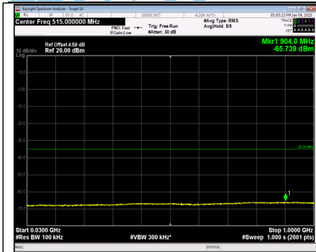
7-7-20MHz-10MHz-16QAM-16QAM-21051-21195-1RB#0 -ORB#0-30~1000MHz-PASS
