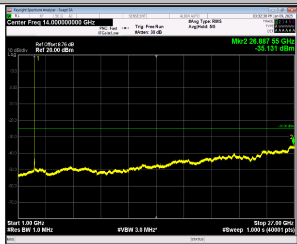
7-7-10MHz-20MHz-16QAM-16QAM-21206-21350-1RB#49- 0RB#0-1000~27000MHz-PASS
