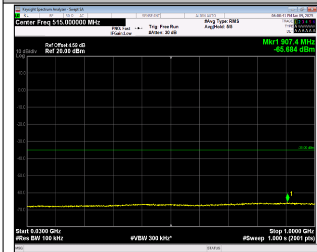
7-7-20MHz-20MHz-16QAM-16QAM-20850-21048-1RB#0 -1RB#99-30~1000MHz-PASS
