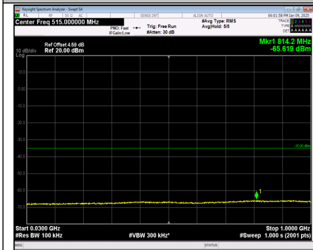
7-7-20MHz-20MHz-16QAM-16QAM-20850-21048-100RB #0-100RB#0-30~1000MHz-PASS
