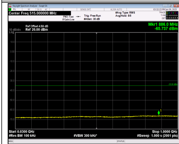
7-7-10MHz-20MHz-16QAM-16QAM-21206-21350-1RB#4 9-0RB#0-30~1000MHz-PASS
