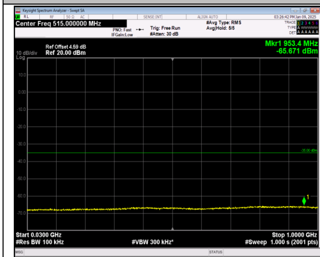
7-7-10MHz-20MHz-QPSK-QPSK-21006-21150-1RB#49-0 RB#0-30~1000MHz-PASS
