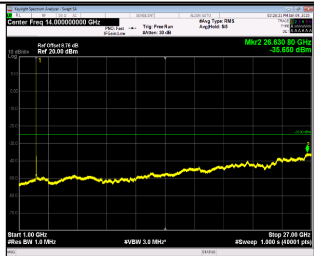
7-7-10MHz-20MHz-16QAM-16QAM-21006-21150-1RB#0-0 RB#0-1000~27000MHz-PASS
