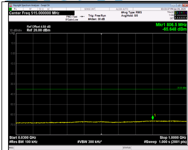
7-7-10MHz-20MHz-16QAM-16QAM-21206-21350-1RB#0 -1RB#99-30~1000MHz-PASS
