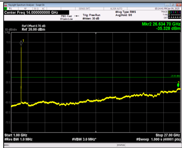
7-7-20MHz-10MHz-16QAM-16QAM-21251-21395-100RB#0 -50RB#0-1000~27000MHz-PASS
