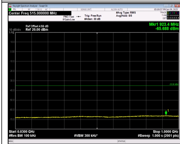
7-7-20MHz-10MHz-QPSK-QPSK-21251-21395-1RB#0-0 RB#0-30~1000MHz-PASS
