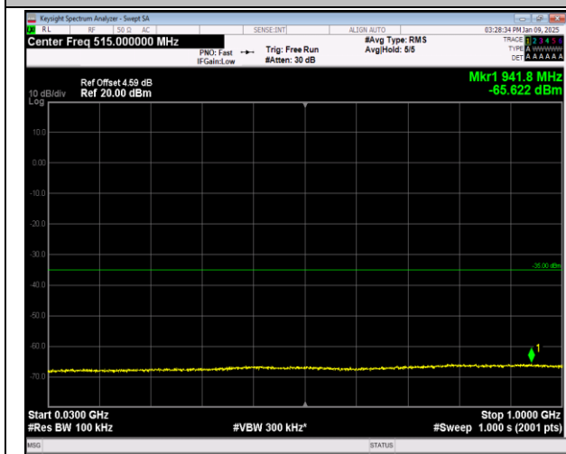
7-7-10MHz-20MHz-16QAM-16QAM-21006-21150-1RB#0 -1RB#99-30~1000MHz-PASS
