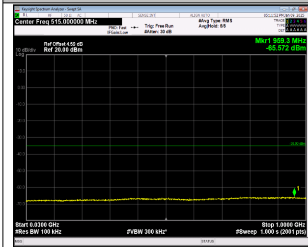
7-7-20MHz-10MHz-16QAM-16QAM-21251-21395-1RB#9 9-0RB#0-30~1000MHz-PASS
