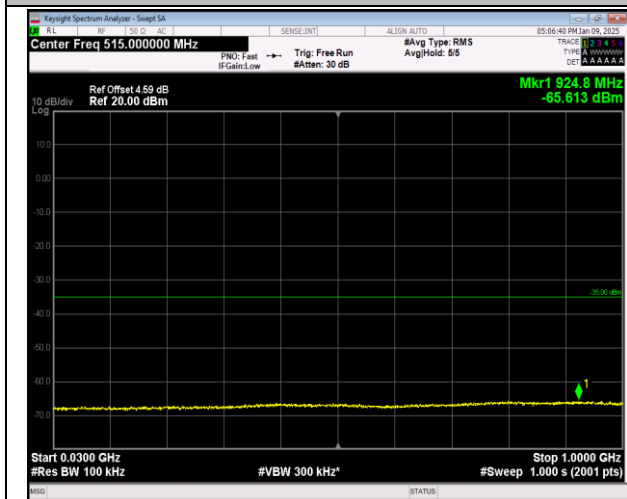
7-7-20MHz-10MHz-16QAM-16QAM-21051-21195-1RB#9 9-ORB#0-30~1000MHz-PASS
