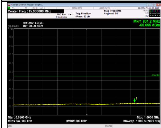
7-7-10MHz-20MHz-16QAM-16QAM-21206-21350-50RB# 0-100RB#0-30~1000MHz-PASS
