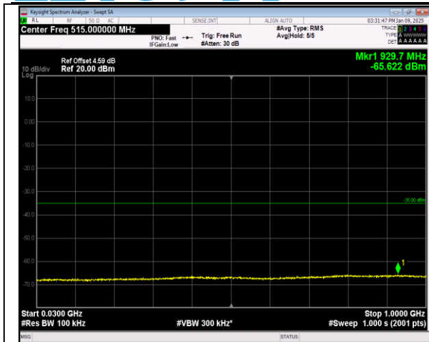
7-7-10MHz-20MHz-QPSK-QPSK-21206-21350-1RB#49-0RB#0-30~1000MHz-PASS
