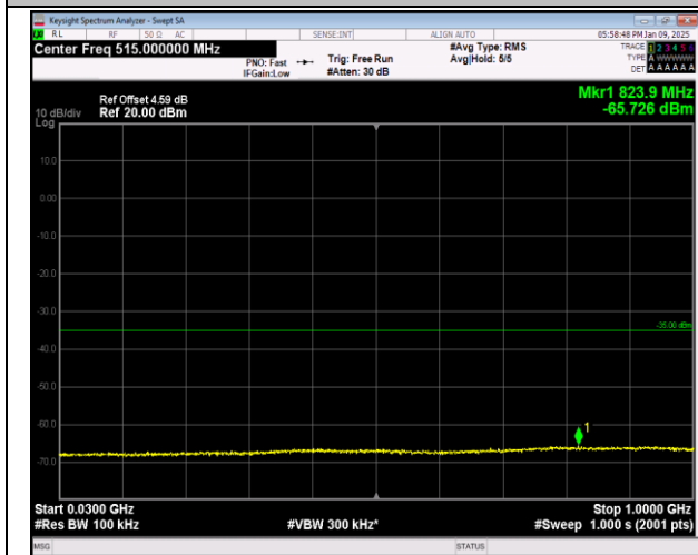
7-7-20MHz-20MHz-QPSK-QPSK-20850-21048-1RB#99-99 ORB#0-30~1000MHz-PASS
