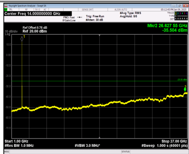
7-7-20MHz-10MHz-QPSK-QPSK-21251-21395-1RB#0-1RB #49-1000~27000MHz-PASS
