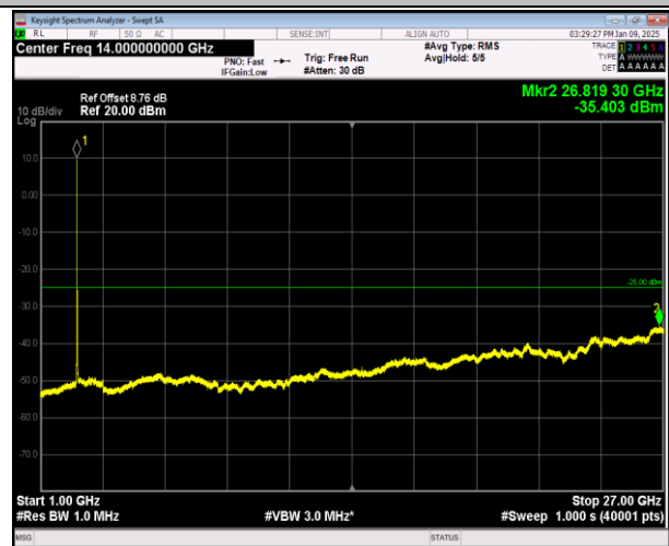
7-7-10MHz-20MHz-QPSK-QPSK-21006-21150-50RB#0-10 ORB#0-1000~27000MHz-PASS
