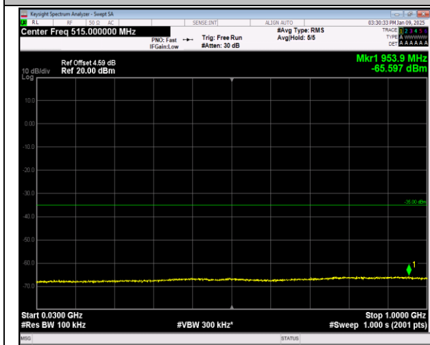
7-7-10MHz-20MHz-QPSK-QPSK-21206-21350-1RB#0-0 RB#0-30~1000MHz-PASS
