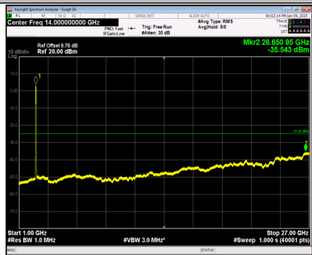
7-7-20MHz-20MHz-16QAM-16QAM-20850-21048-100RB#0 -100RB#0-1000~27000MHz-PASS
