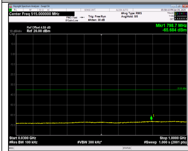
7-7-20MHz-20MHz-16QAM-16QAM-20850-21048-1RB#0 -0RB#0-30~1000MHz-PASS
