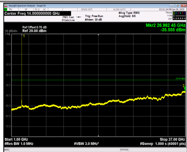
7-7-10MHz-20MHz-16QAM-16QAM-21206-21350-1RB#0-0RB#0-1000~27000MHz-PASS
