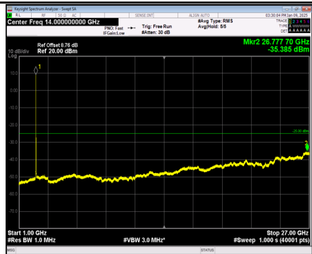
7-7-10MHz-20MHz-16QAM-16QAM-21006-21150-50RB#0- 100RB#0-1000~27000MHz-PASS
