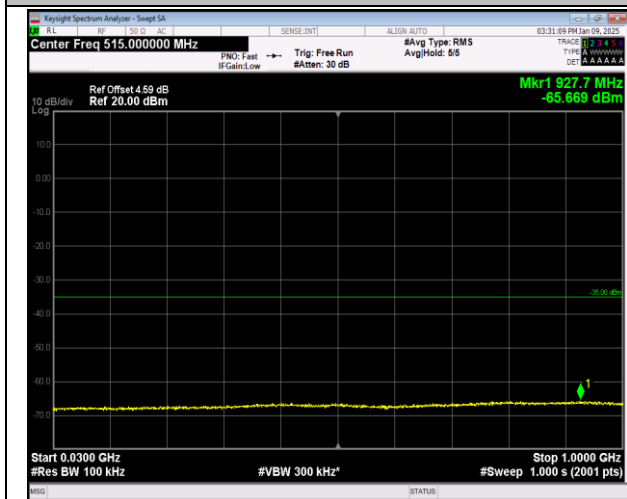
7-7-10MHz-20MHz-16QAM-16QAM-21206-21350-1RB#0-0RB#0-30~1000MHz-PASS
