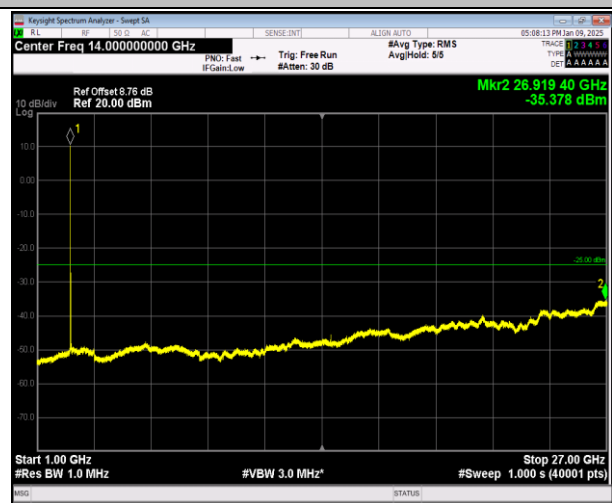
7-7-20MHz-10MHz-16QAM-16QAM-21051-21195-1RB#0-1 RB#49-1000~27000MHz-PASS
