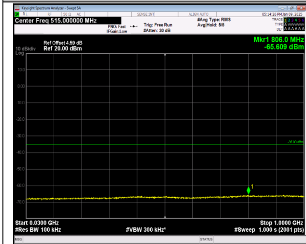
7-7-20MHz-10MHz-16QAM-16QAM-21251-21395-100RB #0-50RB#0-30~1000MHz-PASS
