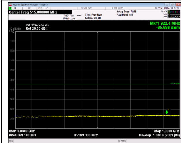
7-7-20MHz-20MHz-QPSK-QPSK-21001-21199-1RB#0-0 RB#0-30~1000MHz-PASS
