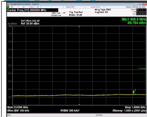
7-7-20MHz-10MHz-16QAM-16QAM-21051-21195-100RB #0-50RB#0-30~1000MHz-PASS
