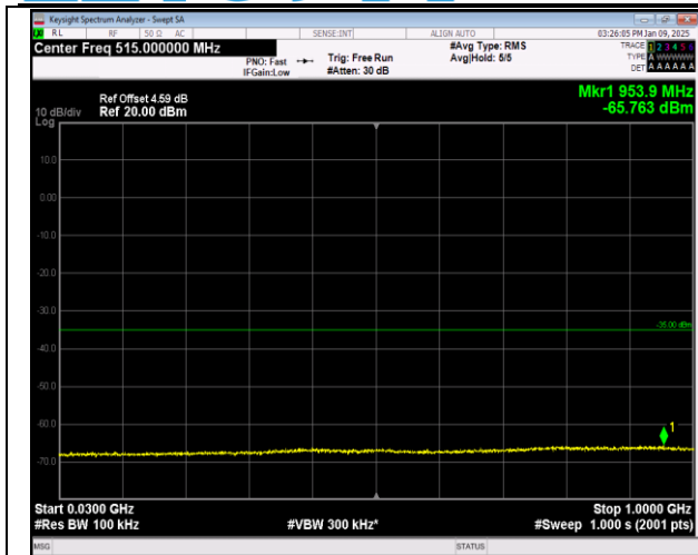
7-7-10MHz-20MHz-16QAM-16QAM-21006-21150-1RB#0 -ORB#0-30~1000MHz-PASS
