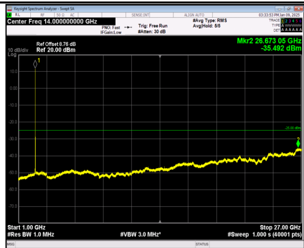
7-7-10MHz-20MHz-16QAM-16QAM-21206-21350-1RB#0-1 RB#99-1000~27000MHz-PASS
