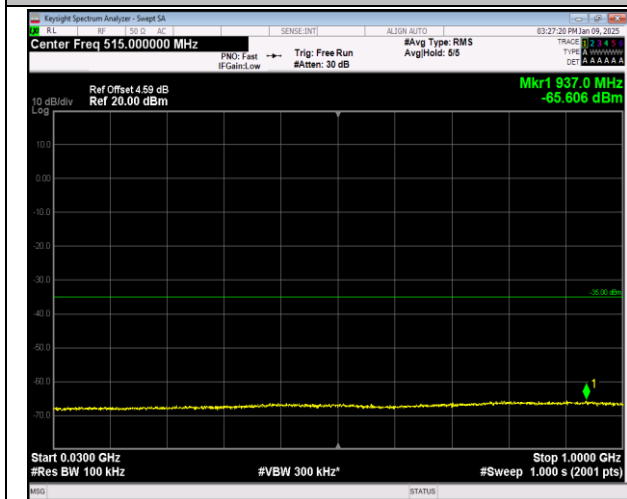
7-7-10MHz-20MHz-16QAM-16QAM-21006-21150-1RB#4 9-ORB#0-30~1000MHz-PASS
