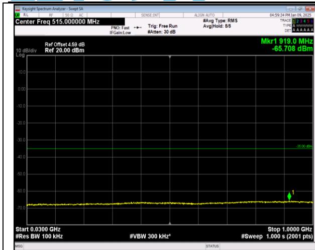
7-7-20MHz-10MHz-QPSK-QPSK-20850-20994-1RB#0-0 RB#0-30~1000MHz-PASS
