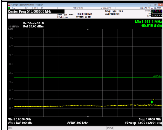
7-7-20MHz-10MHz-QPSK-QPSK-20850-20994-1RB#99-99 ORB#0-30~1000MHz-PASS
