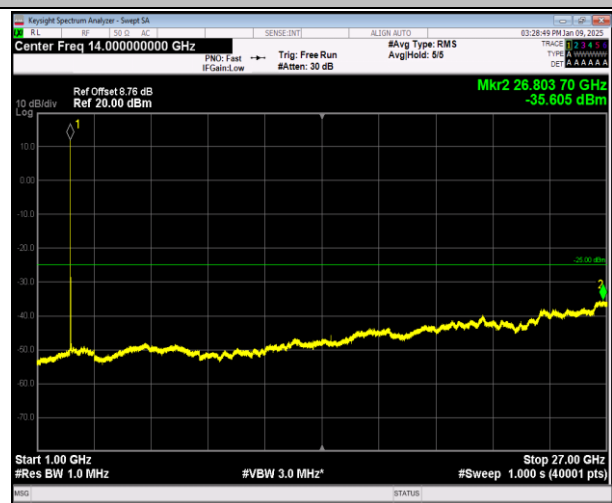
7-7-10MHz-20MHz-16QAM-16QAM-21006-21150-1RB#0-1 RB#99-1000~27000MHz-PASS
