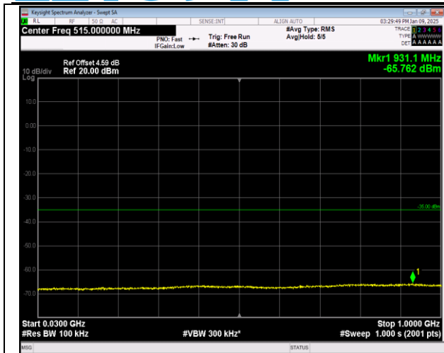
7-7-10MHz-20MHz-16QAM-16QAM-21006-21150-50RB# 0-100RB#0-30~1000MHz-PASS
