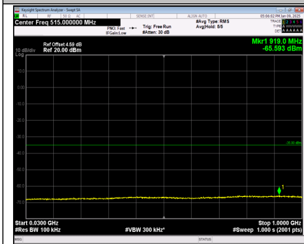
7-7-20MHz-10MHz-QPSK-QPSK-21051-21195-1RB#99-0 RB#0-30~1000MHz-PASS
