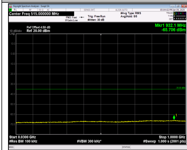
7-7-20MHz-10MHz-16QAM-16QAM-20850-20994-100RB #0-50RB#0-30~1000MHz-PASS
