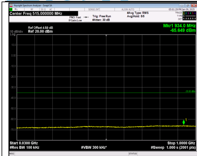
7-7-20MHz-10MHz-16QAM-16QAM-20850-20994-1RB#9 9-0RB#0-30~1000MHz-PASS
