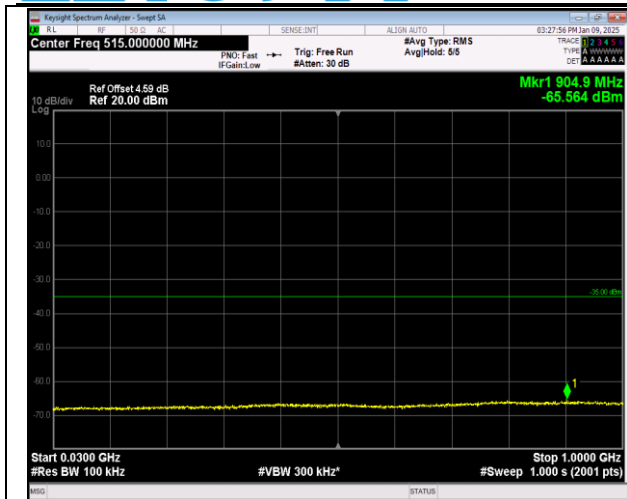
7-7-10MHz-20MHz-QPSK-QPSK-21006-21150-1RB#0-1 RB#99-30~1000MHz-PASS
