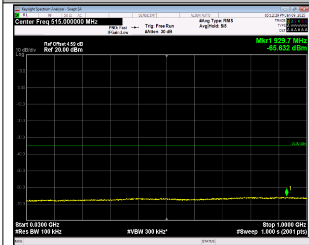
7-7-20MHz-10MHz-QPSK-QPSK-21251-21395-1RB#0-1 RB#49-30~1000MHz-PASS
