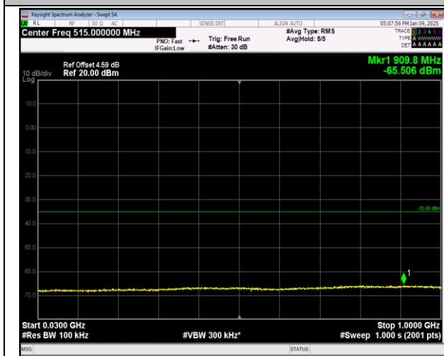
7-7-20MHz-10MHz-16QAM-16QAM-21051-21195-1RB#0 -1RB#49-30~1000MHz-PASS
