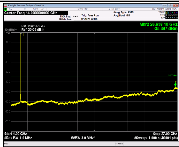
7-7-20MHz-10MHz-16QAM-16QAM-21251-21395-1RB#99- 0RB#0-1000~27000MHz-PASS
