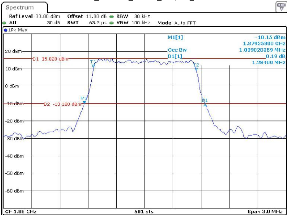
Band 2_1.4 MHz_Middle_16QAM_RB6#0
