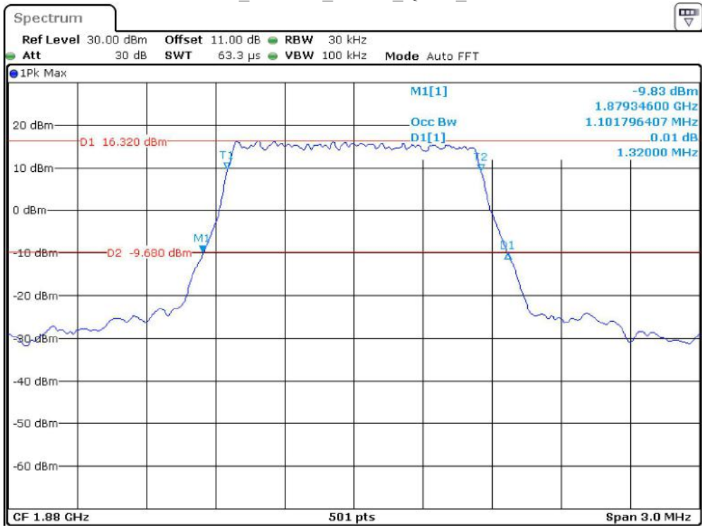
Band 2_1.4 MHz_Middle_QPSK_RB6#0
