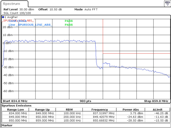
15MHz_15kHz_841.5MHz_DFT-s-OFDM QPSK_RB75@0 -24.63 dBm
