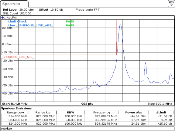
5MHz_15kHz_826.5MHz_DFT-s-OFDM QPSK_RB1@0 -17.94 dBm
