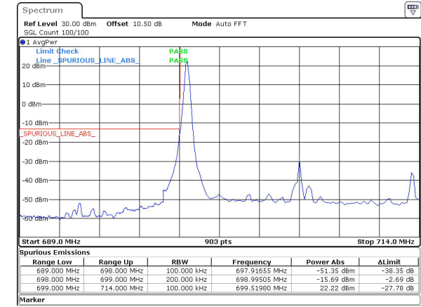
15MHz_15kHz_706.5MHz_DFT-s-OFDM QPSK_RB1@0&-15.69 dBm
