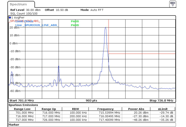
15MHz_15kHz_708.5MHz_DFT-s-OFDM QPSK_RB1@78&-27.30 dBm
