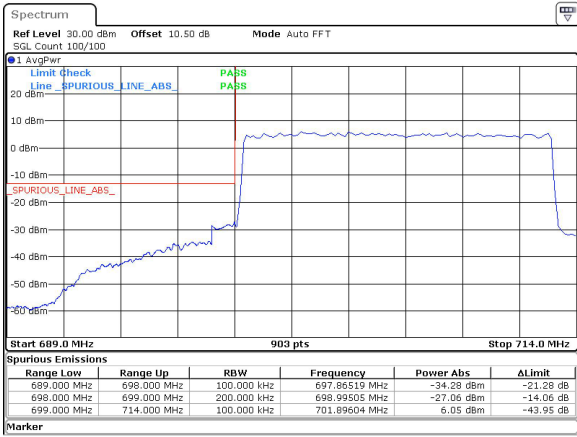
15MHz_15kHz_706.5MHz_DFT-s-OFDM QPSK_RB75@0&-27.06 dBm
