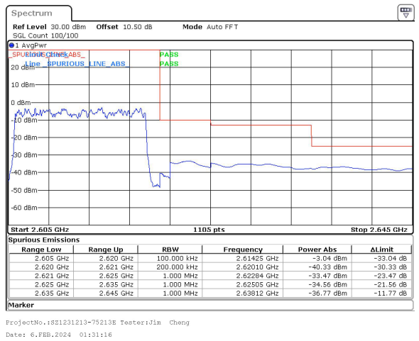
15MHz_30kHz_2612.5MHz_DFT-s-OFDM QPSK_RB36@0&-36.77 dBm
