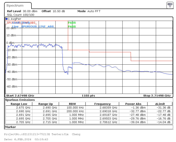
15MHz_30kHz_2682.48MHz_DFT-s-OFDM QPSK_RB36@0&-39.04 dBm
