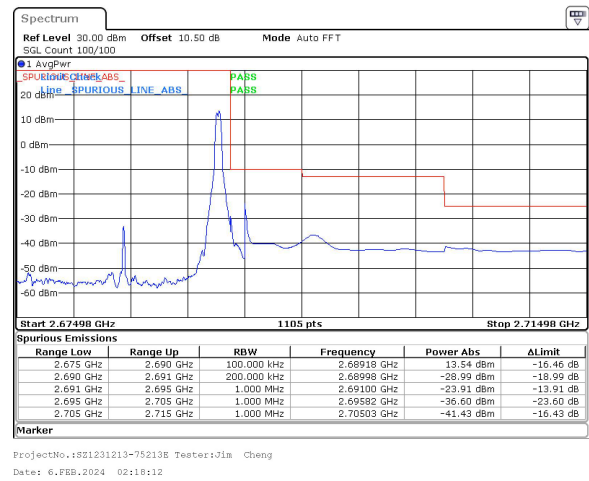
15MHz_30kHz_2682.48MHz_DFT-s-OFDM QPSK_RB1@37&-23.91 dBm
