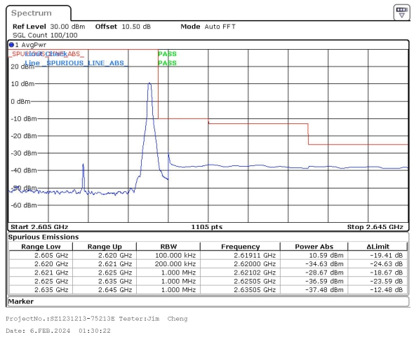
15MHz_30kHz_2612.5MHz_DFT-s-OFDM QPSK_RB1@37&-37.48 dBm
