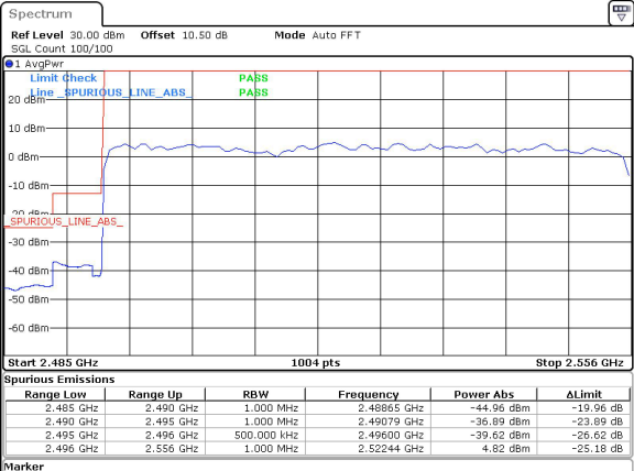
60MHz_30kHz_2526MHz_DFT-s-OFDM QPSK_RB162@0&-44.96 dBm
