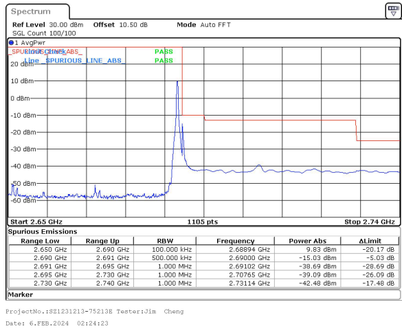
40MHz_30kHz_2670MHz_DFT-s-OFDM QPSK_RB1@105&-15.03 dBm
