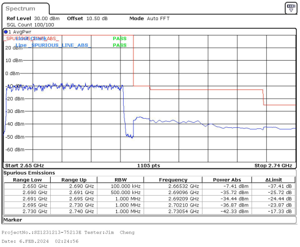
40MHz_30kHz_2670MHz_DFT-s-OFDM QPSK_RB100@0&-42.33 dBm
