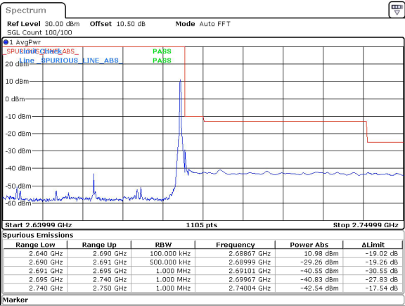
50MHz_30kHz_2664.99MHz_DFT-s-OFDM QPSK_RB1@132&-42.54 dBm
