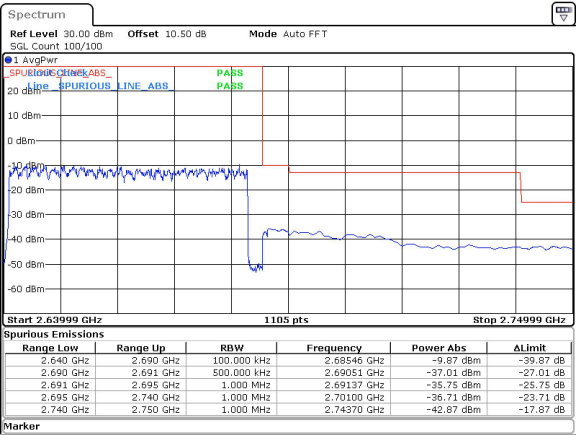
50MHz_30kHz_2664.99MHz_DFT-s-OFDM QPSK_RB128@0&-42.87 dBm
