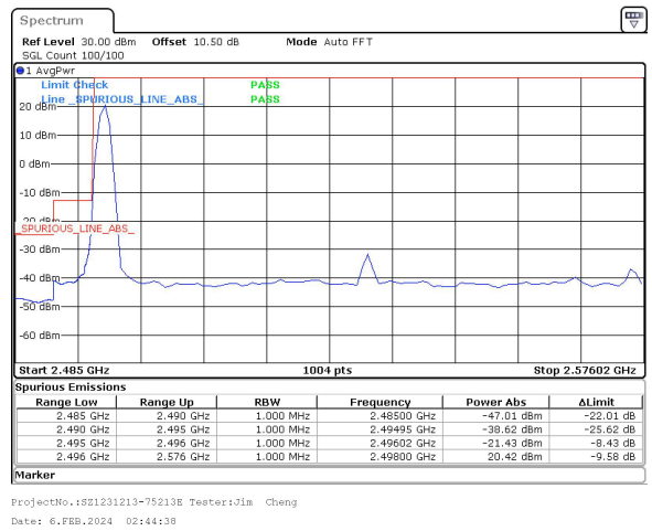
80MHz_30kHz_2536.02MHz_DFT-s-OFDM QPSK_RB1@0&-21.43 dBm
