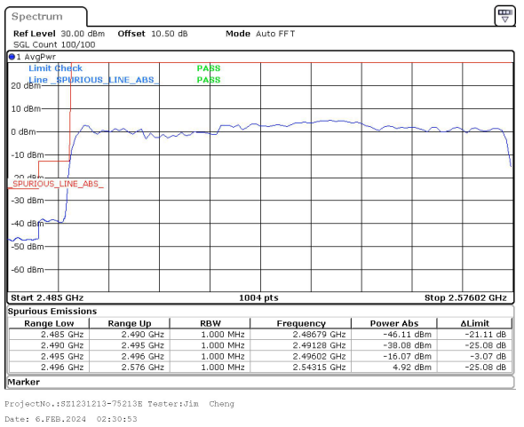
80MHz_30kHz_2536.02MHz_DFT-s-OFDM QPSK_RB216@0&-16.07 dBm
