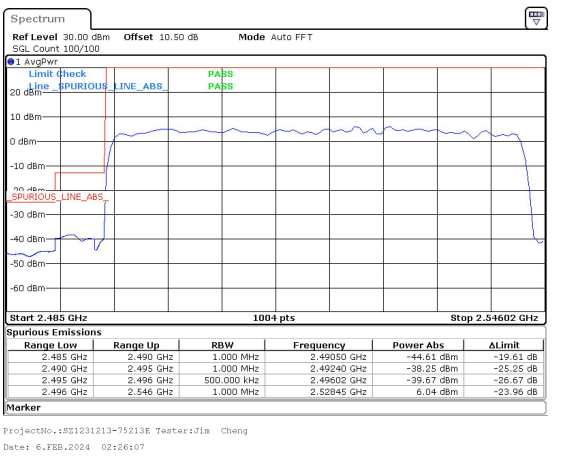
50MHz_30kHz_2521.02MHz_DFT-s-OFDM QPSK_RB128@0&-44.61 dBm
