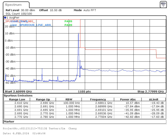
80MHz_30kHz_2649.99MHz_DFT-s-OFDM QPSK_RB1@216&-42.60 dBm
