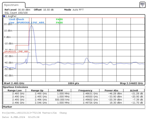
50MHz_30kHz_2521.02MHz_DFT-s-OFDM QPSK_RB1@0&-20.39 dBm
