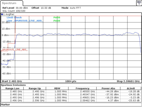
100MHz_30kHz_2546.01MHz_DFT-s-OFDM QPSK_RB270@0&-16.23 dBm
