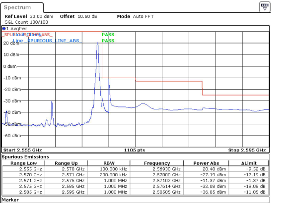
15MHz_15kHz_2562.5MHz_DFT-s-OFDM QPSK_RB1@78&-11.37 dBm
