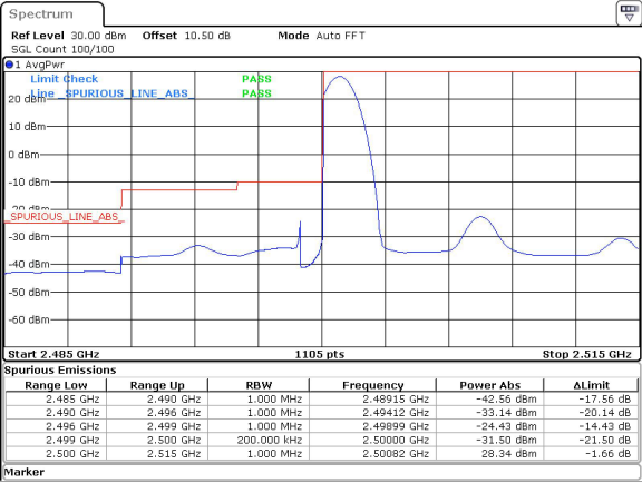
15MHz_15kHz_2507.5MHz_DFT-s-OFDM QPSK_RB1@0&28.34 dBm
