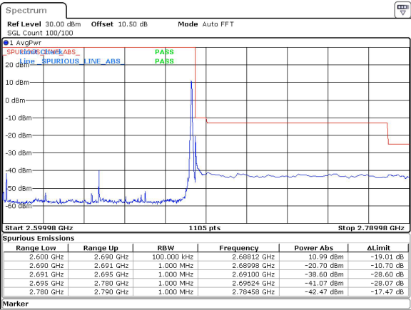
90MHz_30kHz_2644.98MHz_DFT-s-OFDM QPSK_RB1@244&-20.70 dBm
