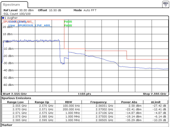
15MHz_15kHz_2562.5MHz_DFT-s-OFDM QPSK_RB75@0&-14.87 dBm
