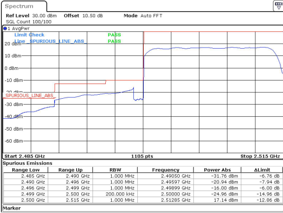
15MHz_15kHz_2507.5MHz_DFT-s-OFDM QPSK_RB75@0&-16.00 dBm
