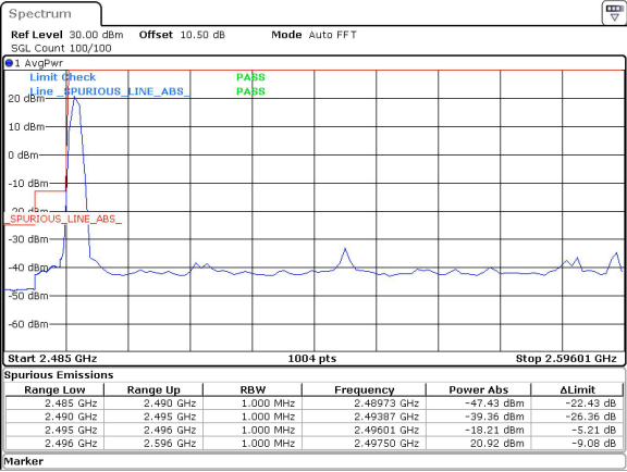
100MHz_30kHz_2546.01MHz_DFT-s-OFDM QPSK_RB1@0&-18.21 dBm
