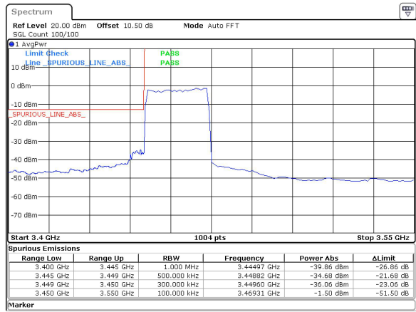
25MHz_30kHz_3462.5MHz_DFT-s-OFDM QPSK_RB64@0&-34.68 dBm
