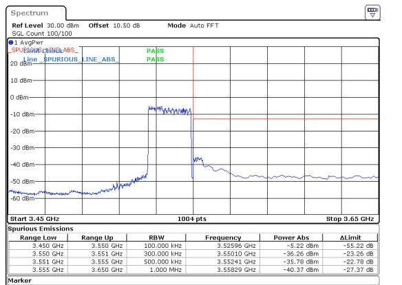
25MHz_30kHz_3537.5MHz_DFT-s-OFDM QPSK_RB64@0&-35.78 dBm
