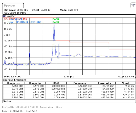
20MHz_15kHz_2560MHz_DFT-s-OFDM QPSK_RB1@105&-15.64 dBm
