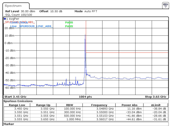
25MHz_30kHz_3537.5MHz_DFT-s-OFDM QPSK_RB1@64&-33.04 dBm
