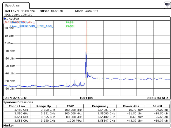
15MHz_30kHz_3542.5MHz_DFT-s-OFDM QPSK_RB1@37&-31.50 dBm
