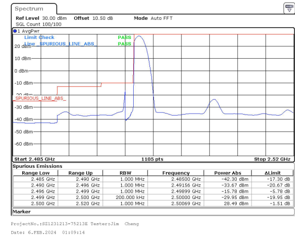
20MHz_15kHz_2510MHz_DFT-s-OFDM QPSK_RB1@0&28.49 dBm
