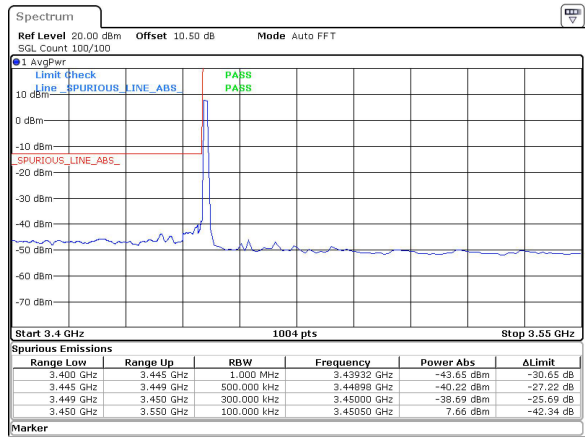
25MHz_30kHz_3462.5MHz_DFT-s-OFDM QPSK_RB1@0&-38.69 dBm
