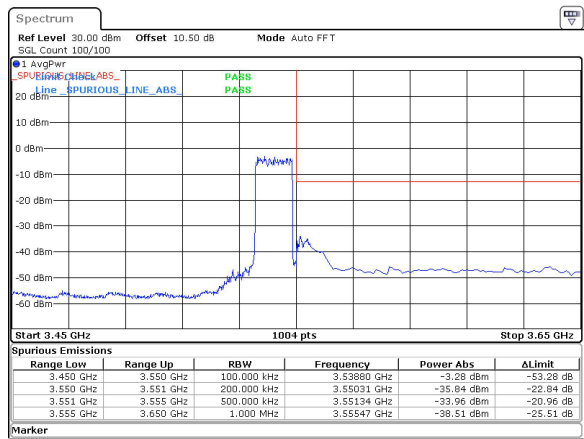
15MHz_30kHz_3542.5MHz_DFT-s-OFDM QPSK_RB36@0&-33.96 dBm
