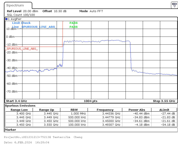
60MHz_30kHz_3480MHz_DFT-s-OFDM QPSK_RB162@0&-34.61 dBm
