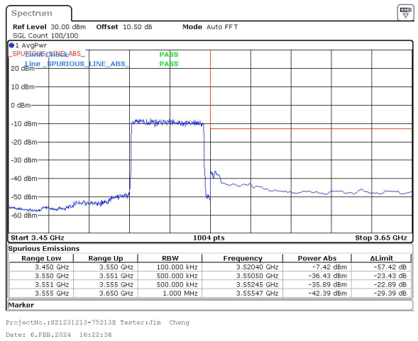
40MHz_30kHz_3530MHz_DFT-s-OFDM QPSK_RB100@0&-35.89 dBm
