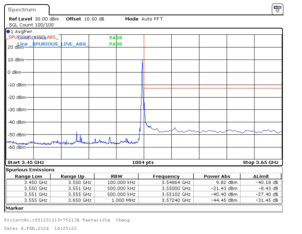
50MHz_30kHz_3525MHz_DFT-s-OFDM QPSK_RB1@132&-21.43 dBm
