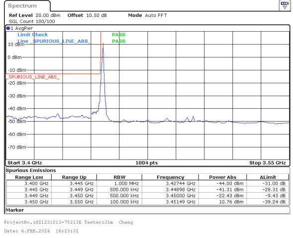
50MHz_30kHz_3475MHz_DFT-s-OFDM QPSK_RB1@0&-22.43 dBm
