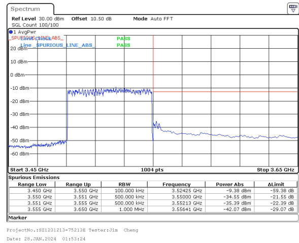
60MHz_30kHz_3520MHz_DFT-s-OFDM QPSK_RB162@0&-34.55 dBm
