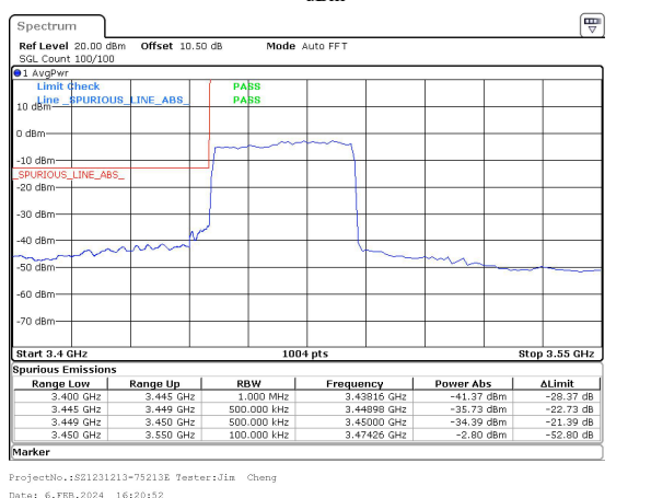
40MHz_30kHz_3470MHz_DFT-s-OFDM QPSK_RB100@0&-34.39 dBm
