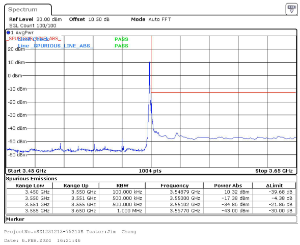
40MHz_30kHz_3530MHz_DFT-s-OFDM QPSK_RB1@105&-17.38 dBm
