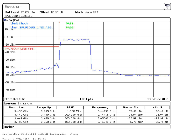
30MHz_30kHz_3465MHz_DFT-s-OFDM QPSK_RB75@0&-34.94 dBm
