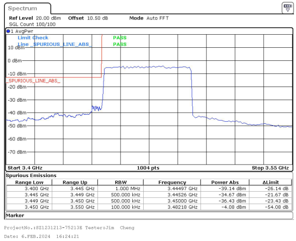
50MHz_30kHz_3475MHz_DFT-s-OFDM QPSK_RB128@0&-34.67 dBm
