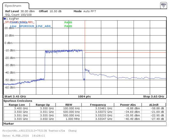
50MHz_30kHz_3525MHz_DFT-s-OFDM QPSK_RB128@0&-34.69 dBm
