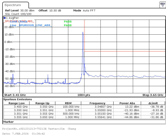
90MHz_30kHz_3505MHz_DFT-s-OFDM QPSK_RB1@244&-21.93 dBm
