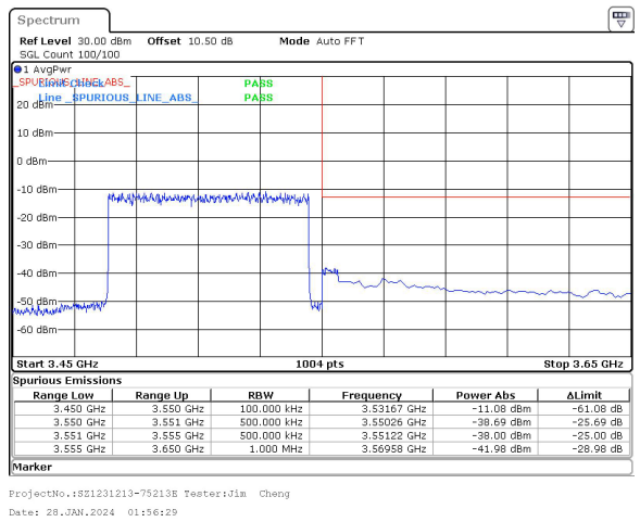
70MHz_30kHz_3515MHz_DFT-s-OFDM QPSK_RB180@0&-38.00 dBm
