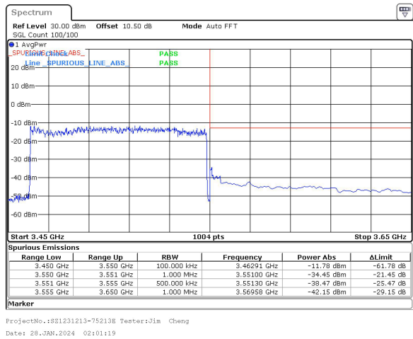
90MHz_30kHz_3505MHz_DFT-s-OFDM QPSK_RB243@0&-34.45 dBm
