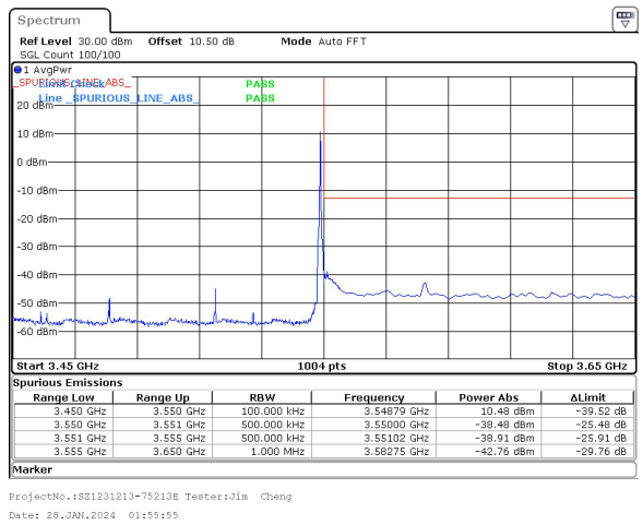
70MHz_30kHz_3515MHz_DFT-s-OFDM QPSK_RB1@188&-38.48 dBm
