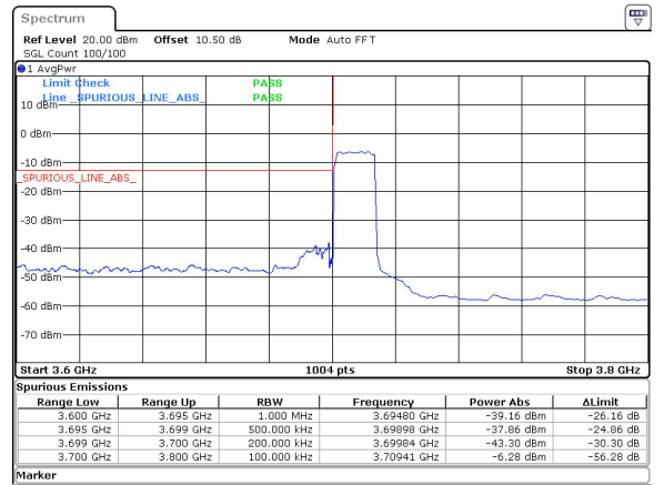
15MHz_30kHz_3707.5MHz_DFT-s-OFDM QPSK_RB36@0&-37.86 dBm
