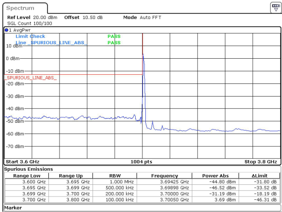
15MHz_30kHz_3707.5MHz_DFT-s-OFDM QPSK_RB1@0&-31.19 dBm
