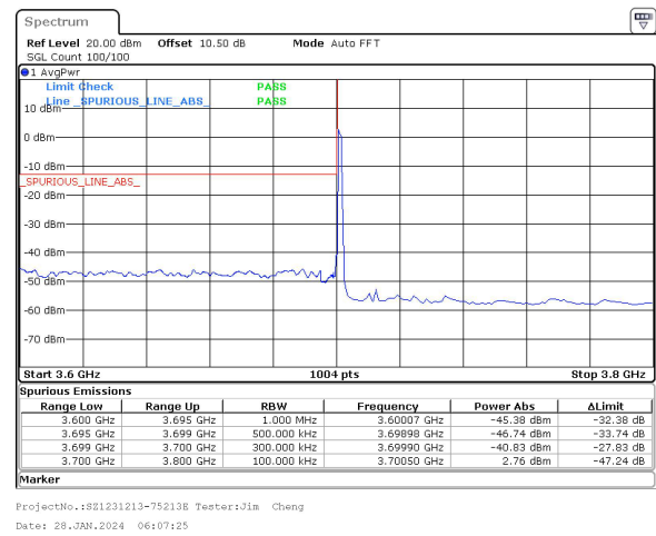
25MHz_30kHz_3712.5MHz_DFT-s-OFDM QPSK_RB1@0&-40.83 dBm
