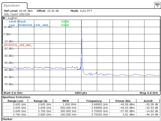
25MHz_15kHz_3712.5MHz_DFT-s-OFDM QPSK_RB1@0&-27.82 dBm
