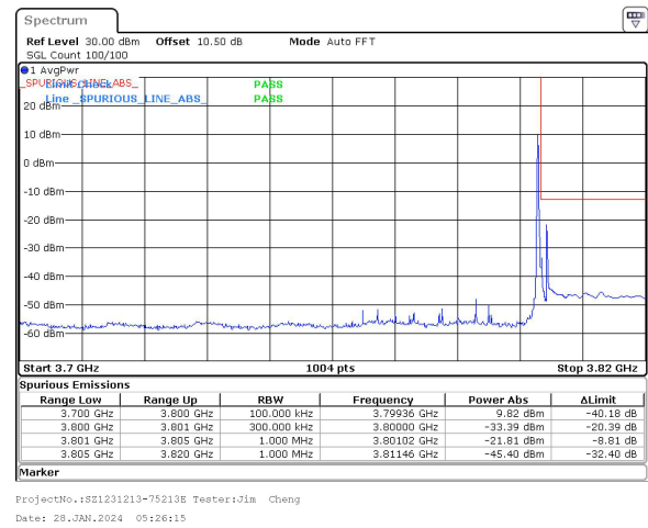
25MHz_15kHz_3787.5MHz_DFT-s-OFDM QPSK_RB1@132&-21.81 dBm
