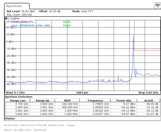
25MHz_30kHz_3787.5MHz_DFT-s-OFDM QPSK_RB1@64&-39.13 dBm
