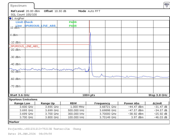
30MHz_30kHz_3715MHz_DFT-s-OFDM QPSK_RB1@0&-38.92 dBm
