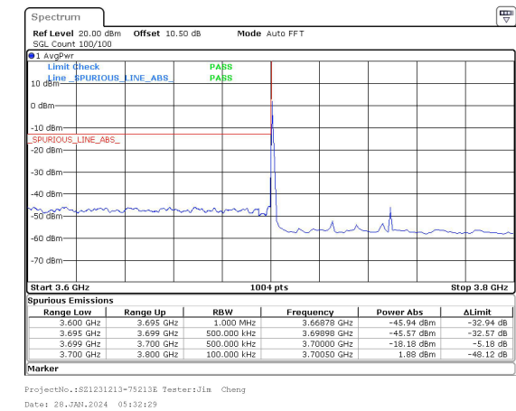
50MHz_15kHz_3725MHz_DFT-s-OFDM QPSK_RB1@0&-18.18 dBm
