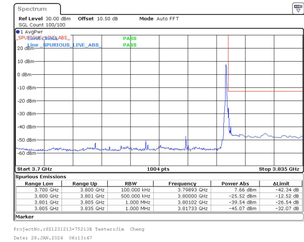
40MHz_30kHz_3780MHz_DFT-s-OFDM QPSK_RB1@105&-25.52 dBm
