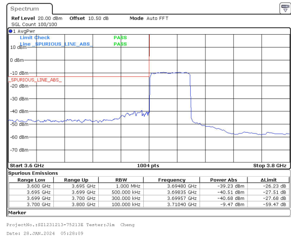
30MHz_15kHz_3715MHz_DFT-s-OFDM QPSK_RB160@0&-39.23 dBm
