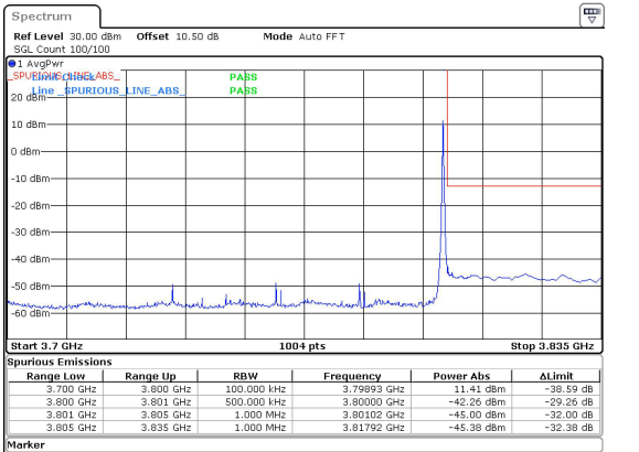
40MHz_15kHz_3780MHz_DFT-s-OFDM QPSK_RB1@215&-42.26 dBm
