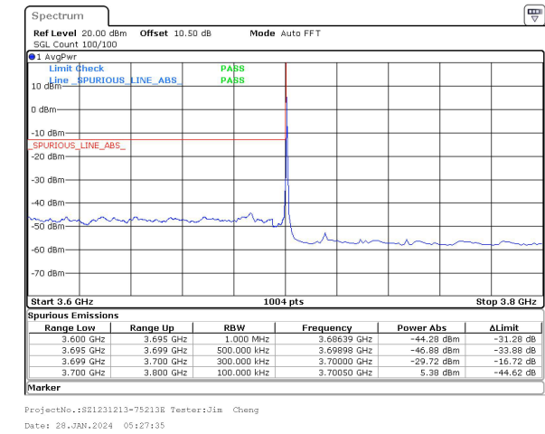
30MHz_15kHz_3715MHz_DFT-s-OFDM QPSK_RB1@0&-29.72 dBm
