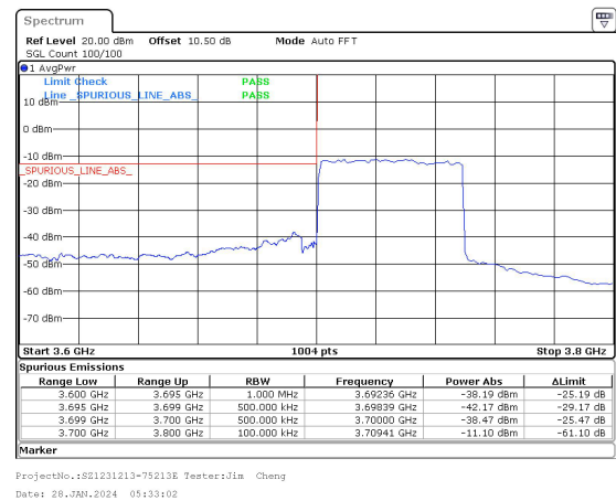
50MHz_15kHz_3725MHz_DFT-s-OFDM QPSK_RB270@0&-38.19 dBm
