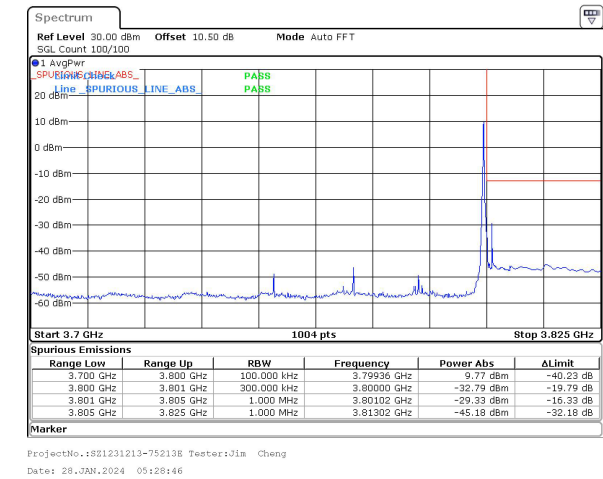
30MHz_15kHz_3785MHz_DFT-s-OFDM QPSK_RB1@159&-29.33 dBm
