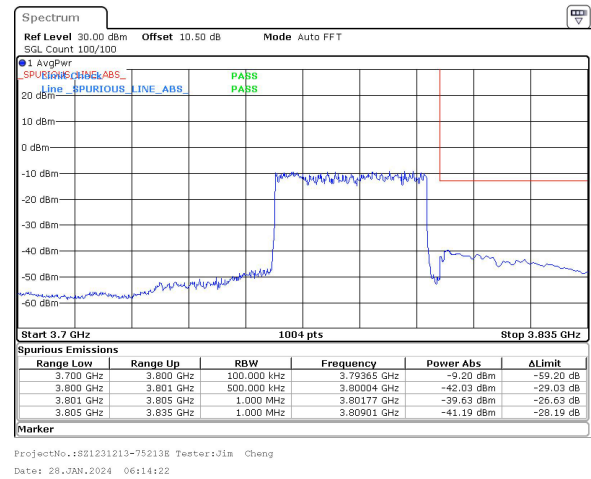
40MHz_30kHz_3780MHz_DFT-s-OFDM QPSK_RB100@0&-39.63 dBm
