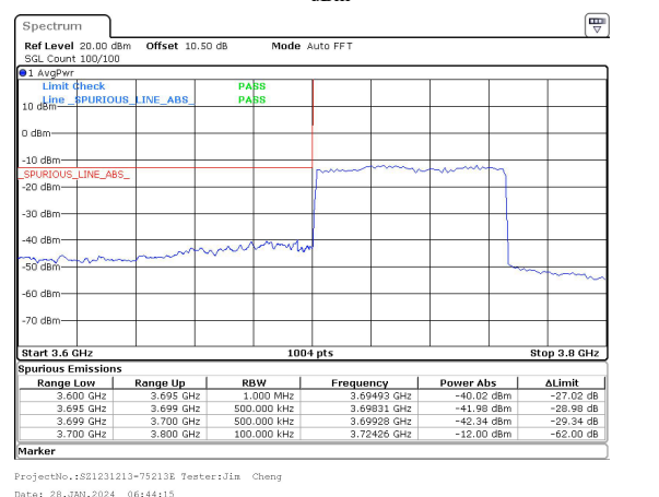
70MHz_30kHz_3735MHz_DFT-s-OFDM QPSK_RB180@0&-40.02 dBm
