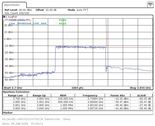
50MHz_15kHz_3775MHz_DFT-s-OFDM QPSK_RB270@0&-39.47 dBm
