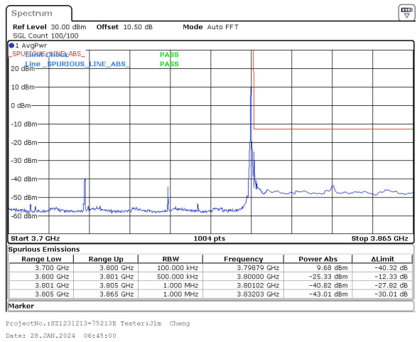
70MHz_30kHz_3765MHz_DFT-s-OFDM QPSK_RB1@188&-25.33 dBm
