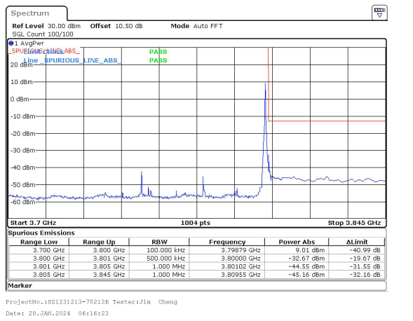
50MHz_30kHz_3775MHz_DFT-s-OFDM QPSK_RB1@132&-32.67 dBm
