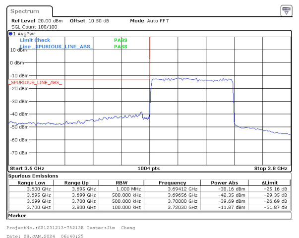
60MHz_30kHz_3730MHz_DFT-s-OFDM QPSK_RB162@0&-38.16 dBm
