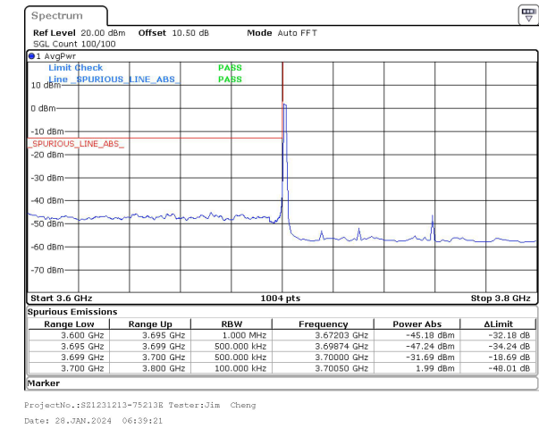
60MHz_30kHz_3730MHz_DFT-s-OFDM QPSK_RB1@0&-31.69 dBm
