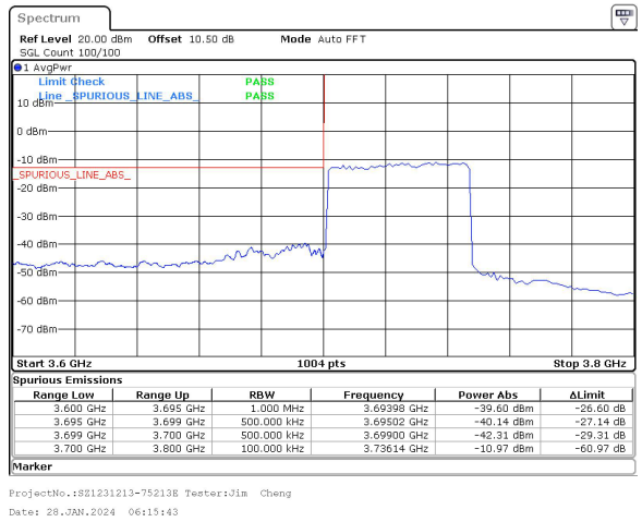
50MHz_30kHz_3725MHz_DFT-s-OFDM QPSK_RB128@0&-39.60 dBm
