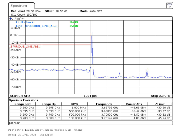
70MHz_30kHz_3735MHz_DFT-s-OFDM QPSK_RB1@0&-43.52 dBm
