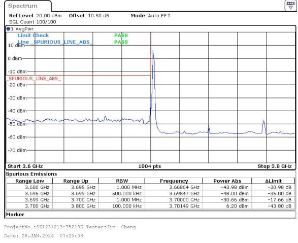
80MHz_30kHz_3740MHz_DFT-s-OFDM QPSK_RB1@0&-30.66 dBm
