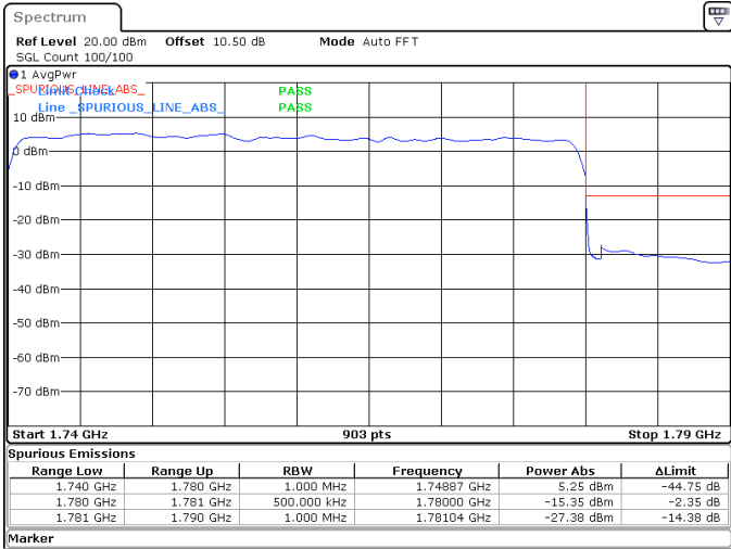
40MHz_15kHz_1760MHz_DFT-s-OFDM QPSK_RB216@0 -15.35 dBm
