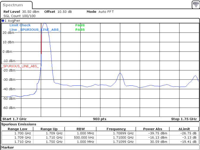
40MHz_15kHz_1730MHz_DFT-s-OFDM QPSK_RB1@0 -16.13 dBm
