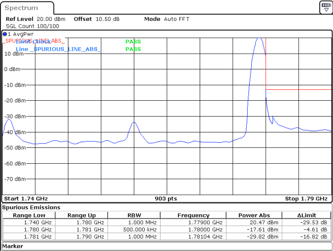
40MHz_15kHz_1760MHz_DFT-s-OFDM QPSK_RB1@215 -17.61 dBm
