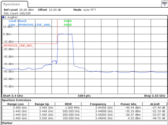
15MHz_15kHz_3457.5MHz_DFT-s-OFDM QPSK_RB75@0 -35.19 dBm
