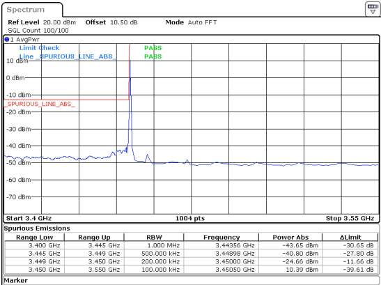
15MHz_15kHz_3457.5MHz_DFT-s-OFDM QPSK_RB1@0 -24.66 dBm
