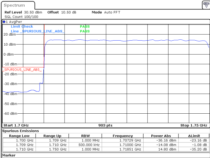
40MHz_15kHz_1730MHz_DFT-s-OFDM QPSK_RB216@0 -14.08 dBm
