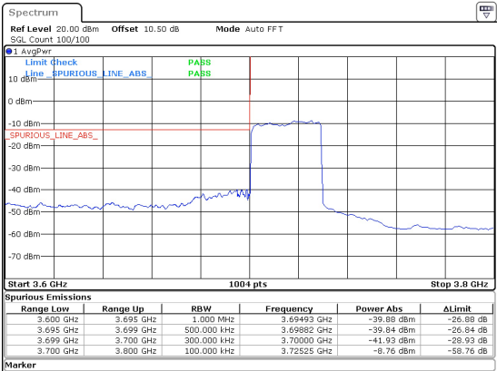
30MHz_15kHz_3715MHz_DFT-s-OFDM QPSK_RB160@0 -39.84 dBm
