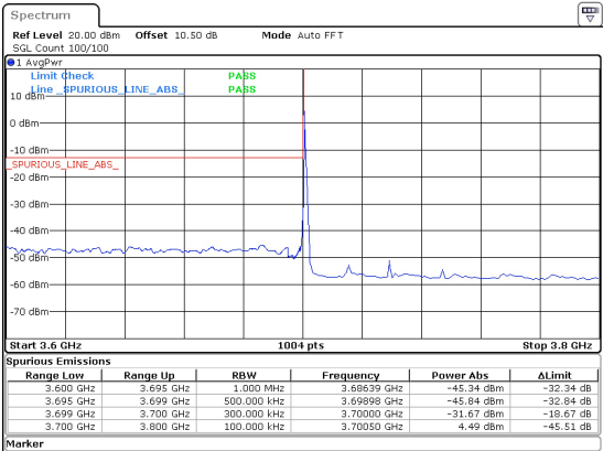
30MHz_15kHz_3715MHz_DFT-s-OFDM QPSK_RB1@0 -31.67 dBm
