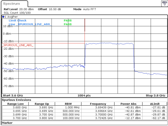
60MHz_30kHz_3730MHz_DFT-s-OFDM QPSK_RB162@0 -40.81 dBm
