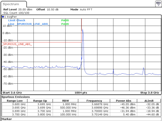
80MHz_30kHz_3740MHz_DFT-s-OFDM QPSK_RB1@0 -31.94 dBm
