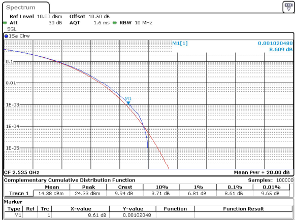
10MHz_15kHz_2535MHz_CP-OFDM 256 QAM_RB52@0 8.61 dB
