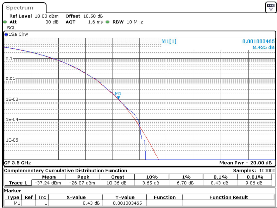
10MHz_15kHz_3500MHz_DFT-s-OFDM 256 QAM_RB50@0 8.43 dB
