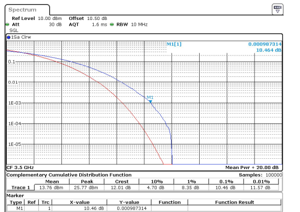
10MHz_30kHz_3500MHz_CP-OFDM 256 QAM_RB24@0 10.46 dB
