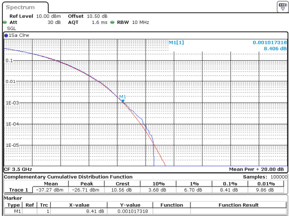
10MHz_15kHz_3500MHz_CP-OFDM 256 QAM_RB52@0 8.41 dB
