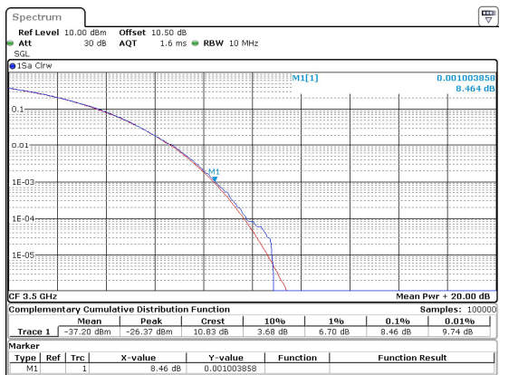
10MHz_30kHz_3500MHz_CP-OFDM 64 QAM_RB24@0 8.46 dB
