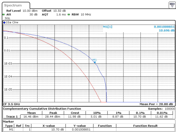
10MHz_30kHz_3500MHz_CP-OFDM 16 QAM_RB24@0 10.70 dB
