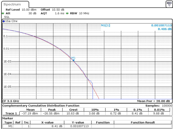
10MHz_15kHz_3500MHz_CP-OFDM 16 QAM_RB52@0 8.41 dB
