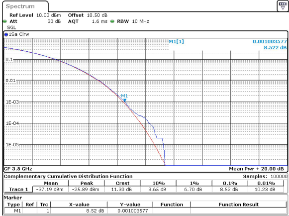
10MHz_15kHz_3500MHz_CP-OFDM 64 QAM_RB52@0 8.52 dB
