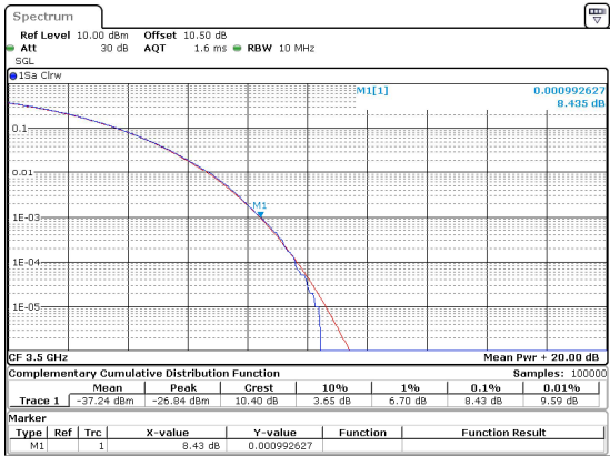
10MHz_15kHz_3500MHz_DFT-s-OFDM 16 QAM_RB50@0 8.43 dB
