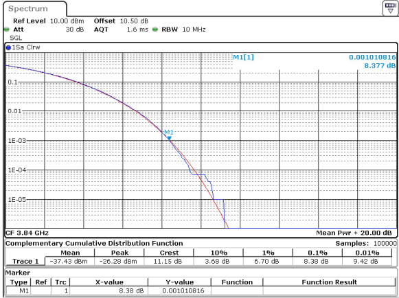
10MHz_15kHz_3840MHz_CP-OFDM QPSK_RB52@0 8.38 dB
