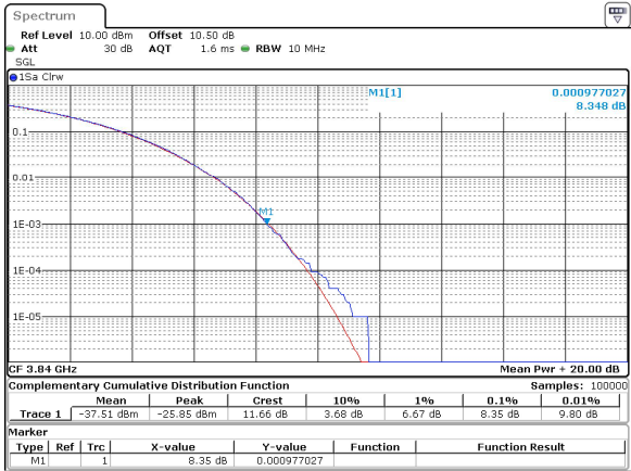
10MHz_15kHz_3840MHz_CP-OFDM 16 QAM_RB52@0 8.35 dB
