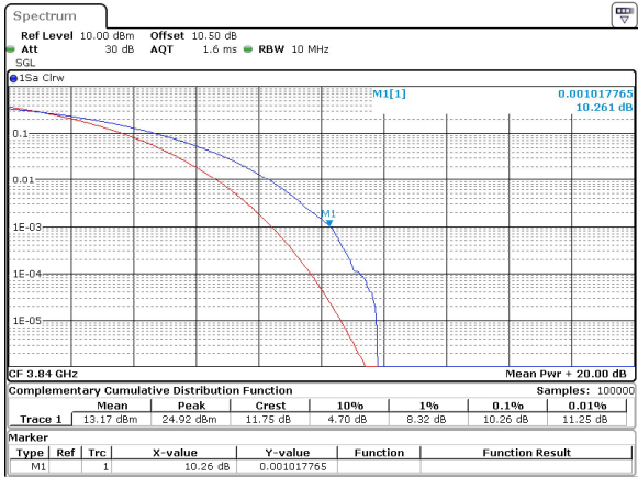
10MHz_15kHz_3840MHz_CP-OFDM 256 QAM_RB52@0 10.26 dB
