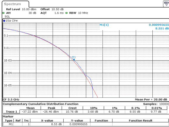
10MHz_30kHz_3500MHz_DFT-s-OFDM 16 QAM_RB24@0 8.55 dB
