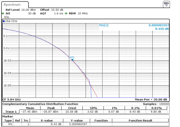
10MHz_15kHz_3840MHz_DFT-s-OFDM 16 QAM_RB50@0 8.43 dB
