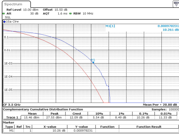
10MHz_30kHz_3500MHz_DFT-s-OFDM 64 QAM_RB24@0 10.26 dB
