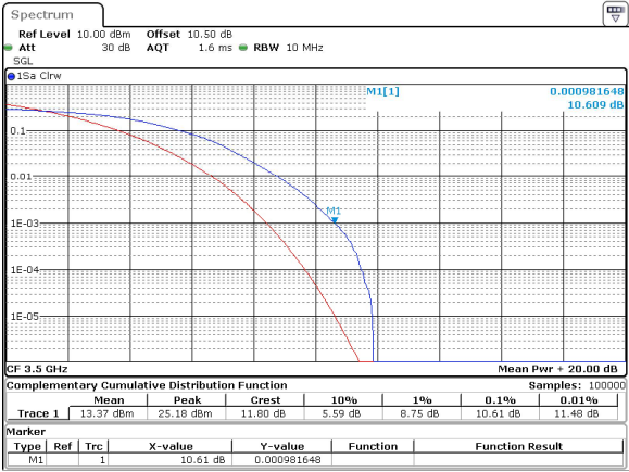
10MHz_30kHz_3500MHz_DFT-s-OFDM 256 QAM_RB24@0 10.61 dB
