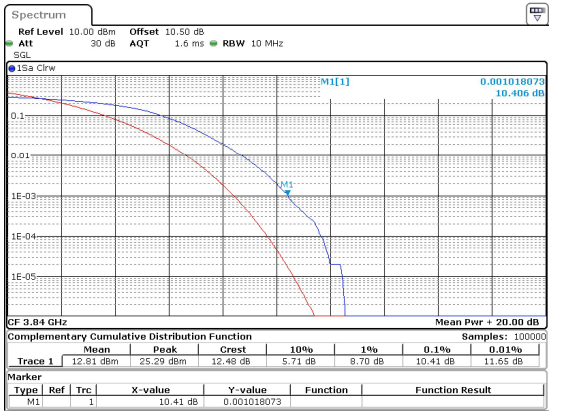
10MHz_15kHz_3840MHz_DFT-s-OFDM 256 QAM_RB50@0 10.41 dB
