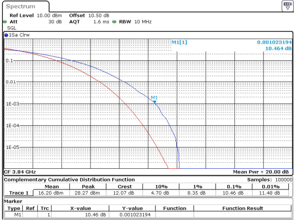
10MHz_15kHz_3840MHz_CP-OFDM 64 QAM_RB52@0 10.46 dB
