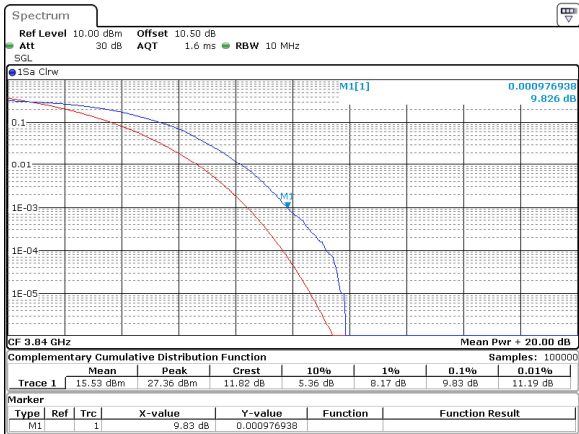
10MHz_30kHz_3840MHz_DFT-s-OFDM 64 QAM_RB24@0 9.83 dB
