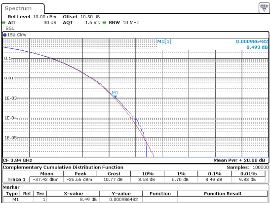
10MHz_30kHz_3840MHz_CP-OFDM 256 QAM_RB24@0 8.49 dB
