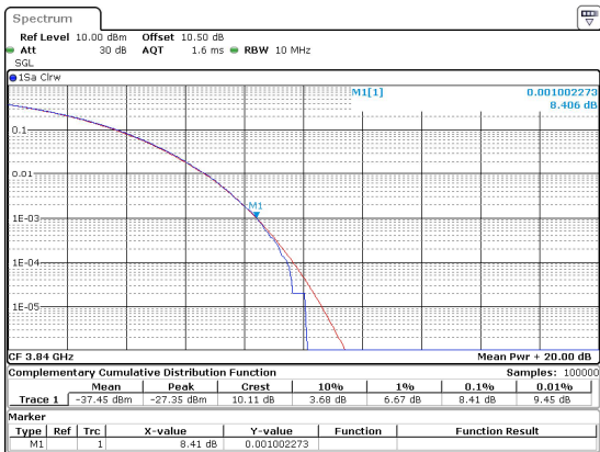
10MHz_30kHz_3840MHz_CP-OFDM 64 QAM_RB24@0 8.41 dB
