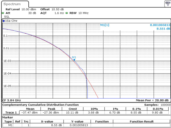
10MHz_30kHz_3840MHz_DFT-s-OFDM 16 QAM_RB24@0 8.55 dB
