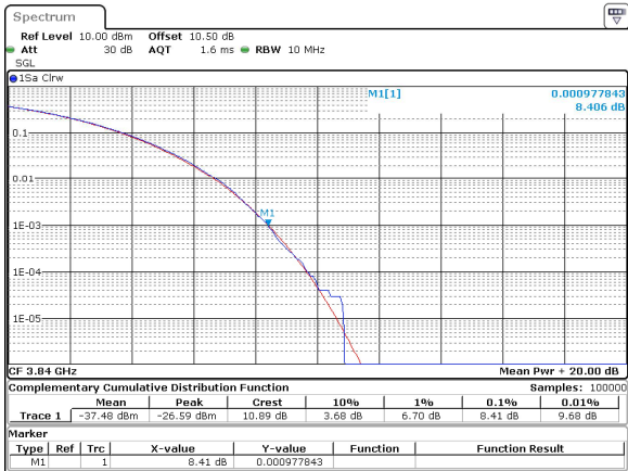
10MHz_30kHz_3840MHz_CP-OFDM 16 QAM_RB24@0 8.41 dB
