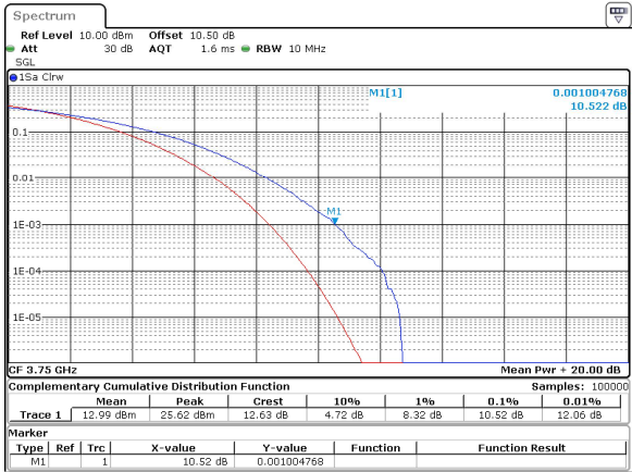
10MHz_15kHz_3750MHz_CP-OFDM 256 QAM_RB52@0 10.52 dB
