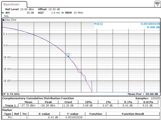
10MHz_15kHz_3750MHz_DFT-s-OFDM 16 QAM_RB50@0 8.41 dB
