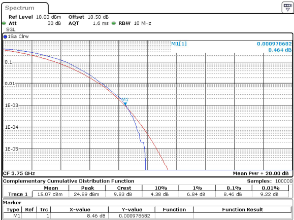
10MHz_30kHz_3750MHz_DFT-s-OFDM 256 QAM_RB24@0 8.46 dB
