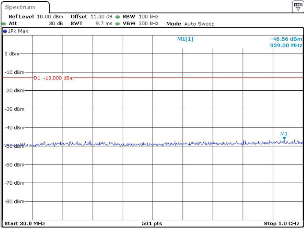
Band 2_1.4 MHz_Low_QPSK_RB6#0_1(30MHz-1GHz)
