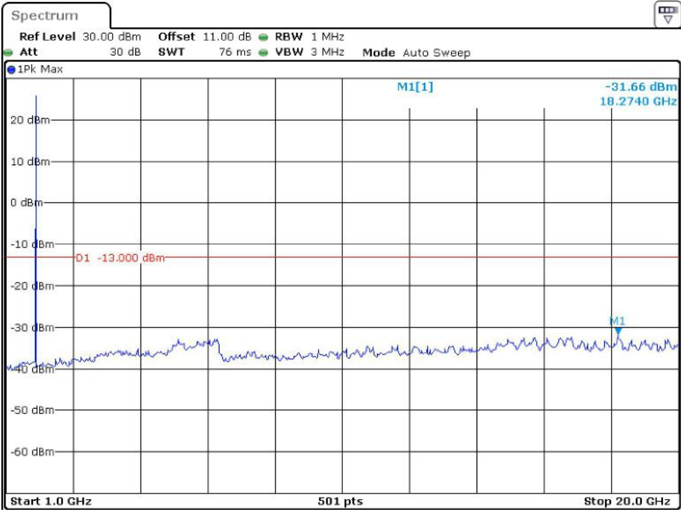
Band 2_1.4 MHz_Low_QPSK_RB6#0_2(1GHz-20GHz)
